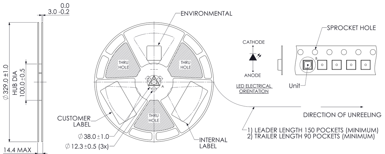
Figure 14. Reel dimensions for LUXEON Versat 2020 PCA 150
