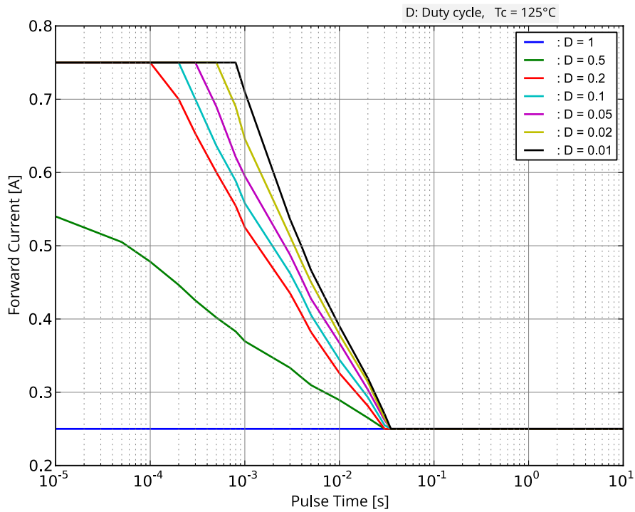
Figure 10. Permissible pulse handling capability for LUXEON Versat 2020 PCA 150
