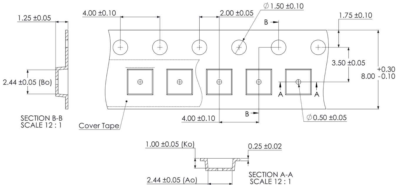
Figure 13. Pocket tape dimensions for LUXEON Versat 2020 PCA 150
