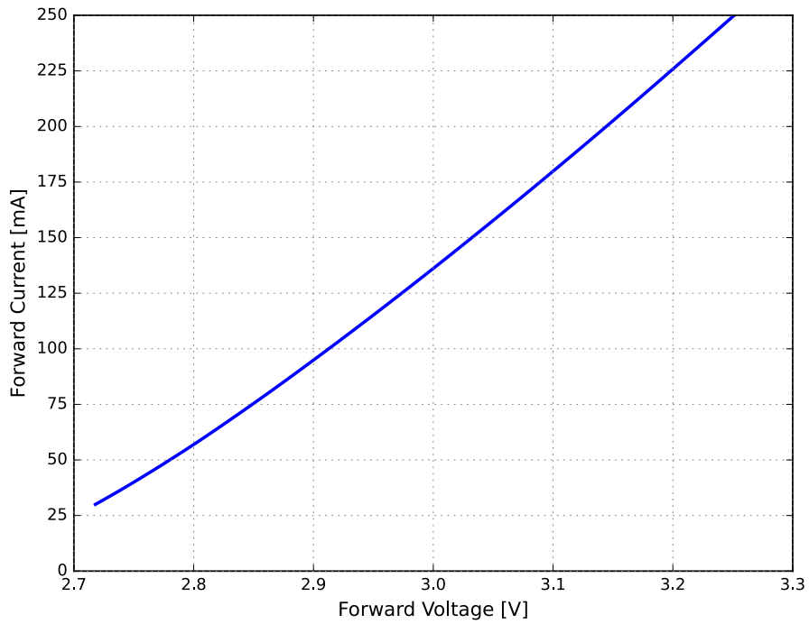
Figure 4. Typical forward current vs. forward voltage for LUXEON Versat 2020 PCA 150 at T_c = 25\text{ }^\circ\text{C}
