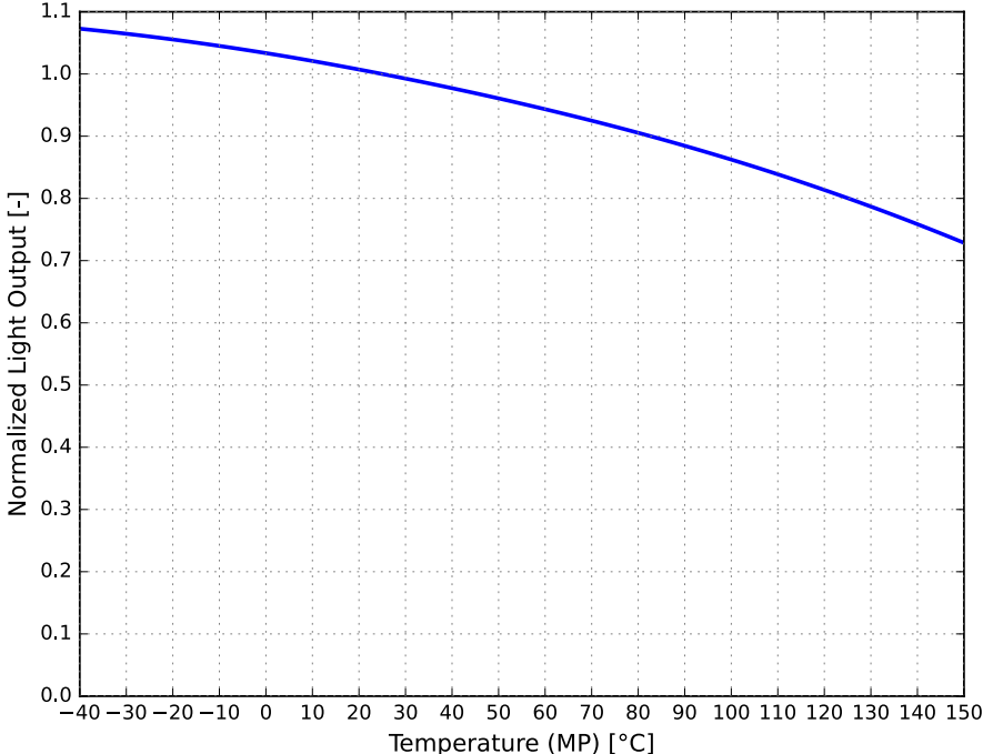
Figure 2. Typical normalized light output vs. case temperature for LUXEON Versat 2020 PCA 150 at 20 ms MP, 150 mA
