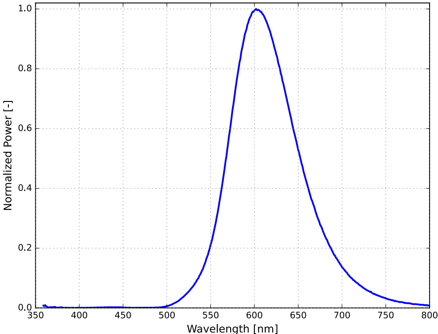
Figure 1. Typical normalized power vs. wavelength for LUXEON Versat 2020 PCA 150 at 20 ms MP, 150 mA, T_c = 25\text{ }^\circ\text{C}
