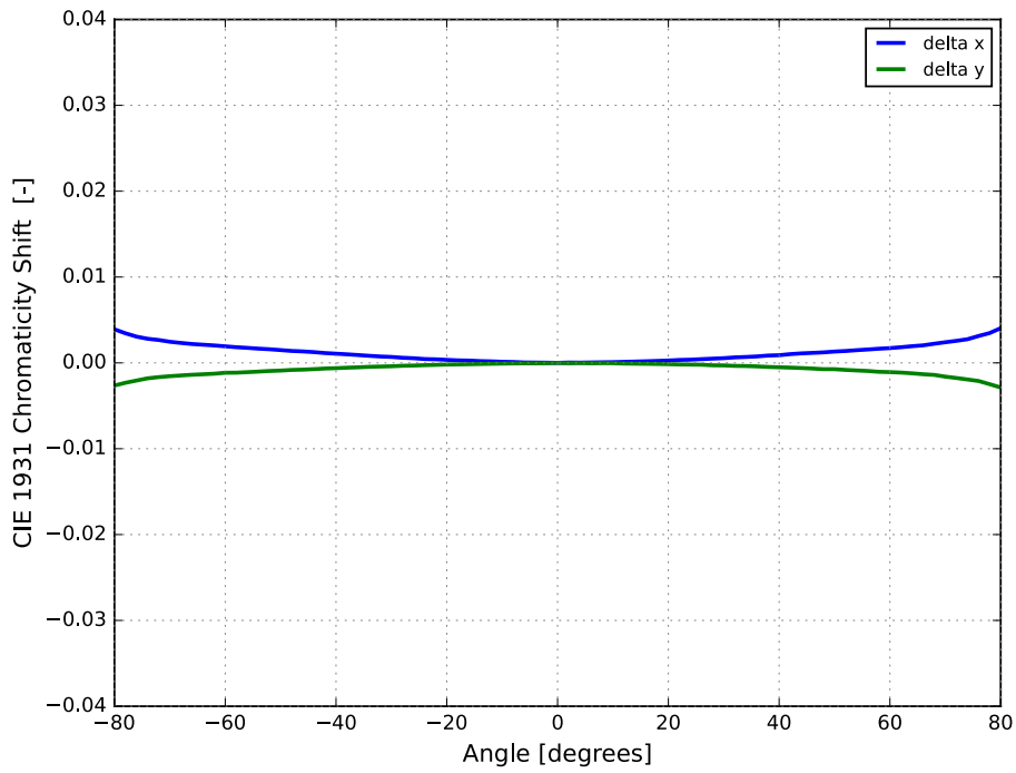
Figure 7. Typical color shift in CIE 1931 x and y coordinates over angle for LUXEON Versat 2020 PCA 150 at 20 ms MP, 150 mA
