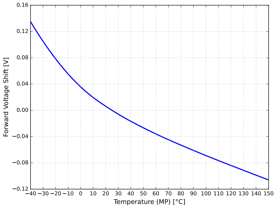
Figure 5. Typical forward voltage shift vs. case temperature for LUXEON Versat 2020 PCA 150
