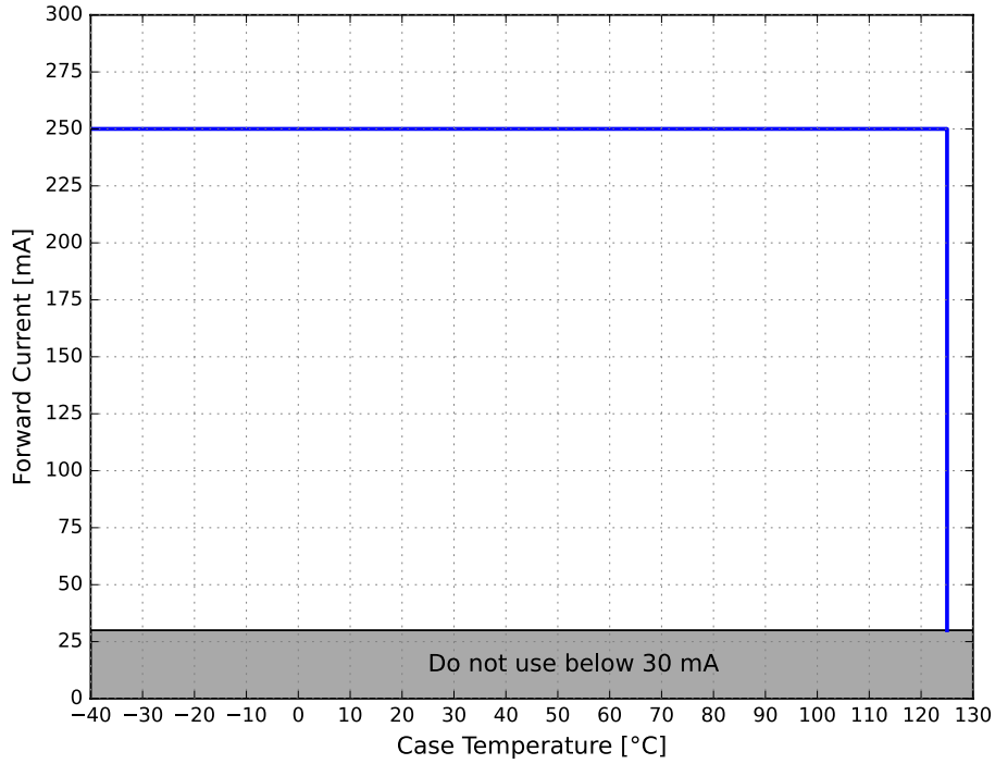
Figure 9. Maximum forward current vs. case temperature for LUXEON Versat 2020 PCA 150
