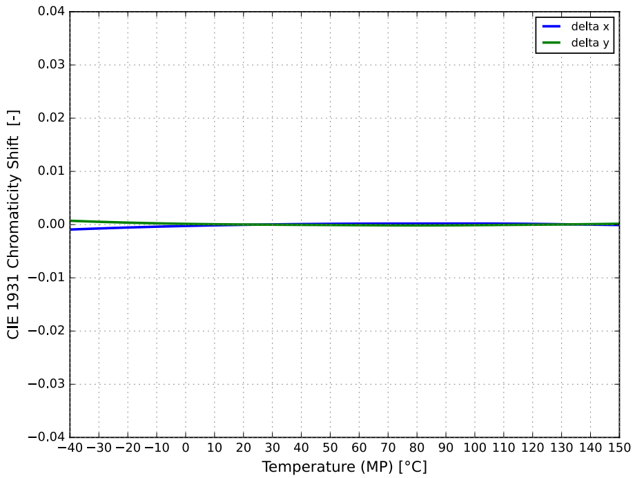
Figure 6. Typical color shift in CIE 1931 x and y coordinates for LUXEON Versat 2020 PCA 150 at 20 ms MP, 150 mA
