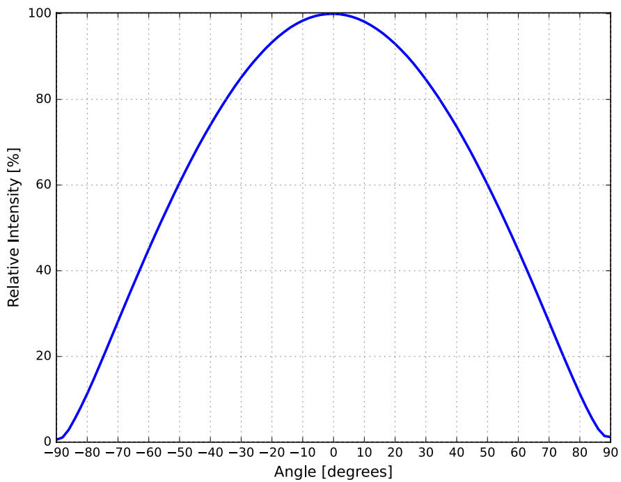
Figure 8. Typical radiation pattern for LUXEON Versat 2020 PCA 150 at 20 ms MP, 150 mA, T_c = 25\text{ }^\circ\text{C}
