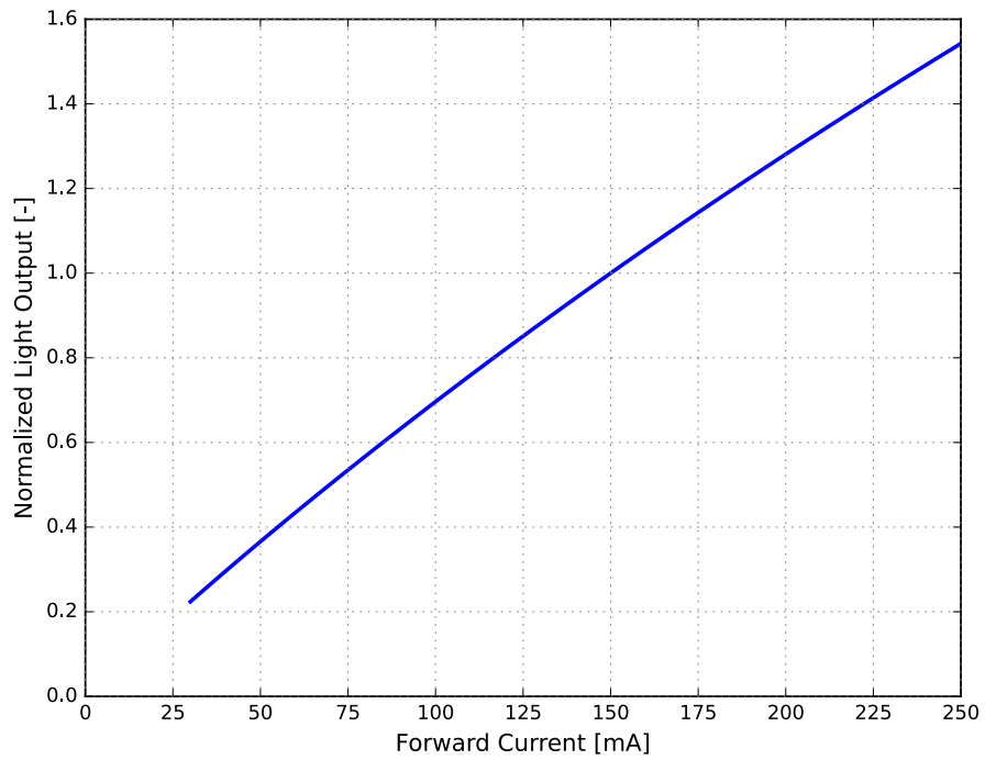
Figure 3. Typical normalized light output vs. forward current for LUXEON Versat 2020 PCA 150 at T_c = 25\text{ }^\circ\text{C}
