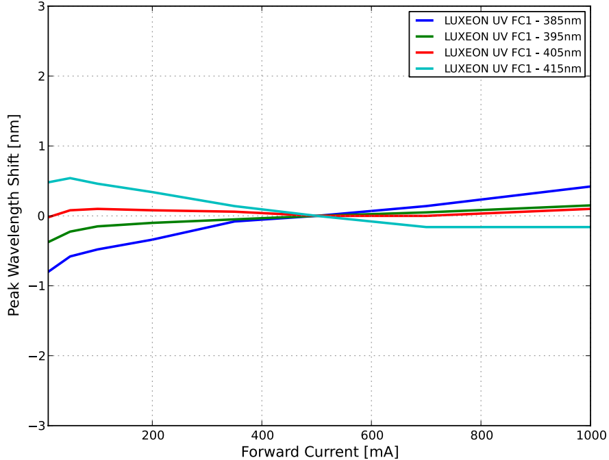
Figure 6. Typical peak wavelength shift vs. forward current for LUXEON UV FC Line at T_j=25^\circ\text{C} .
