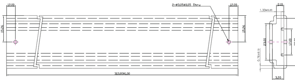
Figure 9d. Tube dimensions for L2C5-xxxx1211x19Px.
