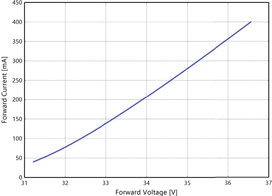
Figure 4a. Typical forward current vs. forward voltage for L2C5-xxxx1202H06Px at T_j=85^\circ\text{C} .
