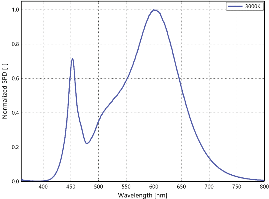
Figure 1a. Typical normalized power vs. wavelength for L2C5-xx80xxxHxxPx at specified test current, T_j=85^{\circ}\text{C} .
