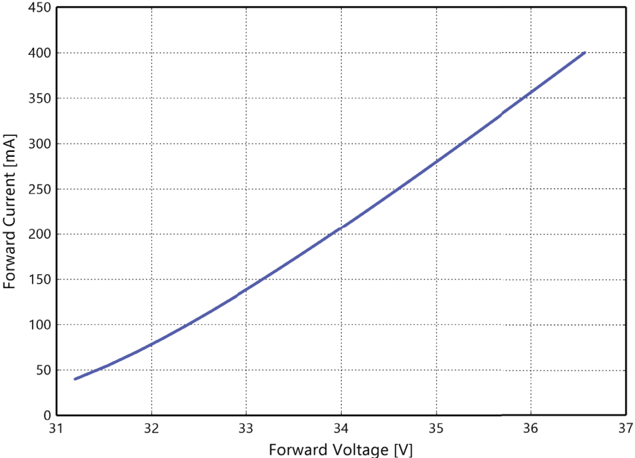
Figure 4b. Typical forward current vs. forward voltage for L2C5-xxxx1202H09Px at T_j=85^\circ\text{C} .
