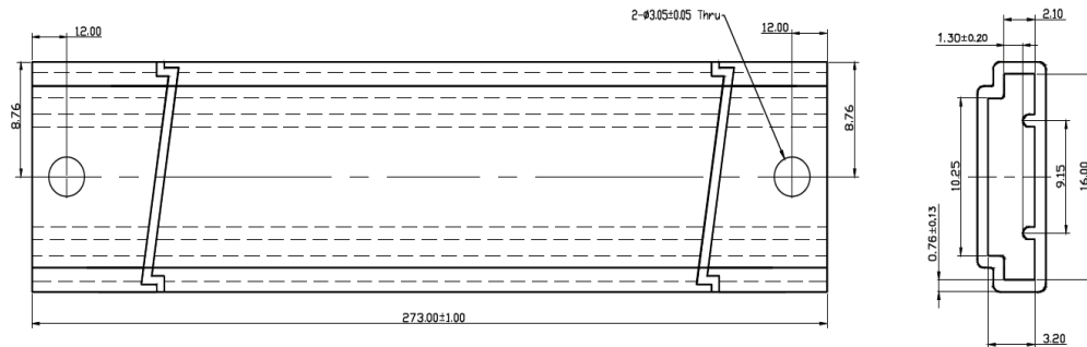
Figure 9a. Tube dimensions for L2C5-xxxx1202x06Px.
