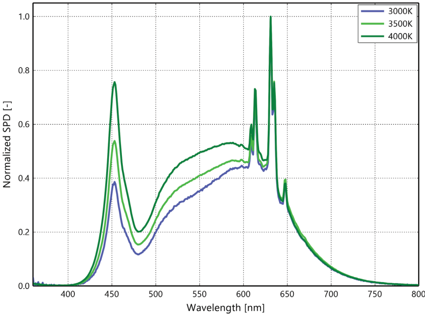
Figure 1b. Typical normalized power vs. wavelength for L2C5-xx90xxxHxxPx at specified test current, T_j=85^{\circ}\text{C} .
