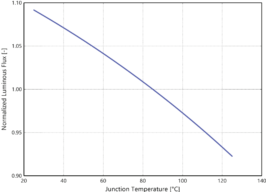
Figure 2. Typical normalized light output vs. junction temperature for L2C5-xxxx12xxxxPx at specified test current.
