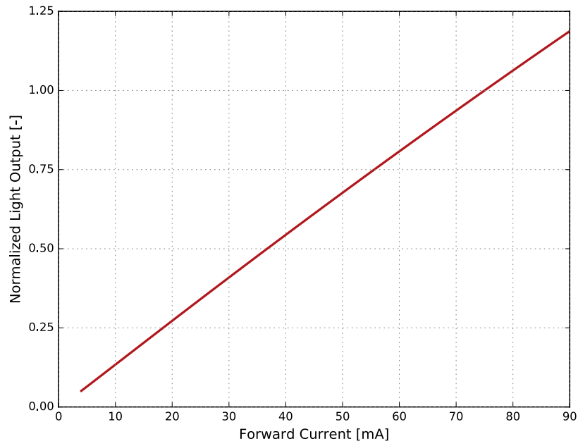
Figure 3. Typical normalized light output vs. forward current for SignalSure 75 at T_j = 25\text{ °C}
