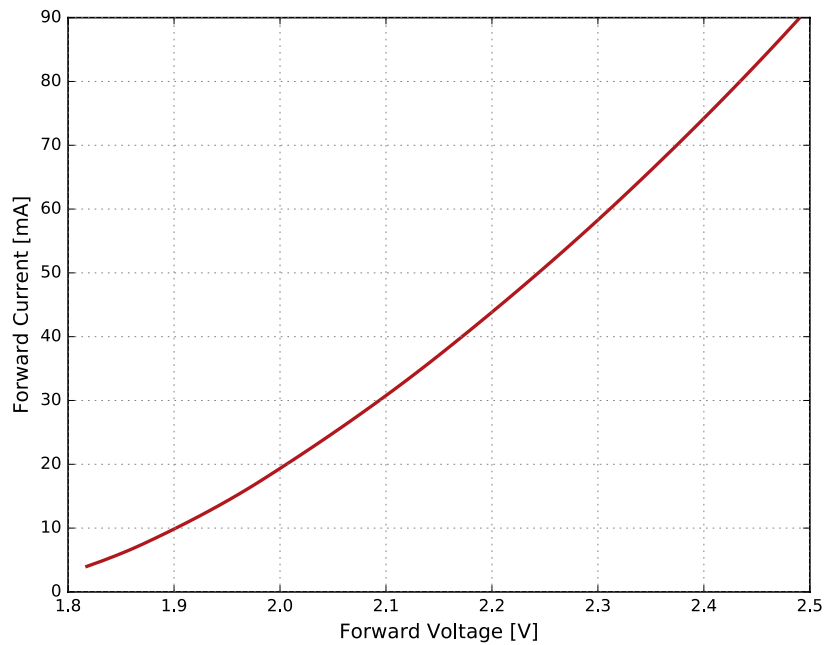
Figure 4a. Typical forward current vs. forward voltage for SignalSure 75 at T_j = 25\text{ °C}
