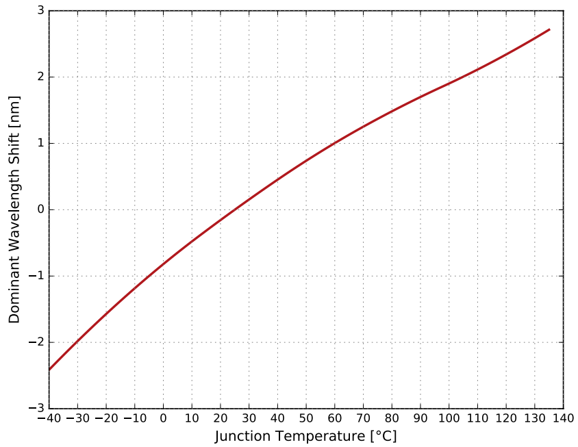
Figure 1b. Typical dominant wavelength shift vs junction temperature for SignalSure 75 at 20 ms MP, 75 mA, T_j = 25\text{ }^\circ\text{C}
