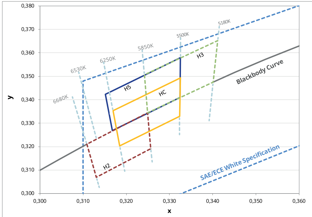
Figure 9. Color bin structure in CIE 1931 color space for LUXEON FX2 Cool White
