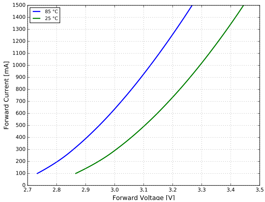
Figure 4a. Typical forward current vs. forward voltage for LUXEON FX2 Cool White at < 20 ms MP, T_c = 85\text{ °C} and 25\text{ °C}
