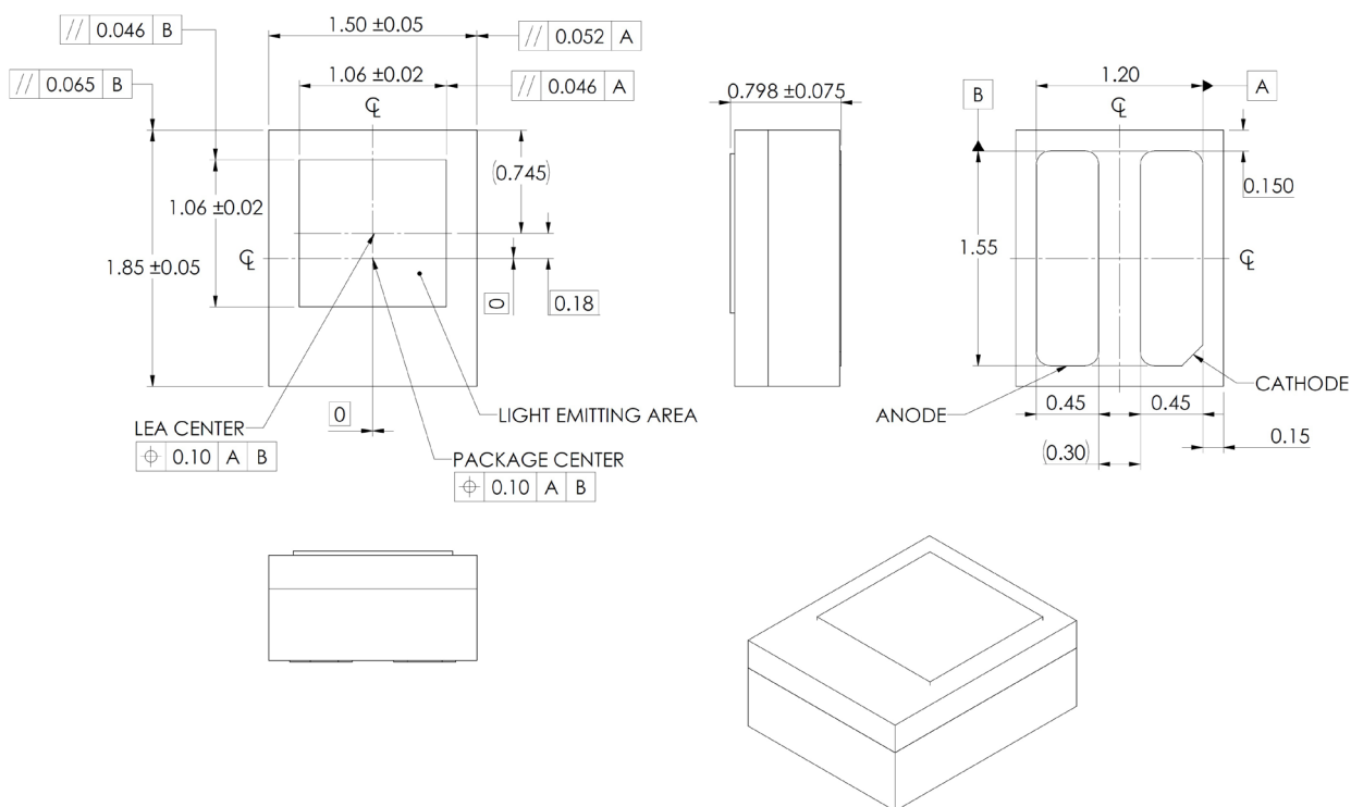
Figure 10. Mechanical dimensions for LUXEON FX2 Cool White
