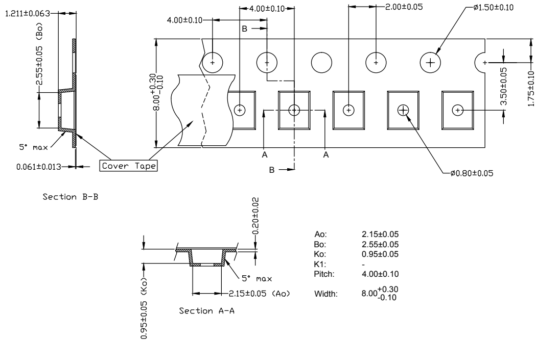
Figure 11. Pocket tape dimensions for LUXEON FX2 Cool White
