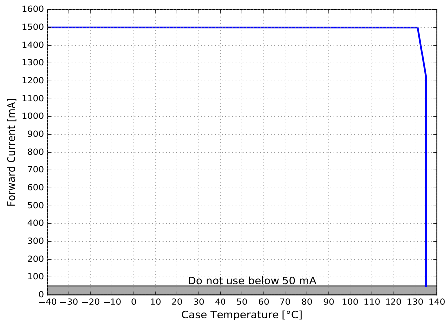
Figure 7. Maximum forward current vs. case temperature for LUXEON FX2 Cool White
