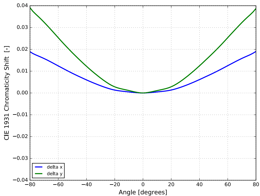
Figure 5c. Typical color shift in CIE 1931 x and y coordinates vs. angle for LUXEON FX2 Cool White at 1000 mA
