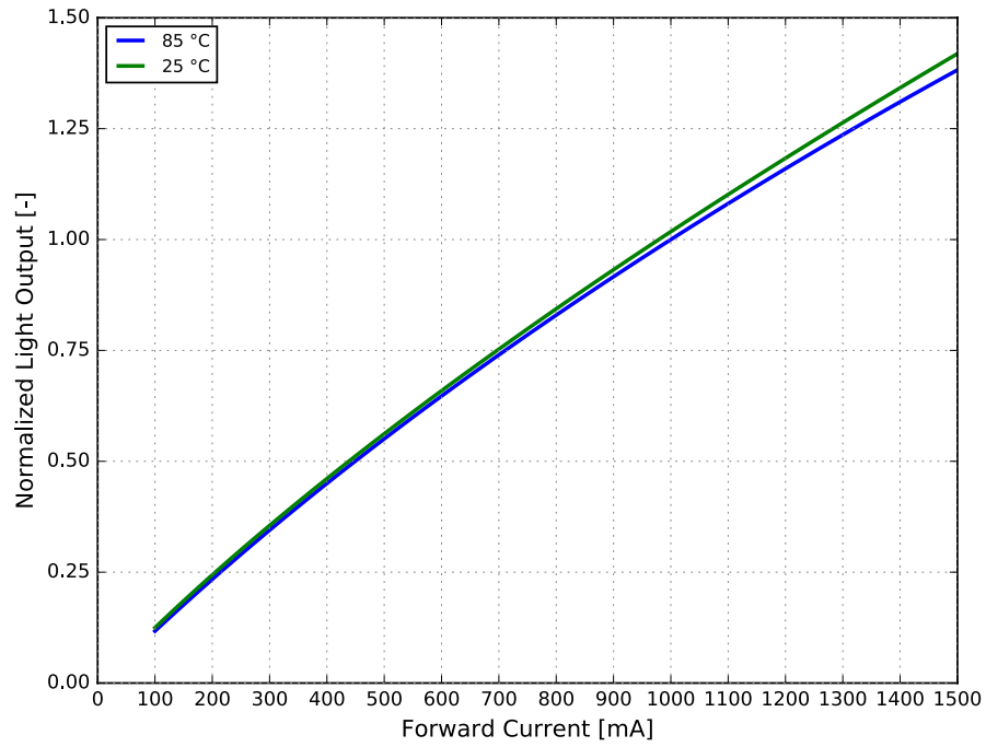
Figure 3b. Typical normalized light output vs. forward current for LUXEON FX2 Cool White at < 20 ms MP, 25°C and 85 °C
