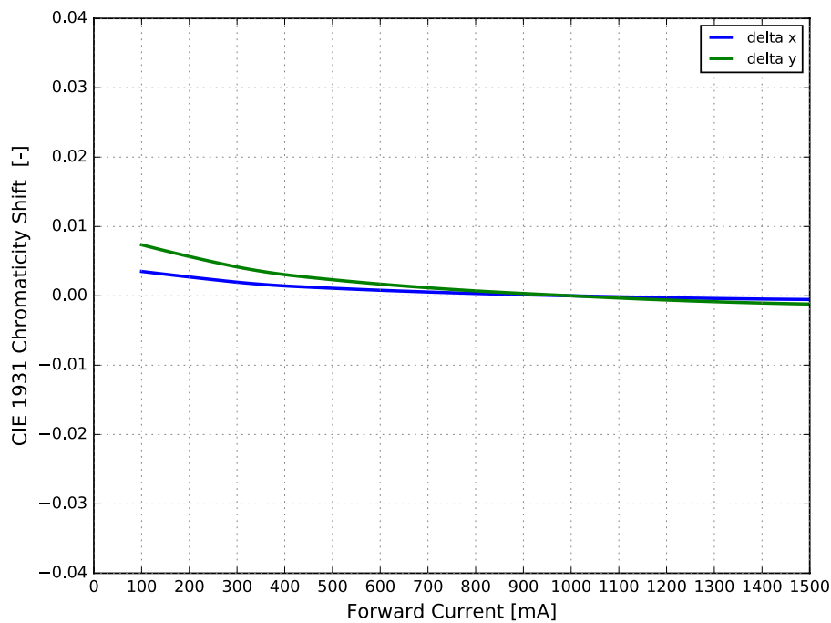
Figure 5b. Typical color shift in CIE 1931 x and y coordinates vs. forward current for LUXEON FX2 Cool White at < 20 ms MP, T_c = 85\text{ }^{\circ}\text{C}
