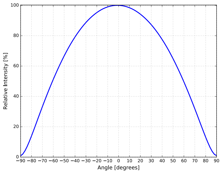
Figure 6. Typical radiation pattern for LUXEON FX2 Cool White at 1000 mA
