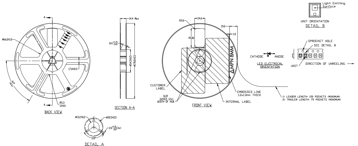
Figure 12. Reel dimensions for LUXEON FX2 Cool White
