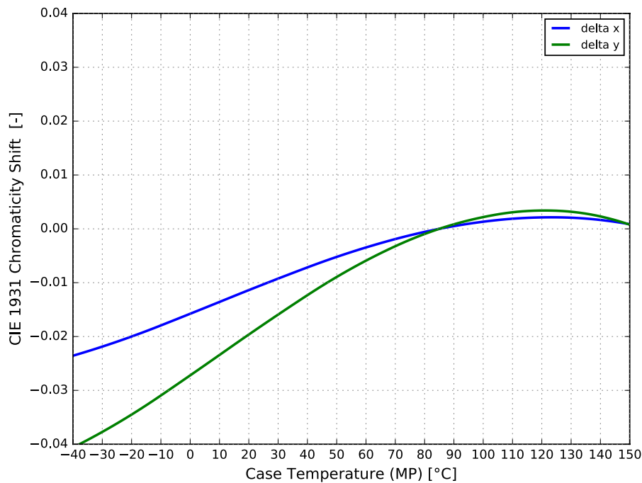
Figure 5a. Typical color shift in CIE 1931 x and y coordinates vs. case temperature for LUXEON FX2 Cool White at < 20 ms MP, 1000 mA
