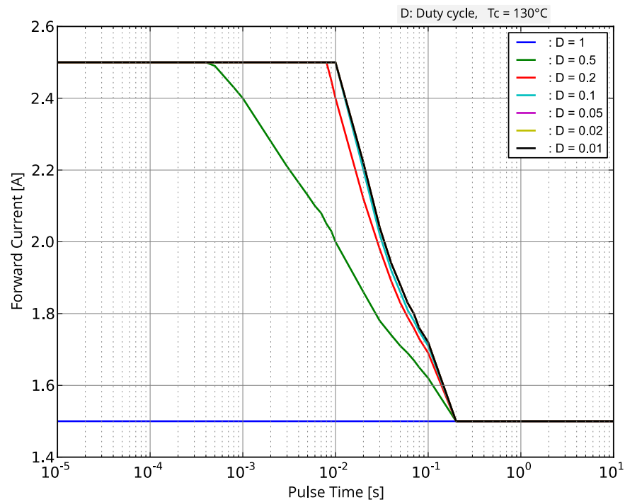
Figure 8. Permissible pulse handling capability for LUXEON FX2 Cool White
