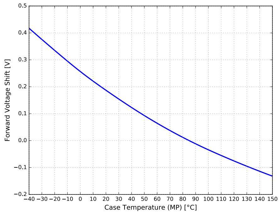
Figure 4b. Typical forward voltage shift vs. case temperature for LUXEON FX2 Plus Cool White at < 20 ms MP, 1000 mA.
