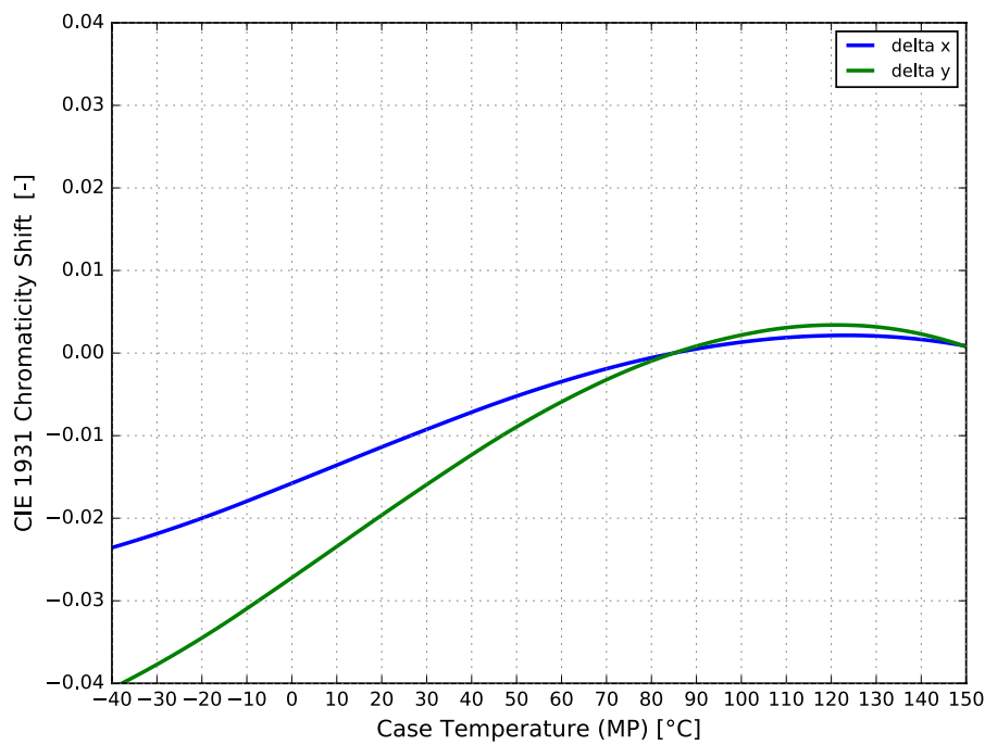
Figure 5a. Typical color shift in CIE 1931 x and y coordinates vs. case temperature for LUXEON FX2 Plus Cool White at < 20 ms MP, 1000 mA.
