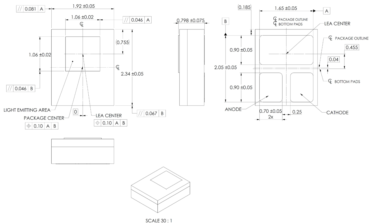
Figure 10. Mechanical dimensions for LUXEON FX2 Plus Cool White.
