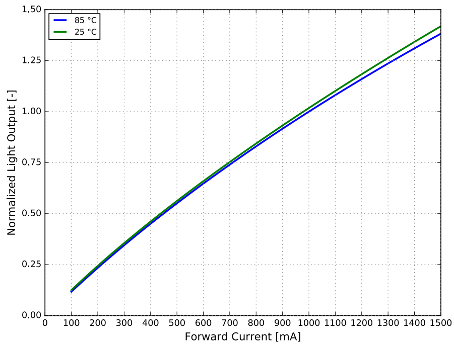
Figure 3b. Typical normalized light output vs. forward current for LUXEON FX2 Plus Cool White at < 20 ms MP, 25°C and 85°C.
