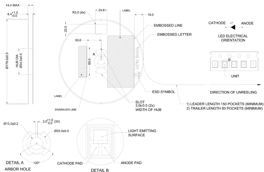
Figure 12. Reel dimensions for LUXEON FX2 Plus Cool White.
