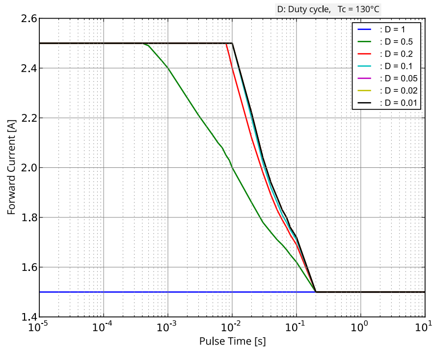
Figure 8. Permissible pulse handling capability for LUXEON FX2 Plus Cool White.
