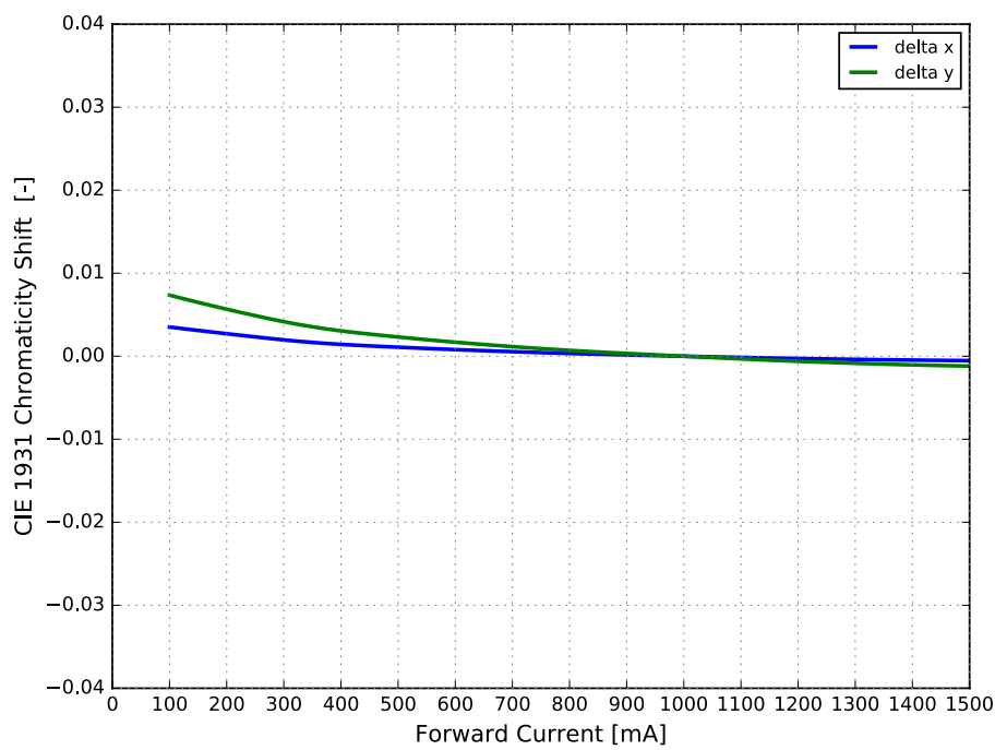
Figure 5b. Typical color shift in CIE 1931 x and y coordinates vs. forward current for LUXEON FX2 Plus Cool White at < 20 ms MP, T c = 85 °C.
