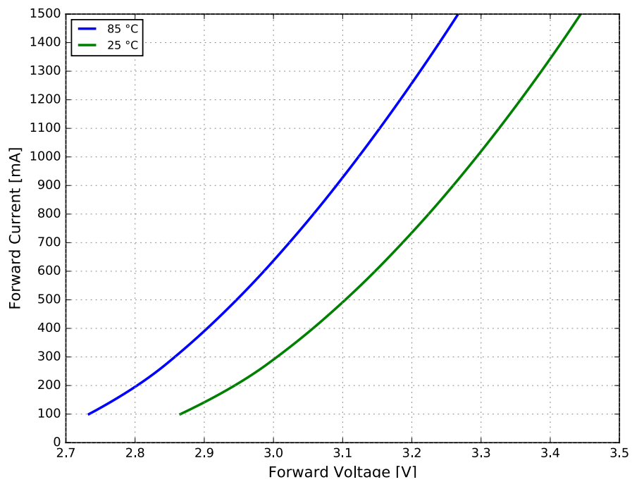
Figure 4a. Typical forward current vs. forward voltage for LUXEON FX2 Plus Cool White at < 20 ms MP, T_c = 85^\circ\text{C} and 25^\circ\text{C} .
