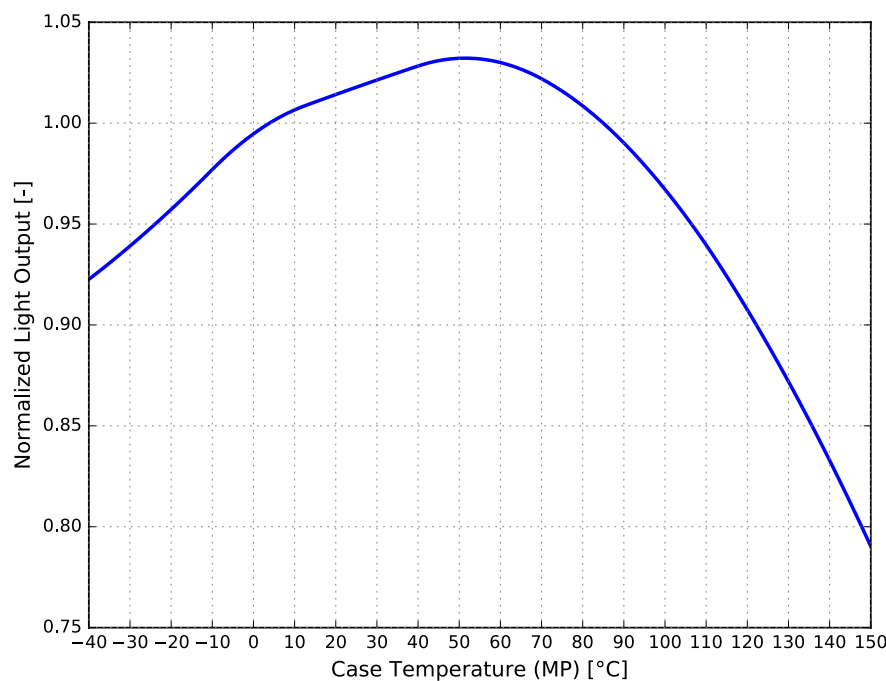
Figure 3a. Typical normalized light output vs. case temperature for LUXEON FX2 Plus Cool White at < 20 ms MP, 1000 mA.
