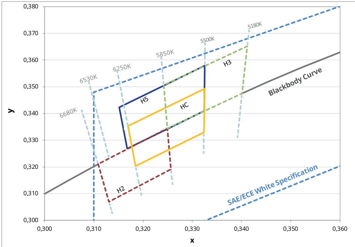
Figure 9. Color bin structure in CIE 1931 color space for LUXEON FX2 Plus Cool White.
