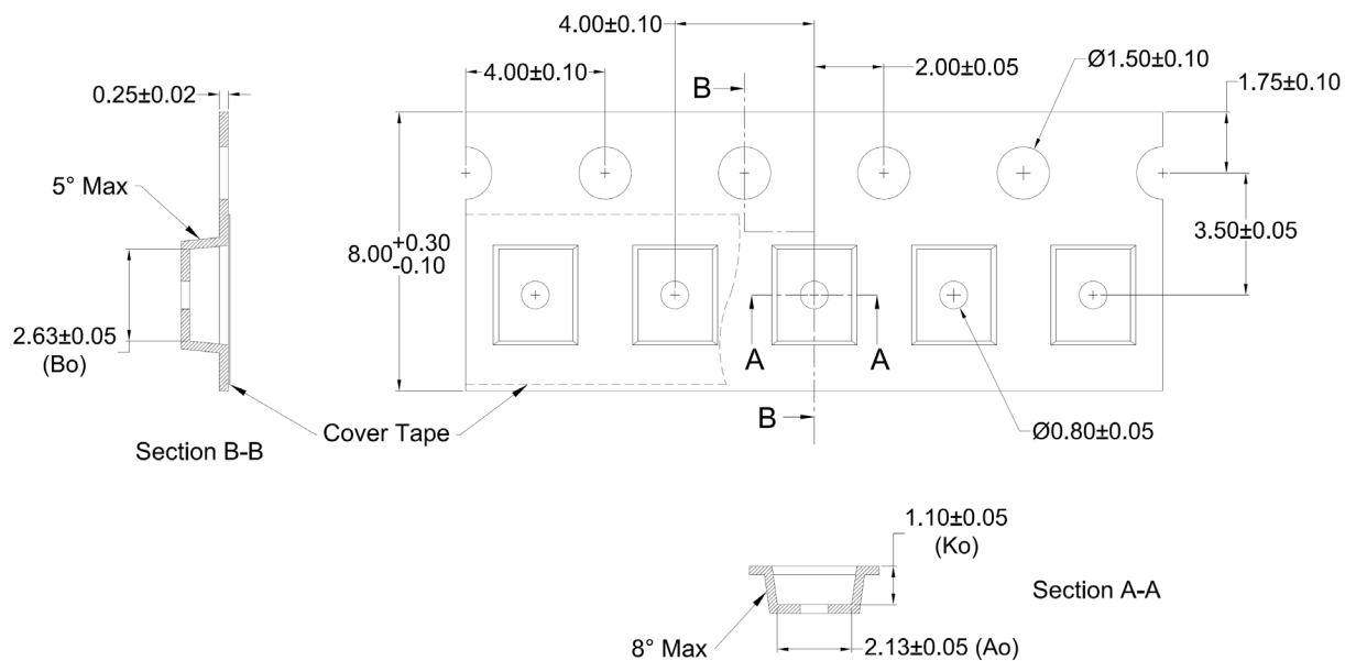
Figure 11. Pocket tape dimensions for LUXEON FX2 Plus Cool White.
