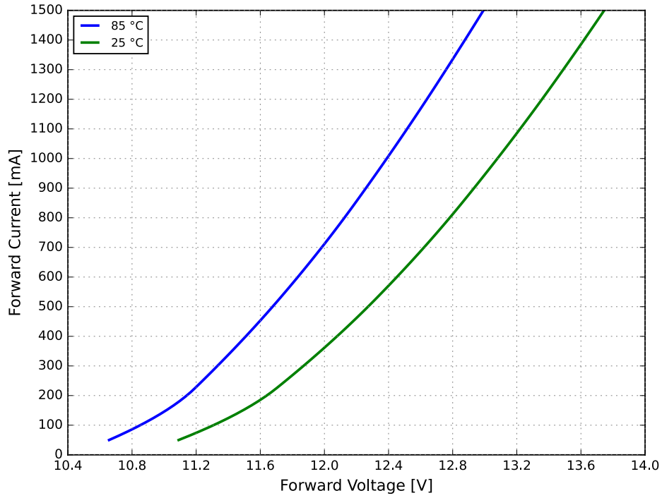
Figure 5. Typical forward current vs. forward voltage for LUXEON Altilon SMD 1x4 at MP binning temperature and at room
