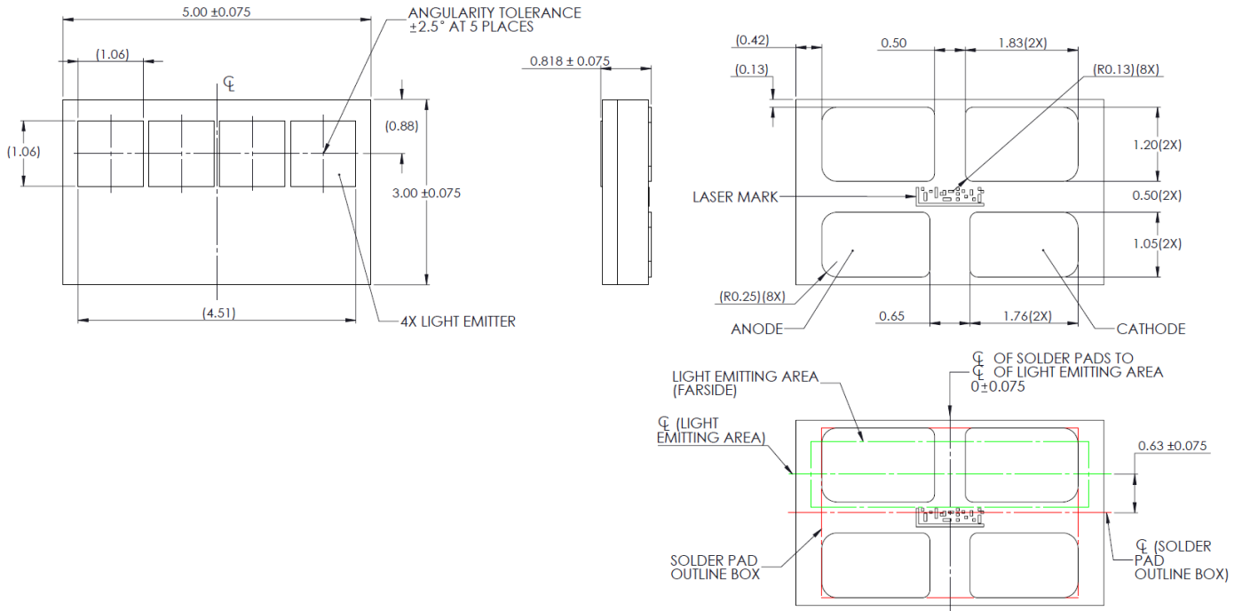
Figure 14: Mechanical Dimensions for LUXEON Altilon SMD 1x4
