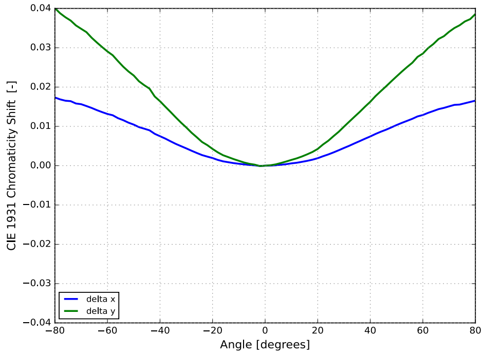
Figure 9. Typical color shift over angle for LUXEON Altilon SMD 1x4
