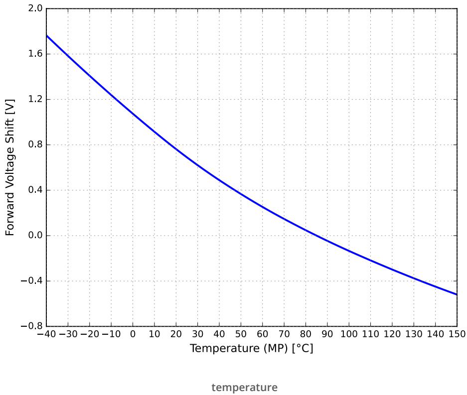
Figure 6. Typical forward voltage shift vs. temperature for LUXEON Altilon SMD 1x4 at MP binning current
