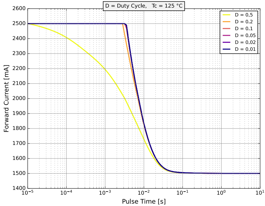
Figure 12a. Pulse handling capability for LUXEON Altilon SMD 1x4 at highest case temperature, where maximum DC current can be applied
