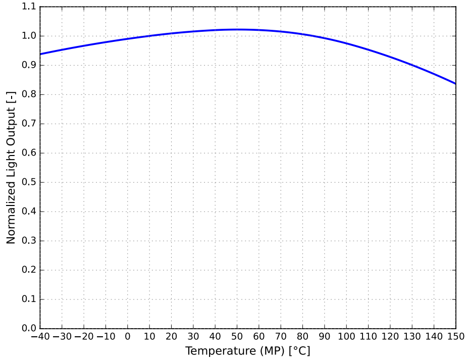
Figure 3. Typical normalized light output vs. temperature for LUXEON Altilon SMD 1x4 at MP binning current
