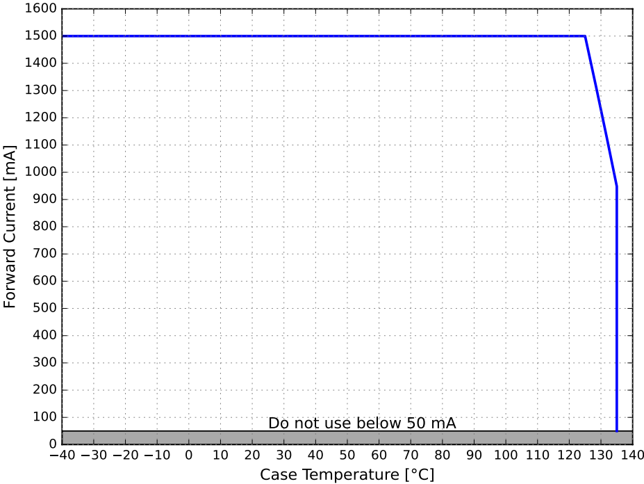
Figure 11. Maximum forward current vs. case temperature for LUXEON Altilon SMD 1x4
