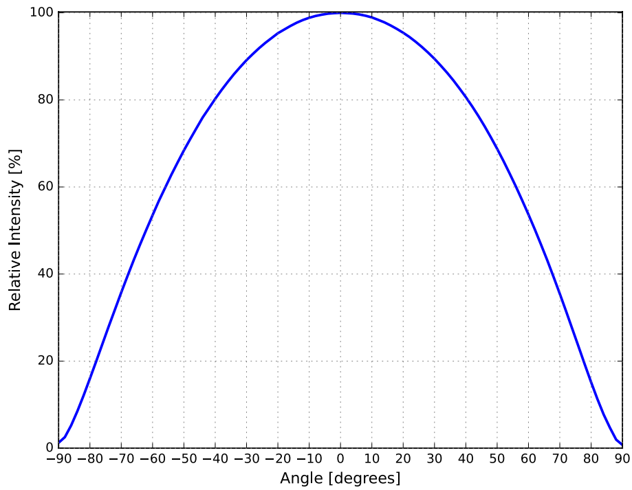
Figure 10. Typical Radiation Pattern for LUXEON Altilon SMD 1x4
