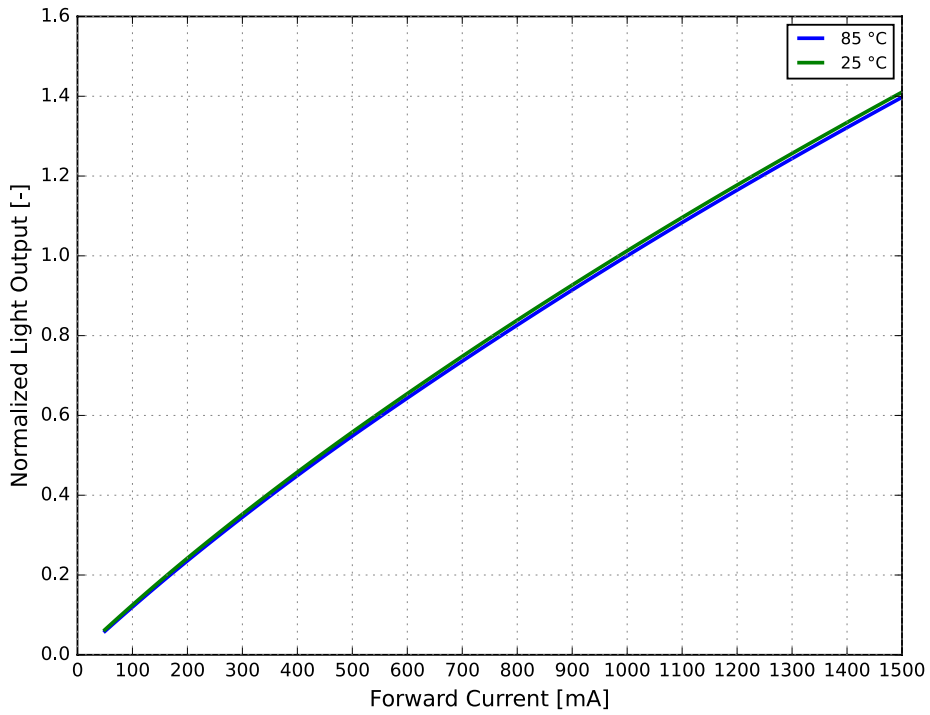
Figure 4. Typical normalized light output vs. forward current for LUXEON Altilon SMD 1x4 at MP binning temperature and at room temperature
