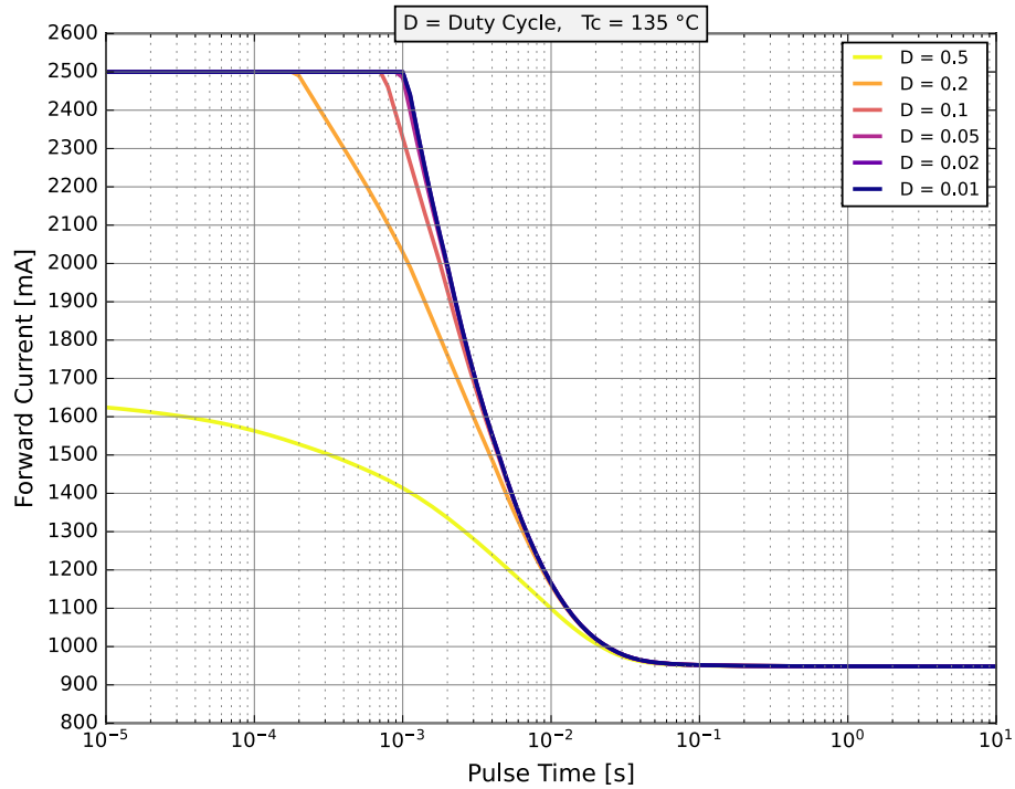
Figure 12b. Pulse handling capability for LUXEON Altilon SMD 1x4 at maximum case temperature
