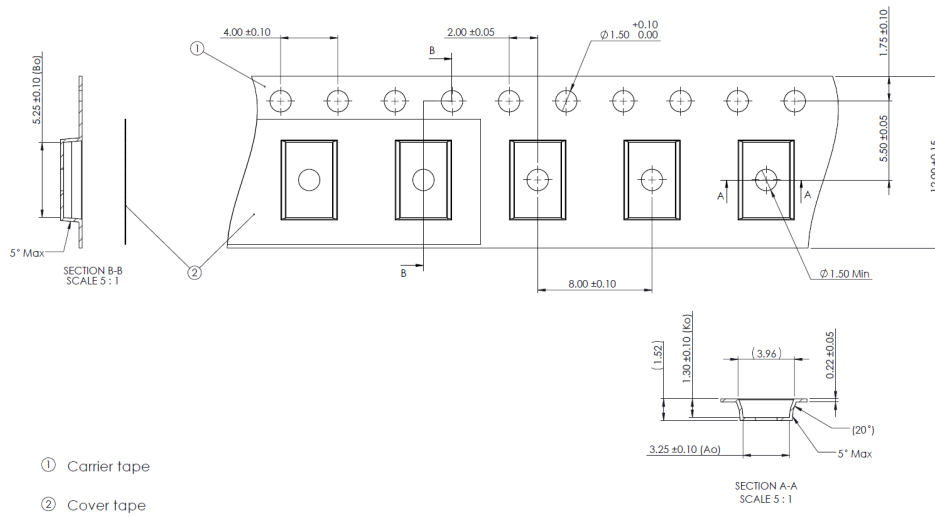
Figure 15. Pocket tape dimensions for LUXEON Altilon SMD 1x4
