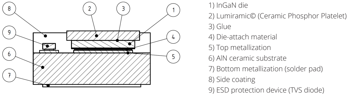
Figure 1. Schematic cross section LUXEON Altilon SMD 1x4
