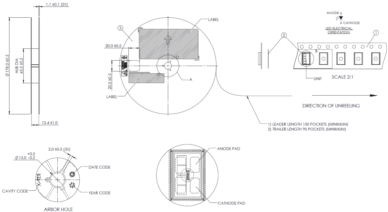
Figure 16. Reel dimensions for LUXEON Altilon SMD 1x4
