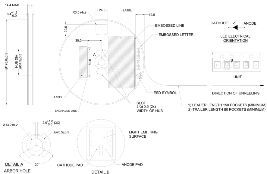
Figure 12. Reel dimensions for LUXEON FX2-L Plus Cool White.
