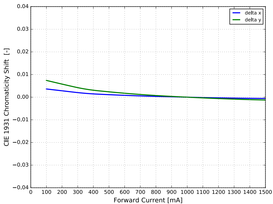
Figure 5b. Typical color shift in CIE 1931 x and y coordinates vs. forward current for LUXEON FX2-L Plus Cool White at < 20 ms MP, T c = 85 °C.
