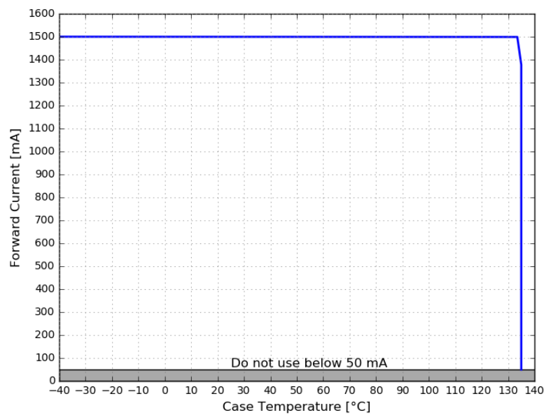
Figure 7. Maximum forward current vs. case temperature for LUXEON FX2-L Plus Cool White.
