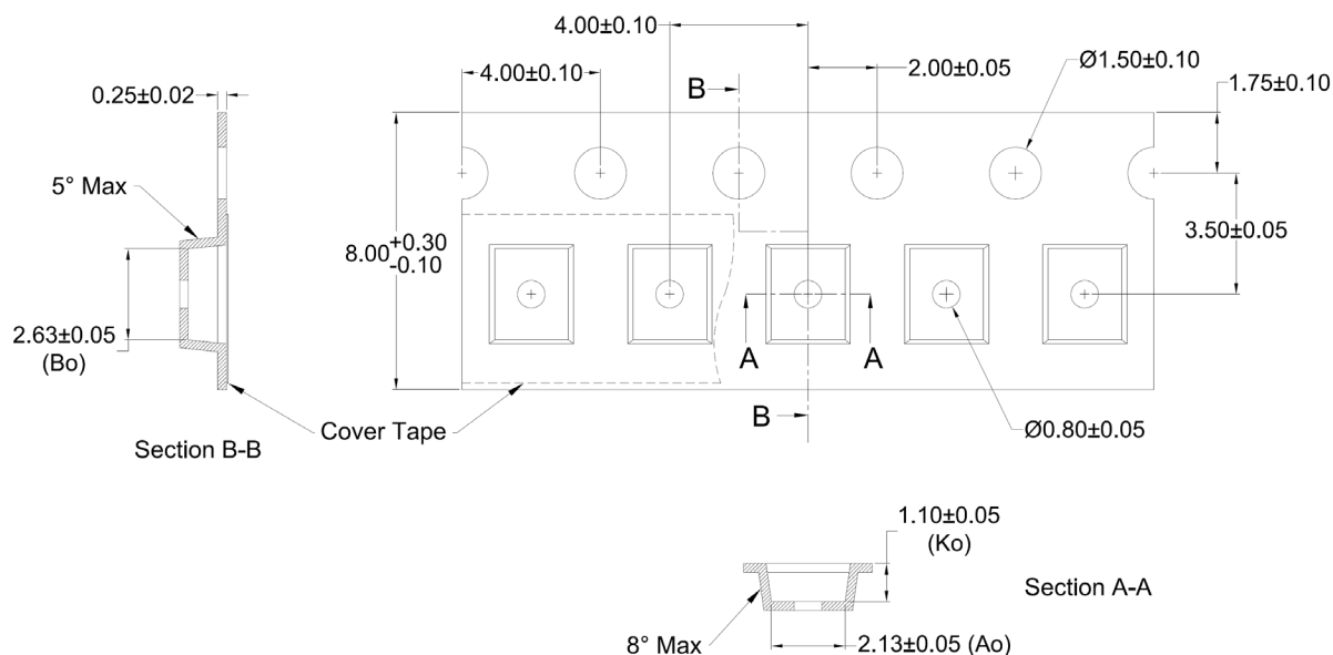
Figure 11. Pocket tape dimensions for LUXEON FX2-L Plus Cool White.
