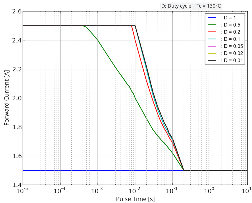
Figure 8. Permissible pulse handling capability for LUXEON FX2-L Plus Cool White.
