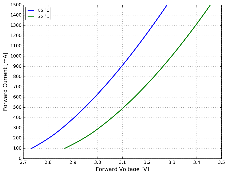
Figure 4a. Typical forward current vs. forward voltage for LUXEON FX2-L Plus Cool White at < 20 ms MP, T_c = 85^\circ\text{C} and 25^\circ\text{C} .
