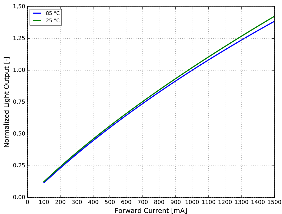
Figure 3b. Typical normalized light output vs. forward current for LUXEON FX2-L Plus Cool White at < 20 ms MP, 25°C and 85°C.
