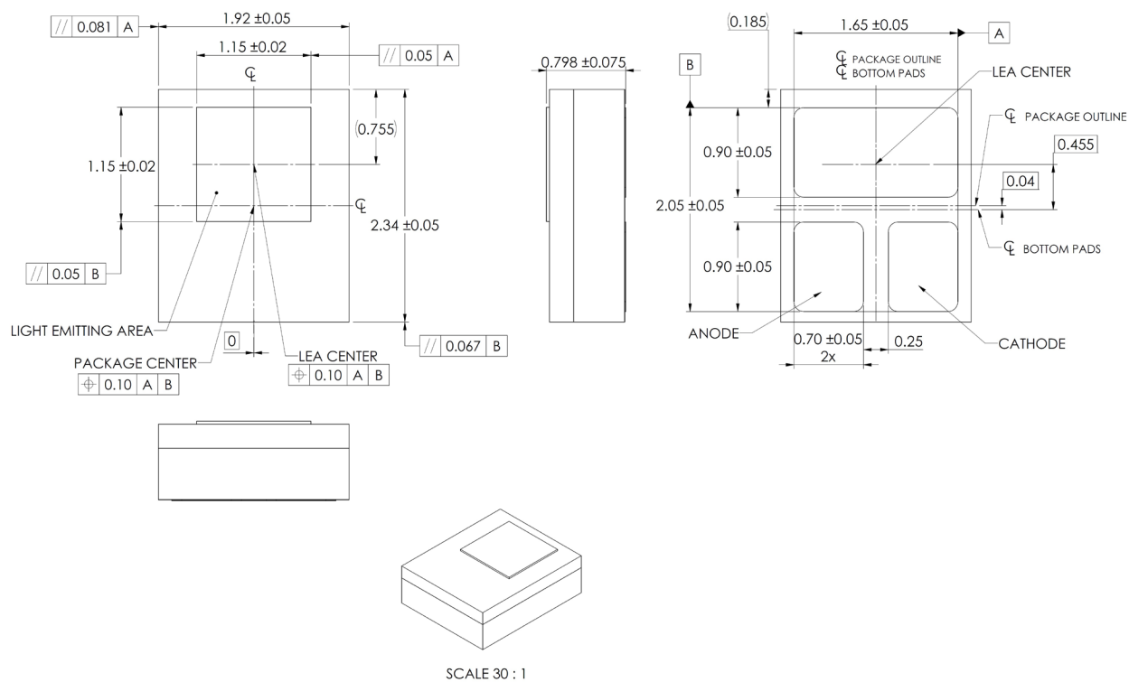
Figure 10. Mechanical dimensions for LUXEON FX2-L Plus Cool White.
