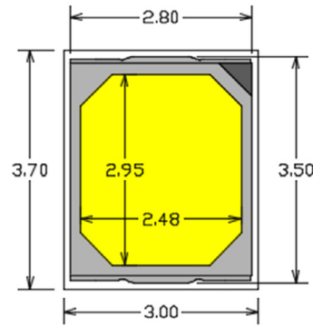
Figure 6. LUXEON 2835 Color emitter in a tape pocket with inner dimensions of 3.0mm x 3.7mm. A suitable starting point is to choose a nozzle size where the x or y dimensions or the diameter (if round nozzle) is larger than the yellow region and able to rest on the outer white plastic housing. Dimensions in mm.
