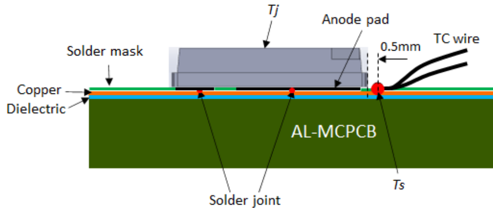
Figure 5. Cross sectional view of a two-pad LUXEON emitter on Al-MCPCB and the corresponding temperature location (top). Actual mounting of thermocouple wire closest to the anode pad of the LUXEON 2835 Color package on Al-MCPCB (bottom).
