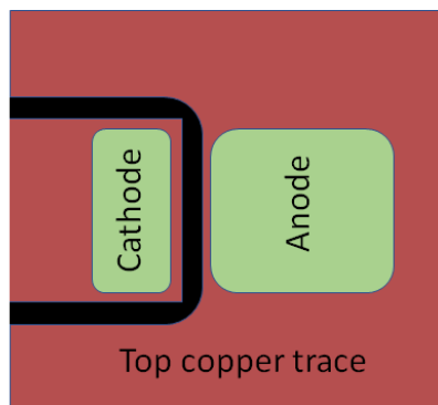
Figure 4. The top copper trace pattern is created such as to maximize the amount of copper surrounding the anode pad. The green area represents the solder mask opening and the red area represents the top copper layer.
