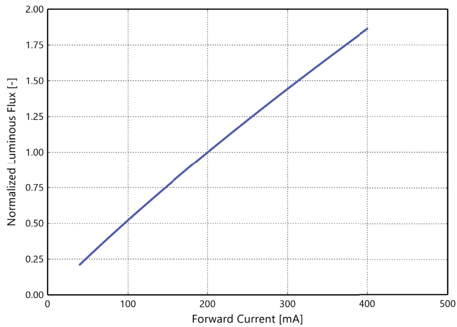
Figure 3a. Typical normalized light output vs. forward current for L2C5-xxxx1202H06Px at T j =85°C.
