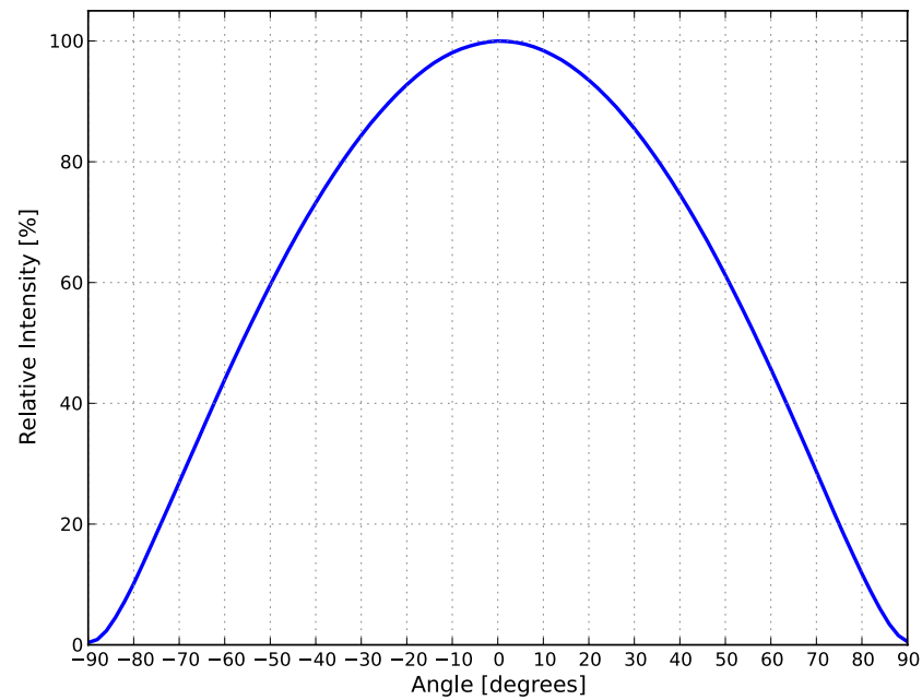
Figure 6. Typical radiation pattern for LUXEON CX Plus CoB – High Density (Below BBL) at specified test current, T_j=85^{\circ}\text{C} .
