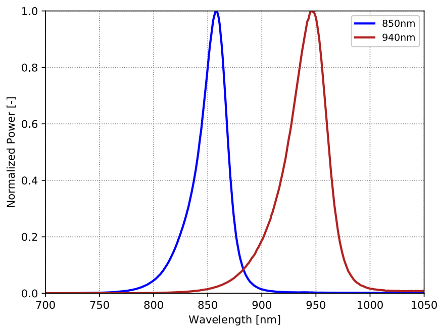
Figure 1. Typical normalized power vs. wavelength for LUXEON IR 2720 Line at 1000mA, T j =25°C.
