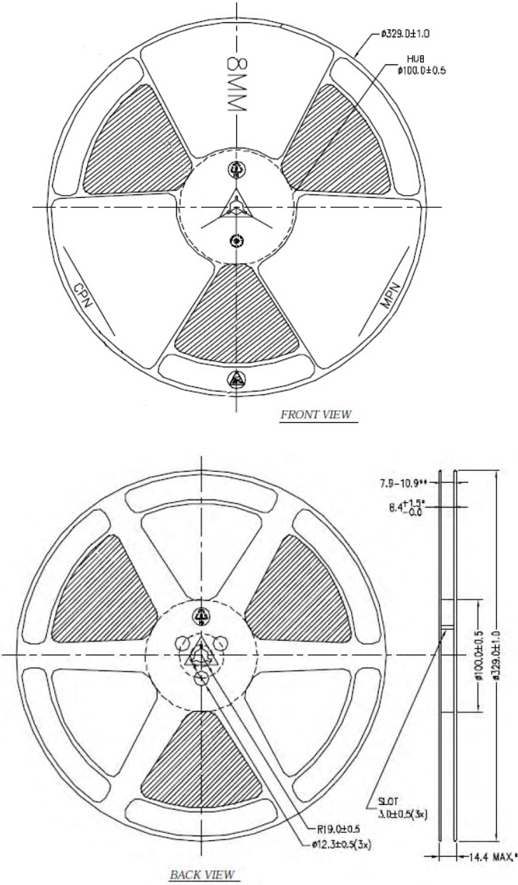
Figure 12: Reel dimensions for LUXEON Z.
