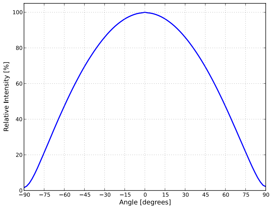
Figure 5: Typical radiation pattern for LXZ1-xxxx at 500mA, T j =85°C.
