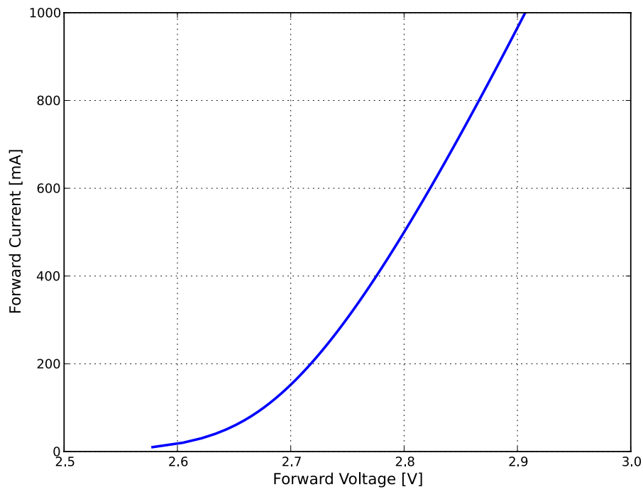
Figure 4: Typical forward current vs. forward voltage for LXZ1-xxxx at T j =85°C.
