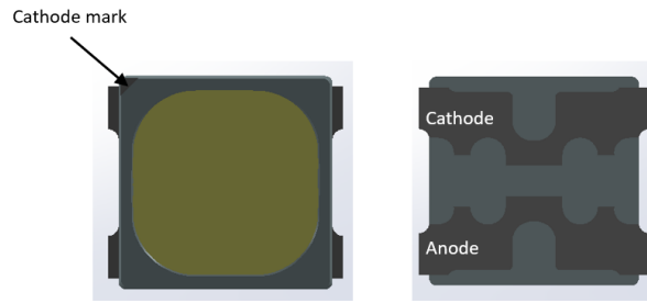
Figure 1b . Package rendering of a representative LUXEON 3030 HE Plus xD1
