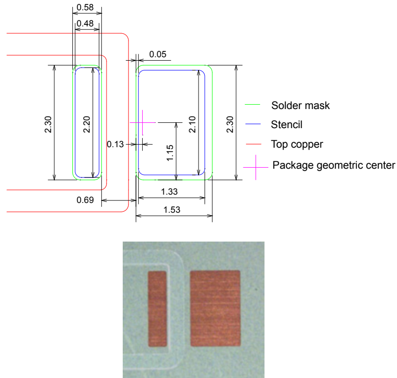
Figure 3a. Recommended PCB footprint design for the LUXEON 3030 2D Round, LUXEON 3030 2D Square, LUXEON 3030 HE, LUXEON 3030 HE Plus (except xD1) and LUXEON 3030 HV (top). In order to ensure proper heat dissipation from the package electrodes to the PCB, it is best to extend the top copper layer of the PCB several millimeters beyond the package of the LUXEON emitter. See Section 3 for more information on the copper layout. All dimensions are in mm. Bottom picture shows the actual FR4 PCB footprint layout
