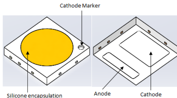
Figure 1a. Package rendering of a representative LUXEON 3030 emitter (except xD1)
