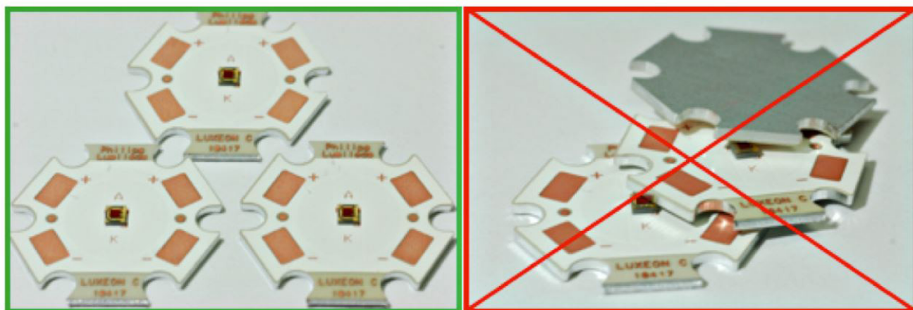
Figure 3b. Illustration of correct placement of assembled board (left) and incorrect stacking of assembled boards (right).
