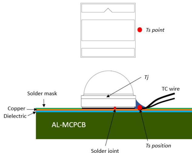
Figure 7. Drawings showing the recommended location of the T_s point (top).
