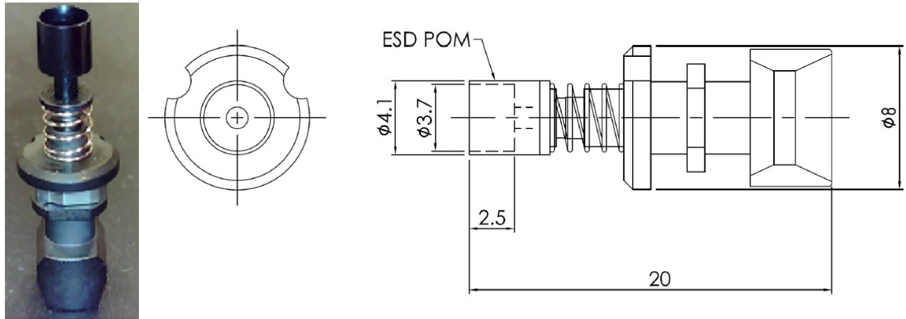
Figure 8. Nozzle design for Yamaha YS-12 (part number: LLB-2550106593 drawing number: YSM20 Nozzle from SMT ABSOLUTE Pte. Ltd.,). All dimensions are in millimeters.
