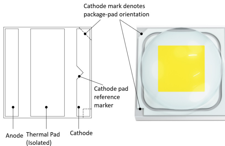
Figure 1. Bottom view (left) and top view (right) of the LUXEON HL2X-V LED.
