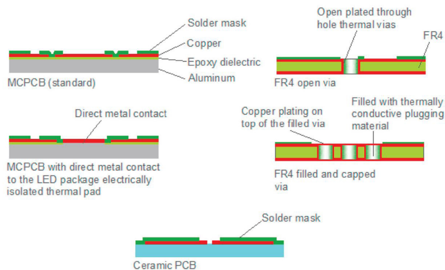
Figure 5. Schematic cross-section of MCPCB (left), FR4 (right) and ceramic (bottom) board constructions illustrate the important aspect of each board design (drawing not to scale).
