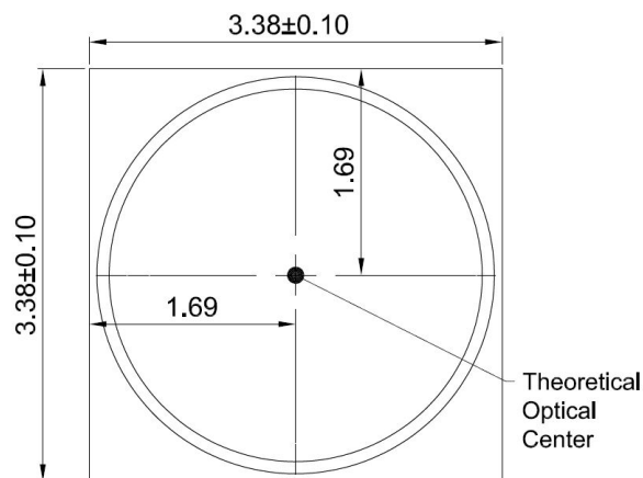
Figure 2. The theoretical optical center of LUXEON HL2X-V. All dimensions are in millimeters.
