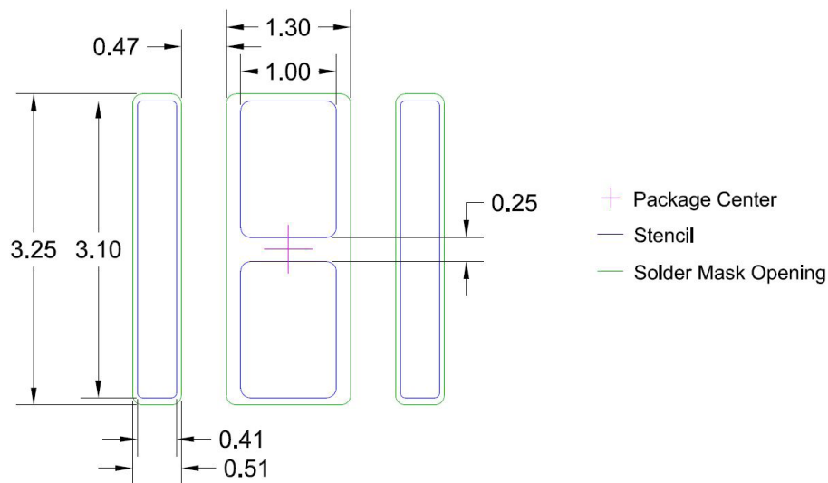
Figure 4. Recommended footprint layout for LUXEON HL2X-V. All dimensions are in millimeters.
