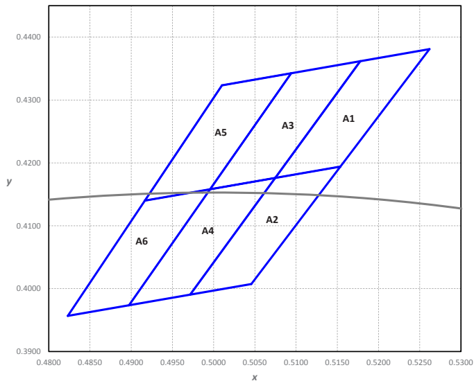
Figure 9a. Color bin structure for LUXEON 3535L Line 2200K.
