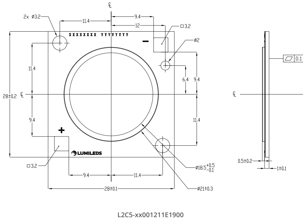
Figure 8. Mechanical dimensions for LUXEON CoB with FreshFocus Technology.
