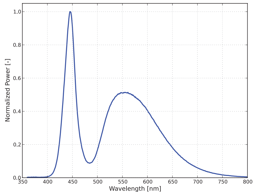
Figure 2. Typical normalized power vs. wavelength for LUXEON F ES Cool White at 20ms MP, 700mA, T_c=85^{\circ}\text{C} .
