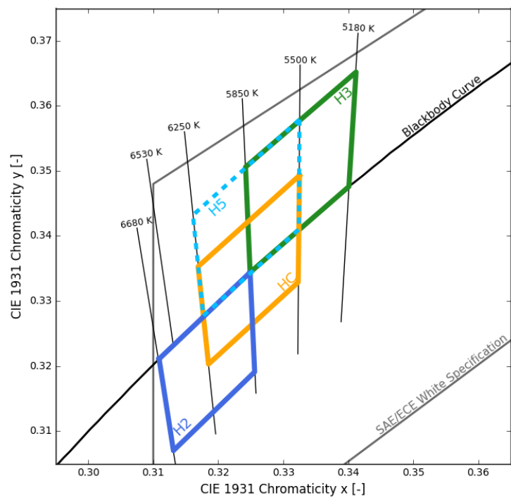
Figure 12. Color bin structure for LUXEON Versat 2016 60 Cool White
