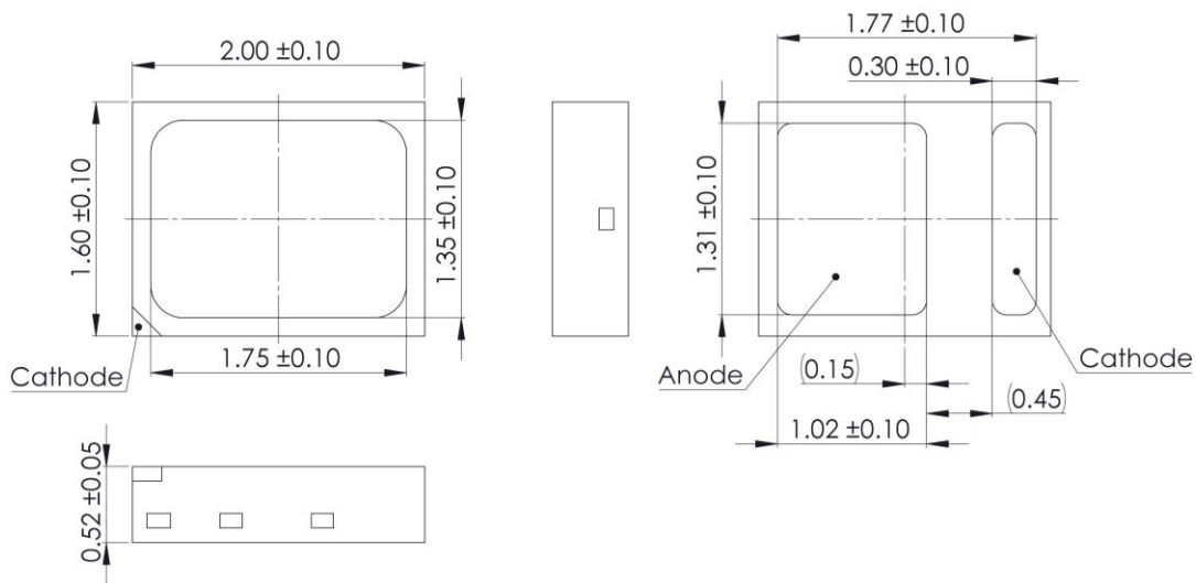
Figure 13. Mechanical dimensions for LUXEON Versat 2016 60 Cool White
