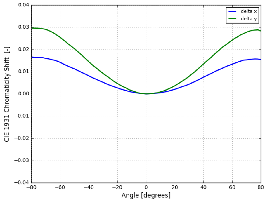
Figure 9. Typical color shift over angle for LUXEON Versat 2016 60 Cool White
