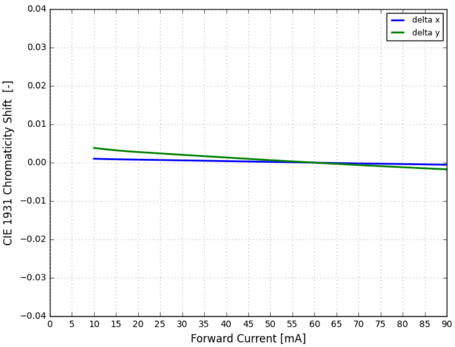
Figure 8. Typical color shift in CIE1931 x, y coordinates vs. forward current for LUXEON Versat 2016 60 Cool White at MP binning temperature
