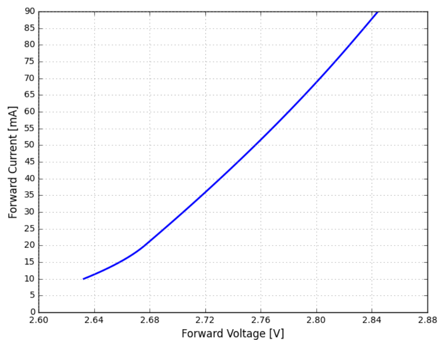
Figure 5. Typical forward current vs. forward voltage for LUXEON Versat 2016 60 Cool White at MP binning temperature
