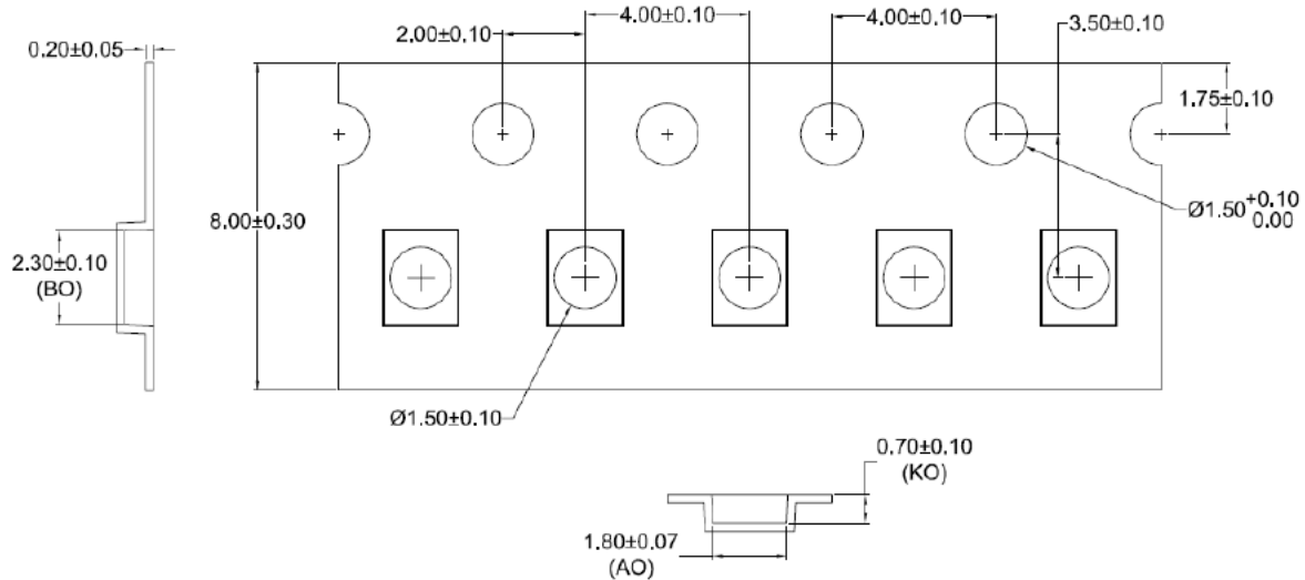
Figure 14. Pocket tape dimensions for LUXEON Versat 2016 60 Cool White
