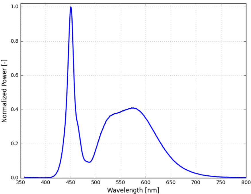
Figure 2. Typical normalized power vs. wavelength for LUXEON Versat 2016 60 Cool White at MP binning condition
