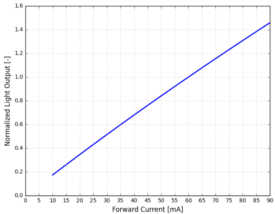
Figure 4. Typical normalized light output vs. forward current for LUXEON Versat 2016 60 Cool White at MP binning temperature
