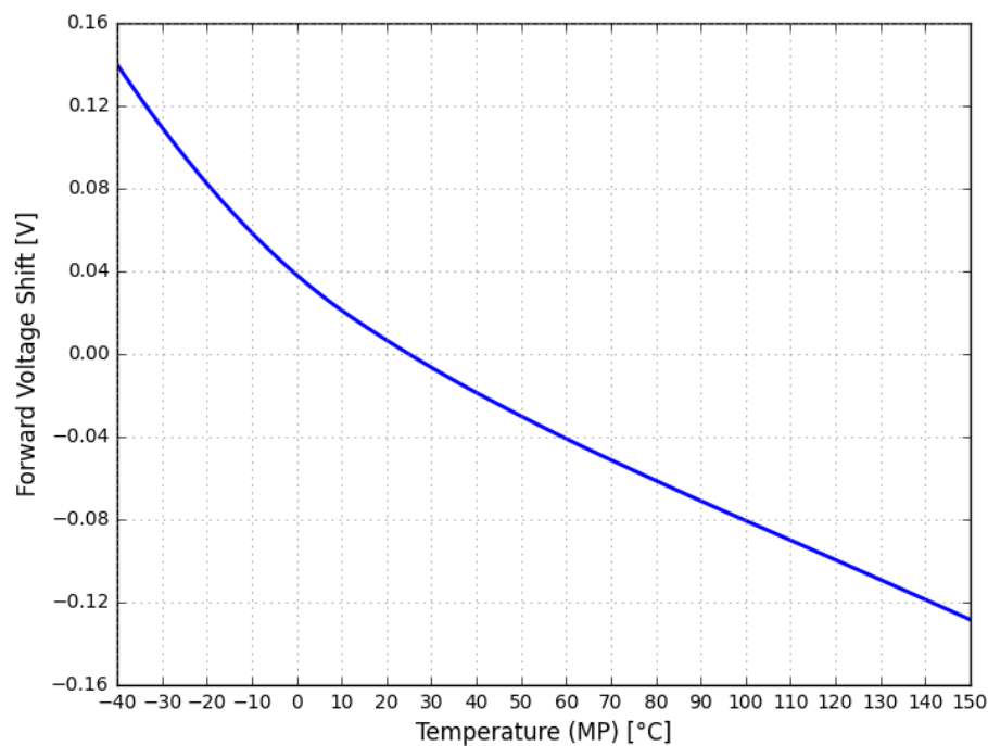
Figure 6. Typical forward voltage shift vs. temperature for LUXEON Versat 2016 60 Cool White at MP binning current
