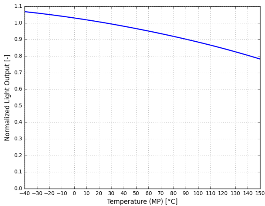
Figure 3. Typical normalized light output vs. temperature for LUXEON Versat 2016 60 Cool White at MP binning current
