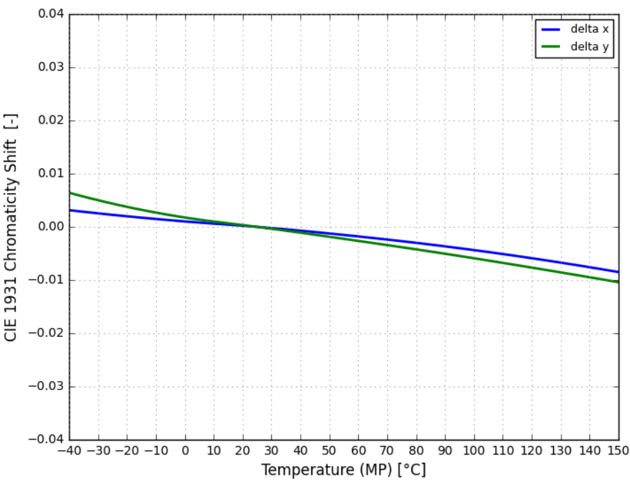
Figure 7. Typical color shift in CIE1931 x, y coordinates vs. temperature for LUXEON Versat 2016 60 Cool White at MP binning current
