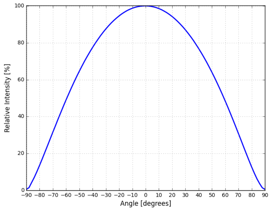
Figure 10. Typical radiation pattern for LUXEON Versat 2016 60 Cool White
