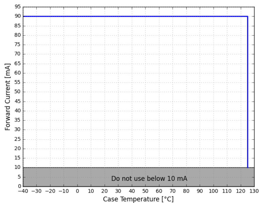
Figure 11. Maximum forward current vs. case temperature for LUXEON Versat 2016 60 Cool White
