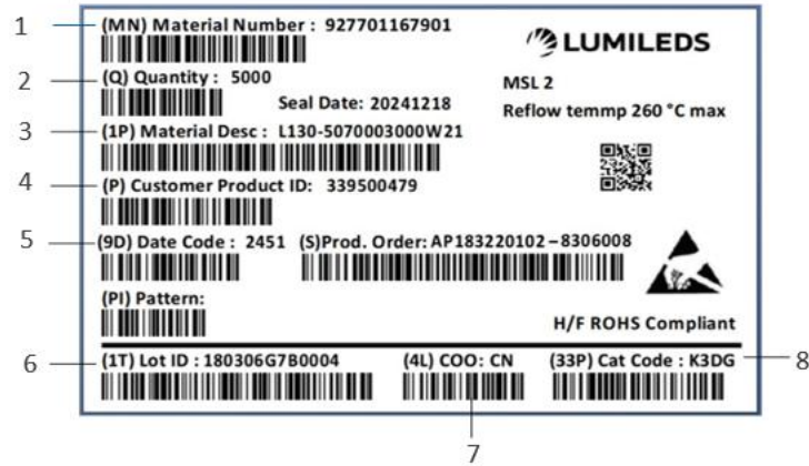
Figure 16. Example of a product label for LUXEON Versat 2016 60 Cool White
