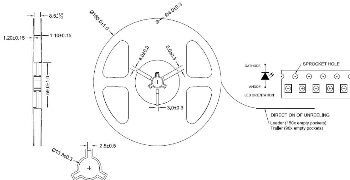
Figure 15. Reel dimensions for LUXEON Versat 2016 60 Cool White
