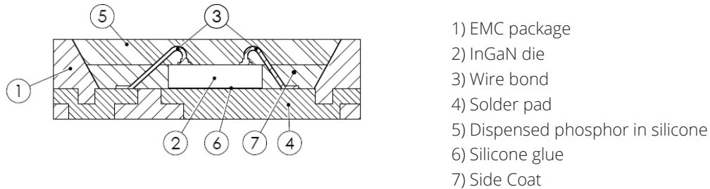
Figure 1. Schematic cross section LUXEON Versat 2016 60 Cool White
