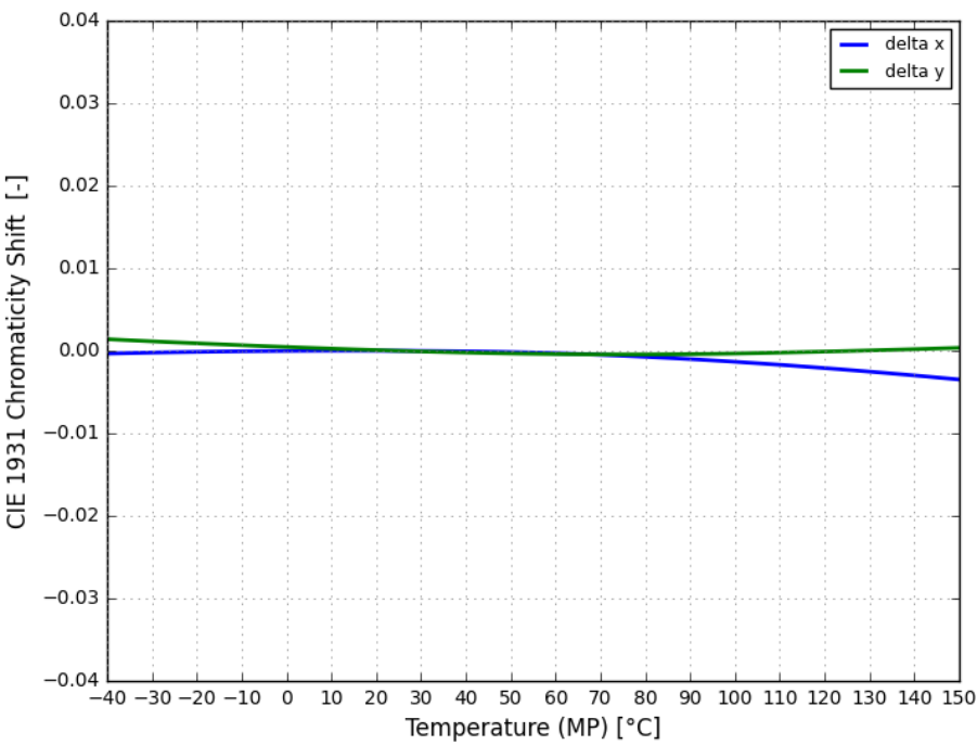
Figure 7. Typical color shift in CIE1931 x, y coordinates vs. temperature for LUXEON Versat 2016 60 PC Amber at MP binning current
