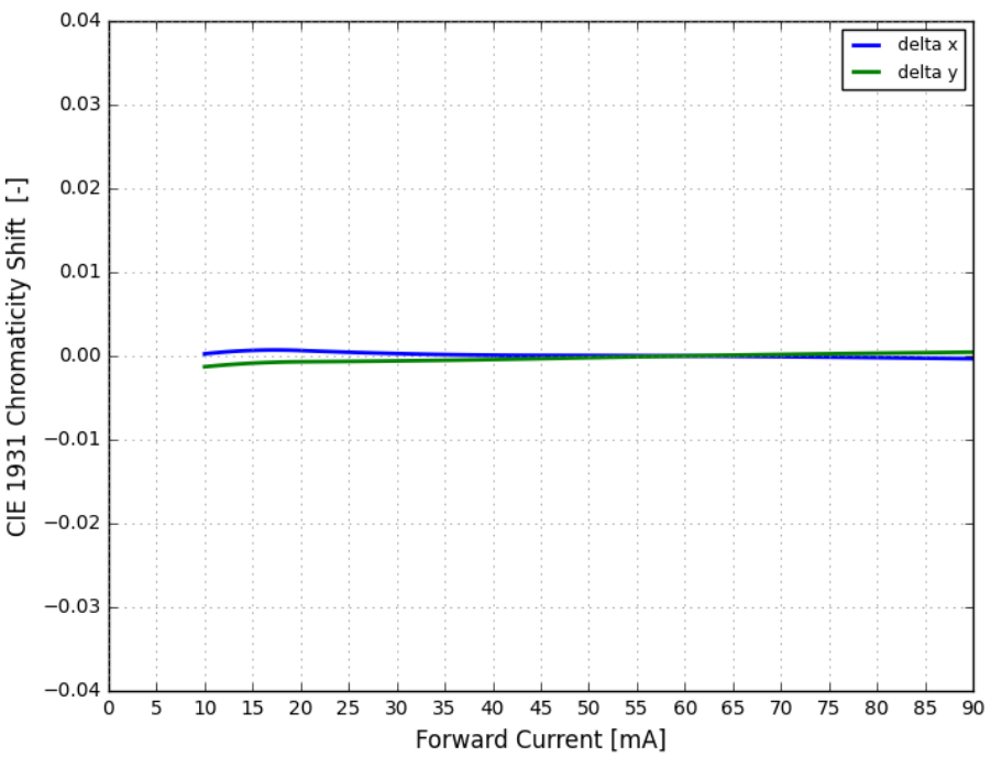
Figure 8. Typical color shift in CIE1931 x, y coordinates vs. forward current for LUXEON Versat 2016 60 PC Amber at MP binning temperature
