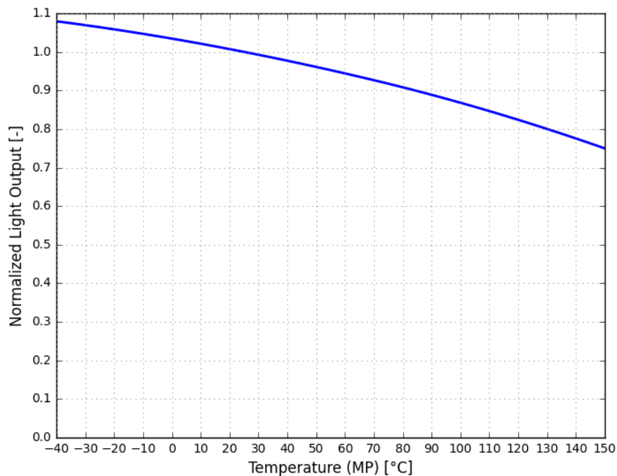
Figure 3. Typical normalized light output vs. temperature for LUXEON Versat 2016 60 PC Amber at MP binning current
