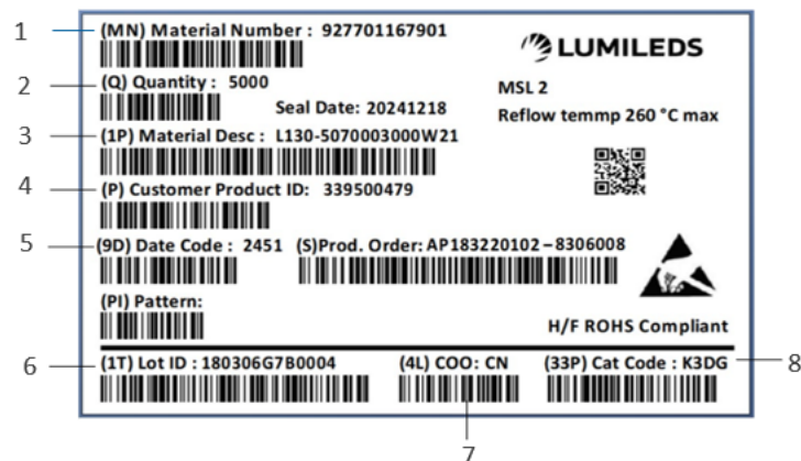
Figure 16. Example of a product label for LUXEON Versat 2016 60 PC Amber
