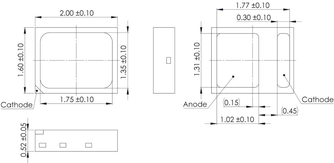
Figure 13. Mechanical dimensions for LUXEON Versat 2016 60 PC Amber
