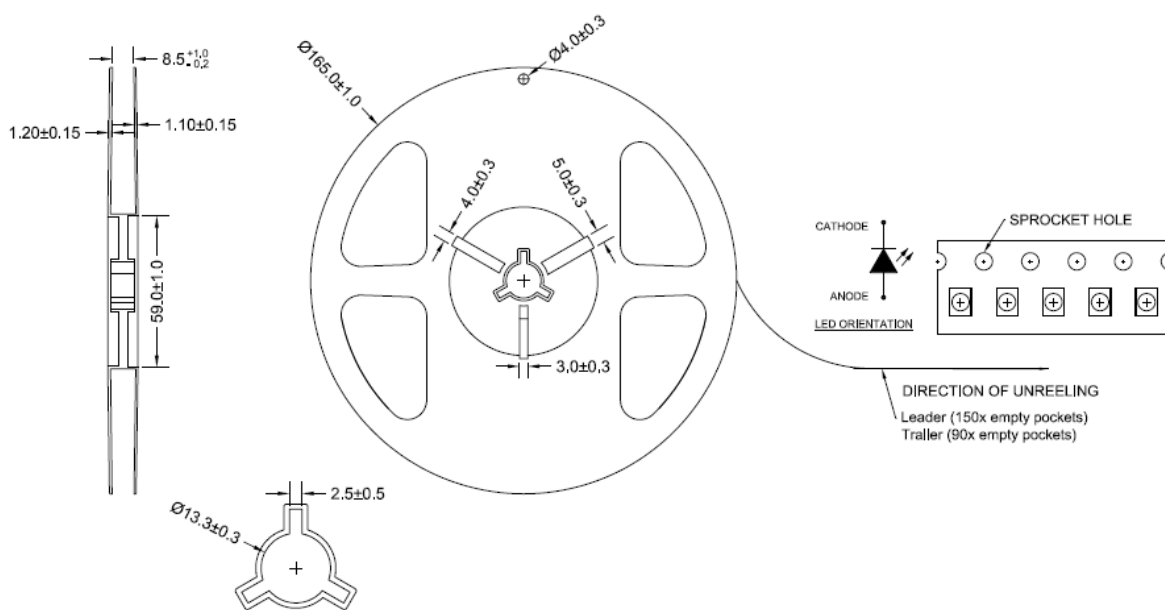
Figure 15. Reel dimensions for LUXEON Versat 2016 60 PC Amber
