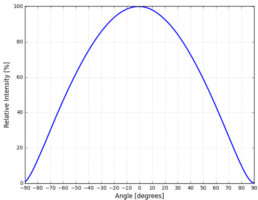
Figure 10. Typical radiation pattern for LUXEON Versat 2016 60 PC Amber
