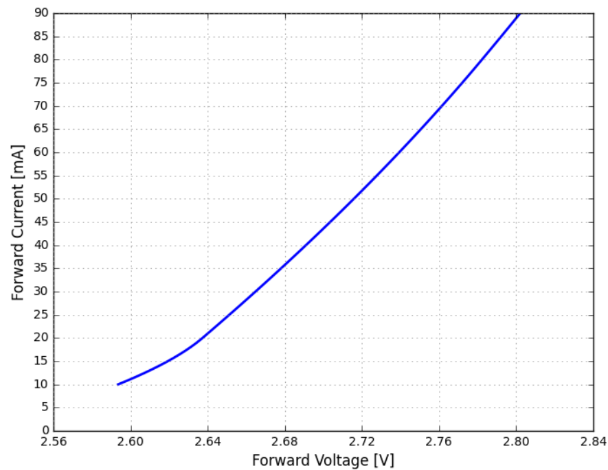
Figure 5. Typical forward current vs. forward voltage for LUXEON Versat 2016 60 PC Amber at MP binning temperature
