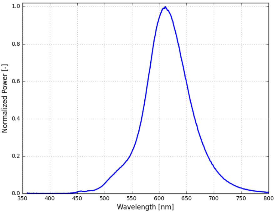
Figure 2. Typical normalized power vs. wavelength for LUXEON Versat 2016 60 PC Amber at MP binning condition
