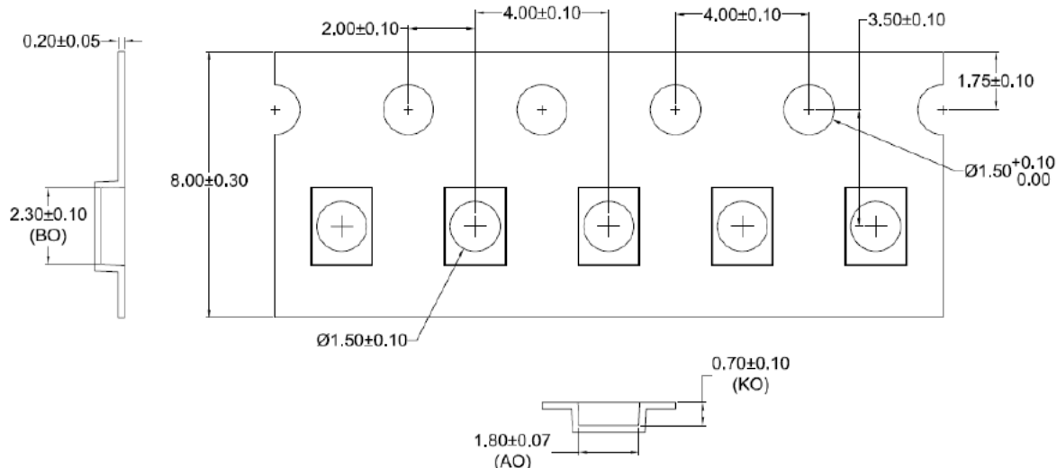
Figure 14. Pocket tape dimensions for LUXEON Versat 2016 60 PC Amber
