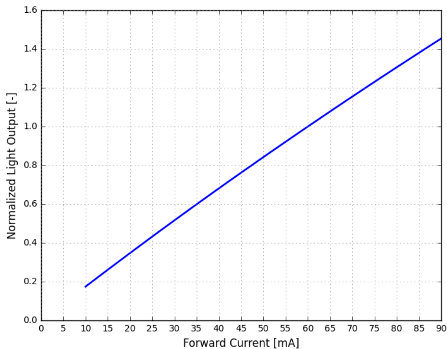
Figure 4. Typical normalized light output vs. forward current for LUXEON Versat 2016 60 PC Amber at MP binning temperature
