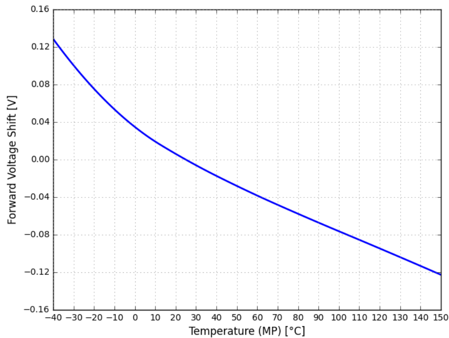
Figure 6. Typical forward voltage shift vs. temperature for LUXEON Versat 2016 60 PC Amber at MP binning current
