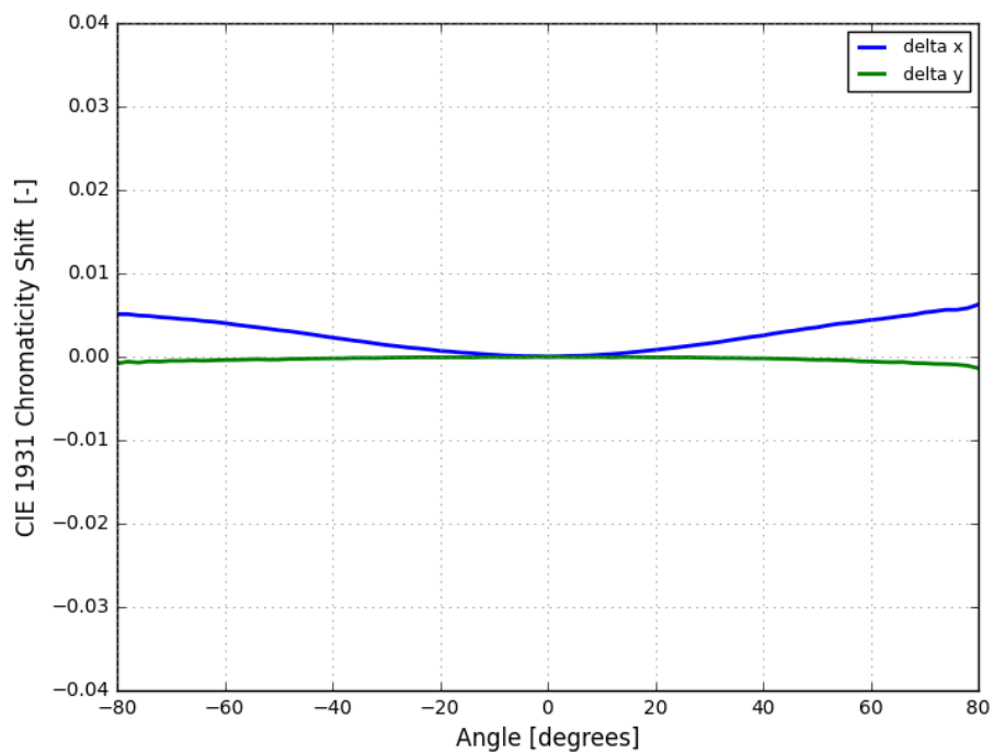
Figure 9. Typical color shift over angle for LUXEON Versat 2016 60 PC Amber
