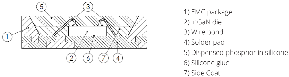
Figure 1. Schematic cross section LUXEON Versat 2016 60 PC Amber
