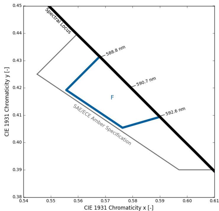
Figure 12. Color bin structure for LUXEON Versat 2016 60 PC Amber
