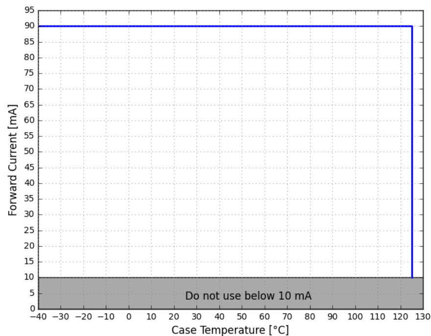
Figure 11. Maximum forward current vs. case temperature for LUXEON Versat 2016 60 PC Amber
