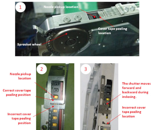
Figure 19: Three representative feeder designs. Feeder 1 does not require any modification. Feeder 2 requires the cover tape peeling position to be shifted. Feeder 3 requires the shutter to be removed before the cover tape peeling position can be adjusted.
