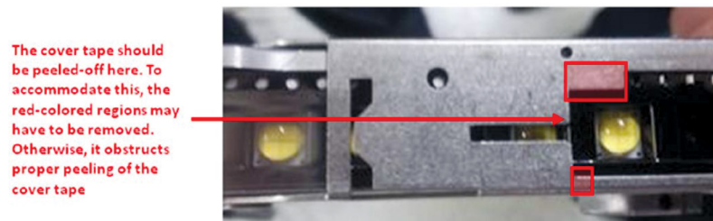
Figure 23: The cover tape peeling location in this feeder needs to be widened so that the cover tape can be peeled off without any obstruction.
