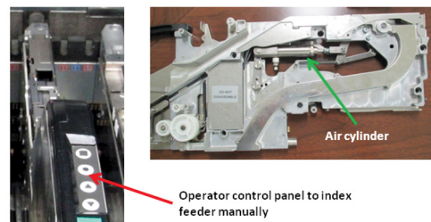
Figure 18: Examples of an electric feeder (left) and a pneumatic feeder (right) which are typically used in pick and place machines to advance the tape with LEDs.
