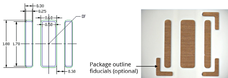
Figure 4: LUXEON SunPlus 20 PCB footprint (top). Actual LUXEON SunPlus 20 PCB with white solder mask and optional package outline fiducials (bottom). All dimensions in mm.
