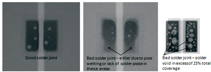
Figure 25: Example of good and bad x-ray result on a two pad LED emitter.
