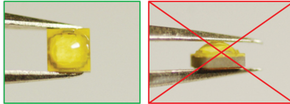
Figure 3: Correct handling (left) and incorrect handling (right) of LUXEON SunPlus 20.
