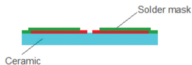
Figure 8: Cross section of ceramic based PCB. Note that there is no dielectric epoxy layer between copper (red) layer and the ceramic substrate which make ceramic PCB an excellent solution for high current operation with high density packing.
