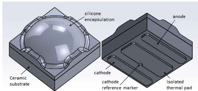
Figure 1: Image rendering of LUXEON SunPlus 20 emitter.
