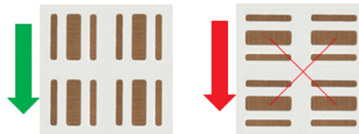
Figure 14: When possible, the PCB should be oriented such that the stencil printing direction is along the long side of the pads (green arrow, left picture). Avoid the stencil printing direction perpendicular to the long side of the pads (red arrow, right picture).
