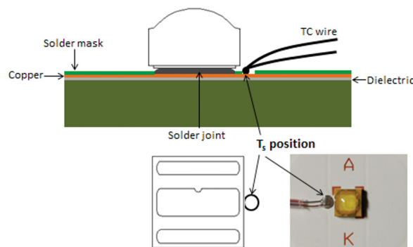
Figure 26: T_s location for LUXEON SunPlus 20 mounted on PCB. Place the TC wire as close as possible to the LUXEON SunPlus 20 thermal pad.
