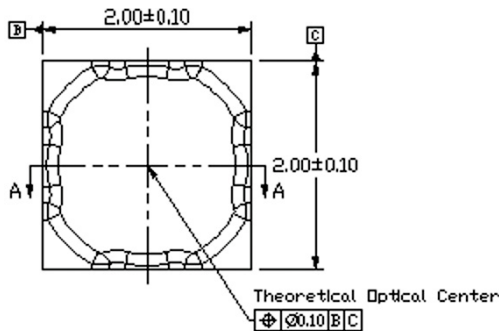
Figure 2: Optical center. All dimensions in mm.
