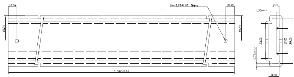
Figure 7b. Tube dimensions for L2C5-SPx11211E1900.
