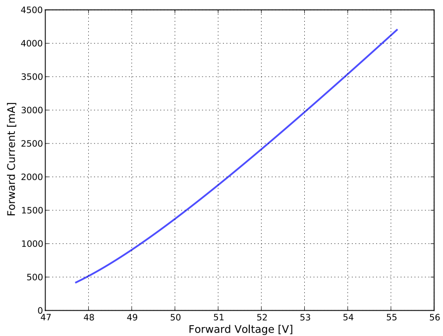
Figure 3c. Typical forward current vs. forward voltage for L2C5-SPx11825G3200 at T_j = 85^\circ\text{C} .
