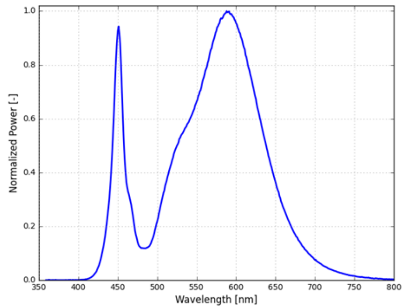
Figure 2. Typical normalized power vs. wavelength for LUXEON Versat 2016 60 3570 at MP binning condition
