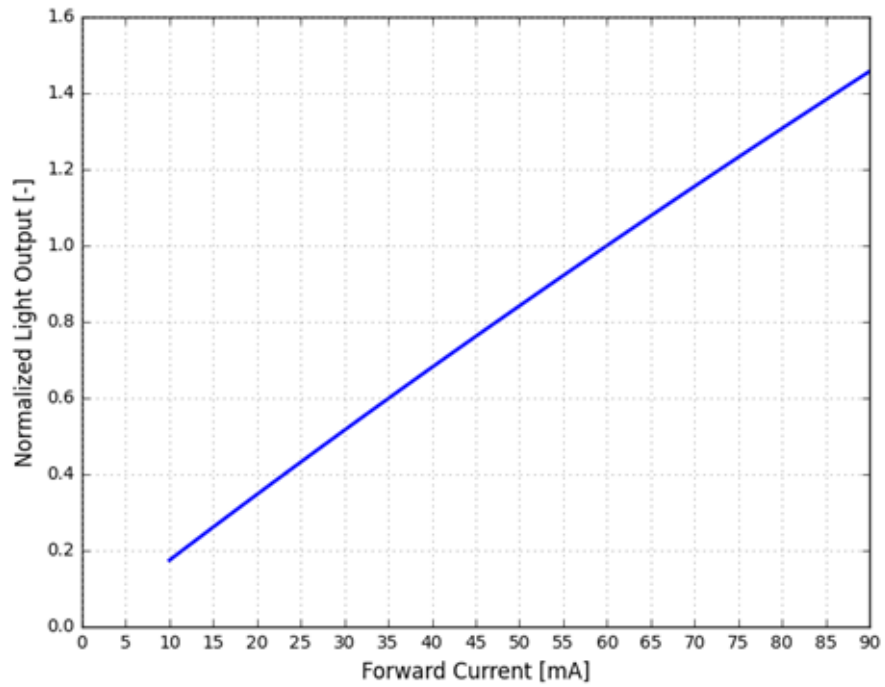
Figure 4. Typical normalized light output vs. forward current for LUXEON Versat 2016 60 3570 at MP binning temperature
