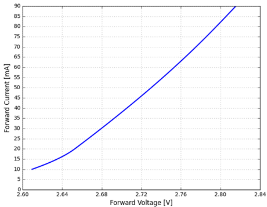
Figure 5. Typical forward current vs. forward voltage for LUXEON Versat 2016 60 3570 at MP binning temperature
