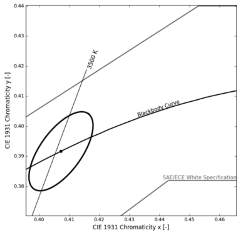
Figure 12. Color bin structure for LUXEON Versat 2016 60 3570
