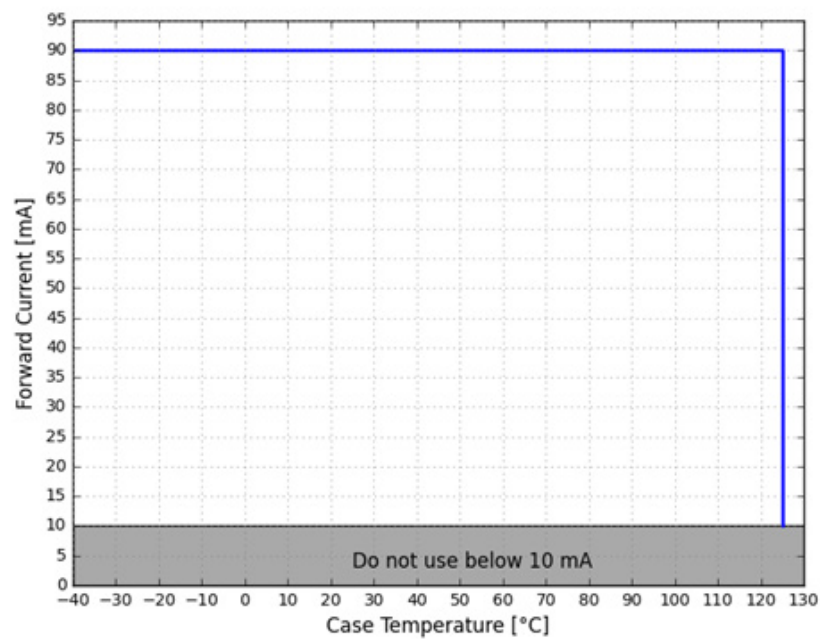
Figure 11. Maximum forward current vs. case temperature for LUXEON Versat 2016 60 3570
