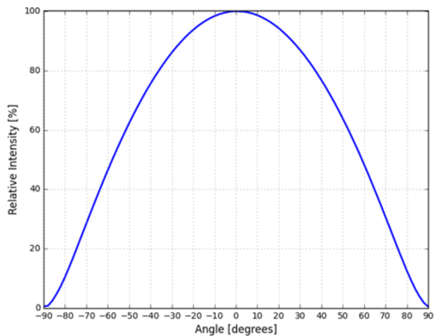
Figure 10. Typical radiation pattern for LUXEON Versat 2016 60 3570
