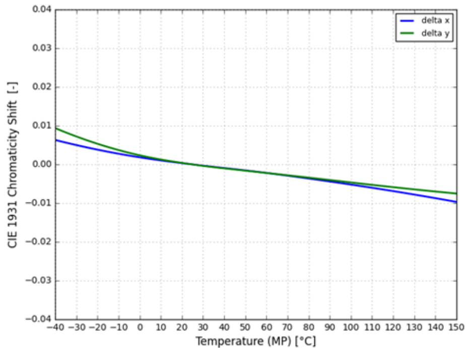
Figure 7. Typical color shift in CIE1931 x, y coordinates vs. temperature for LUXEON Versat 2016 60 3570 at MP binning current
