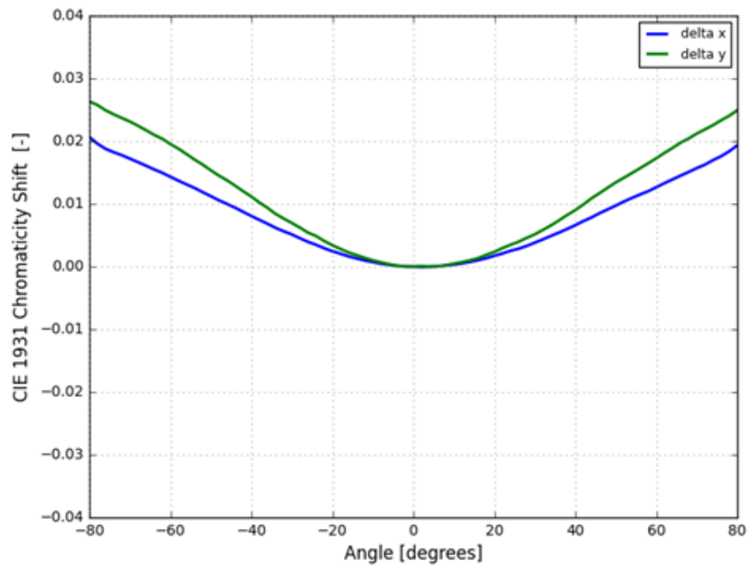
Figure 9. Typical color shift over angle for LUXEON Versat 2016 60 3570
