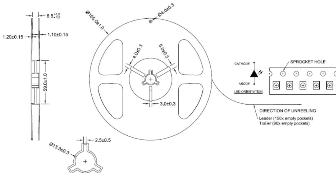
Figure 16. Reel dimensions for LUXEON Versat 2016 60 3570
