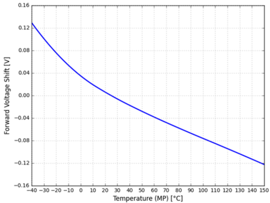
Figure 6. Typical forward voltage shift vs. temperature for LUXEON Versat 2016 60 3570 at MP binning current
