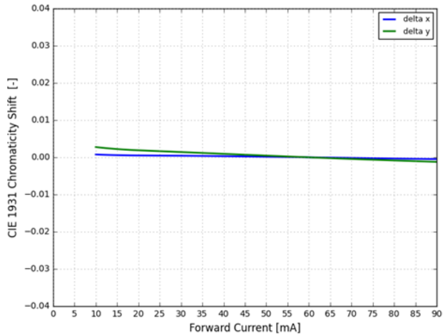
Figure 8. Typical color shift in CIE1931 x, y coordinates vs. forward current for LUXEON Versat 2016 60 3570 at MP binning temperature
