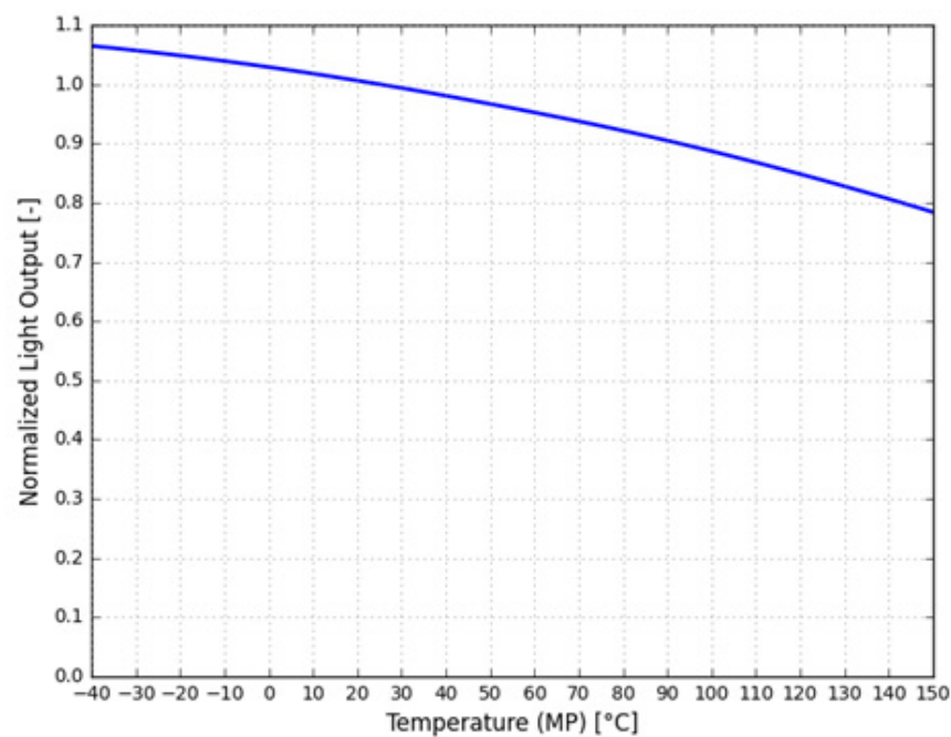
Figure 3. Typical normalized light output vs. temperature for LUXEON Versat 2016 60 3570 at MP binning current
