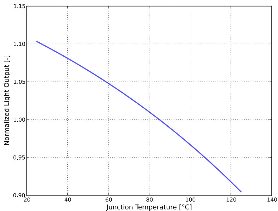
Figure 2. Typical normalized light output vs. junction temperature for L2C5-xxxx12xxxxP0 at specified test current.
