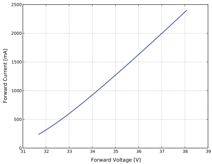
Figure 4e. Typical forward current vs. forward voltage for L2C5-xxxx1211FxxP0 at T_j=85^{\circ}\text{C} .
