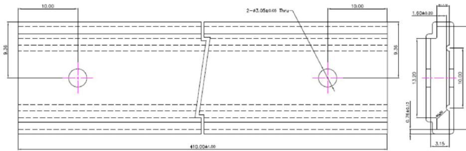
Figure 9a. Tube dimensions for L2C5-xxxx1203F09P0.
