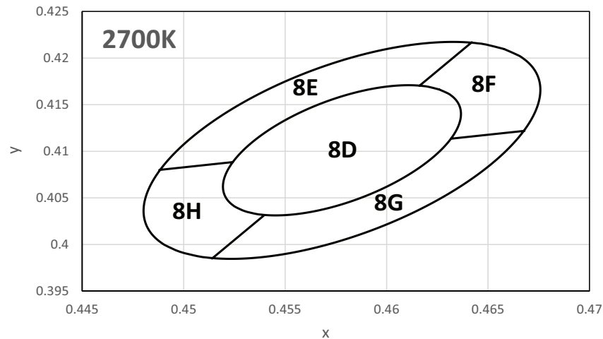
Figure 2a. 1/5 th color bin structure for LUXEON 2835 Commercial 2700K at specified test current and binning temperature of T_j=25^{\circ}\text{C} .
