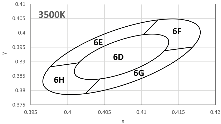
Figure 2c. 1/5 th color bin structure for LUXEON 2835 Commercial 3500K at specified test current and binning temperature of T_j=25^{\circ}\text{C} .
