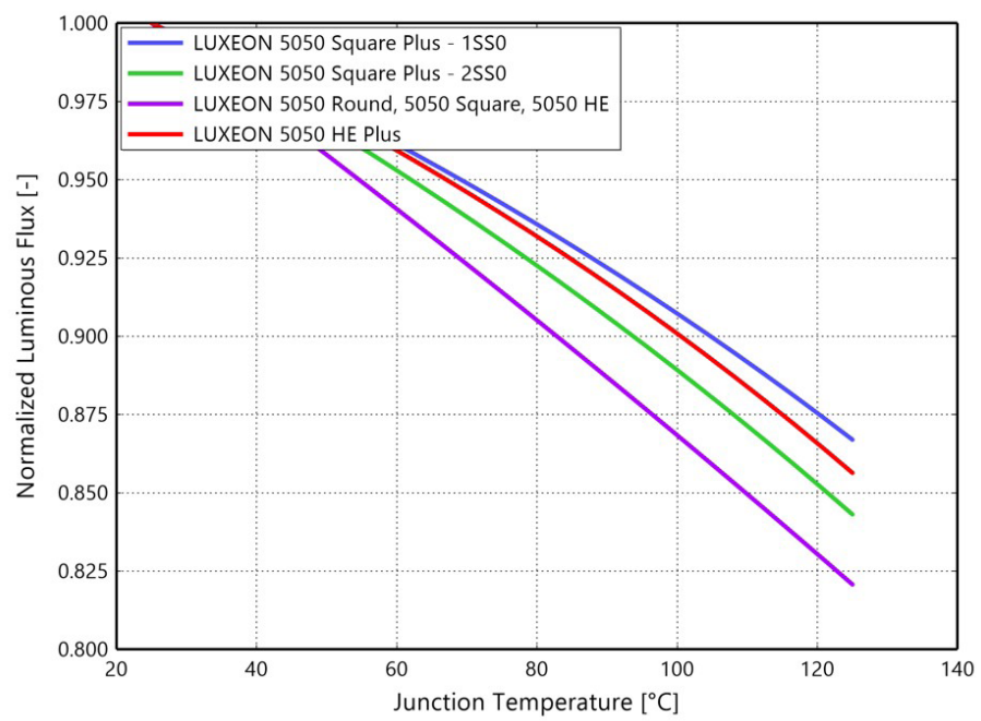
Figure 3a. Typical normalized light output vs. junction temperature for all LUXEON 5050 at test current
