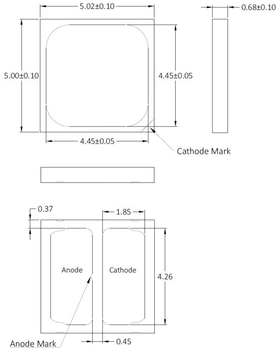
Figure 8C. Mechanical dimensions for LUXEON 5050 Square Plus
