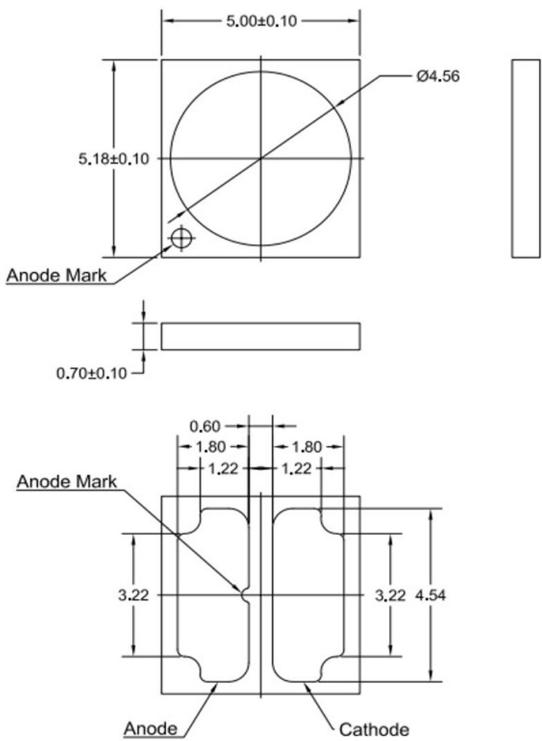
Figure 8a. Mechanical dimensions for LUXEON 5050 Round LES
