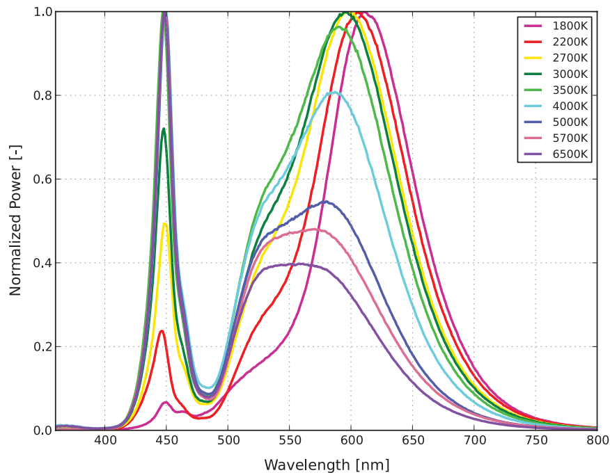
Figure 2a. Typical normalized power vs. wavelength for 70CRI LUXEON 5050 at test current, T_j=25^{\circ}\text{C}
