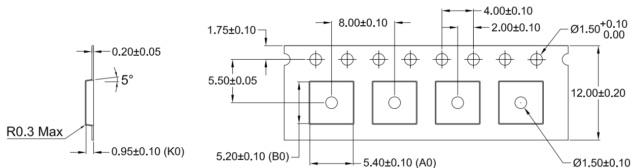
Figure 11a. Pocket Tape dimensions for LUXEON 5050 Round LES, LUXEON 5050 Square LES, LUXEON 5050 HE and LUXEON 5050 HE Plus
