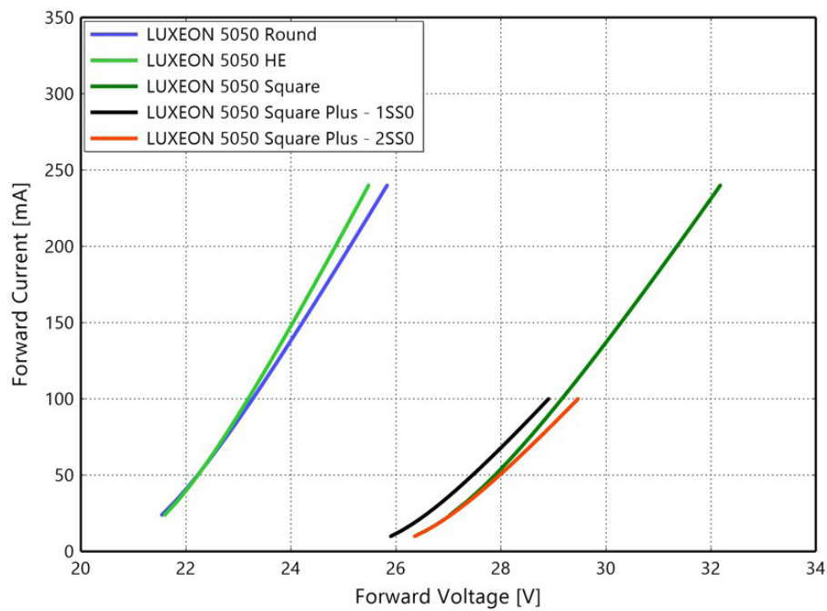
Figure 4b. Typical forward current vs. forward voltage for LUXEON 5050 - 24V/30V, T_j=25^{\circ}\text{C}
