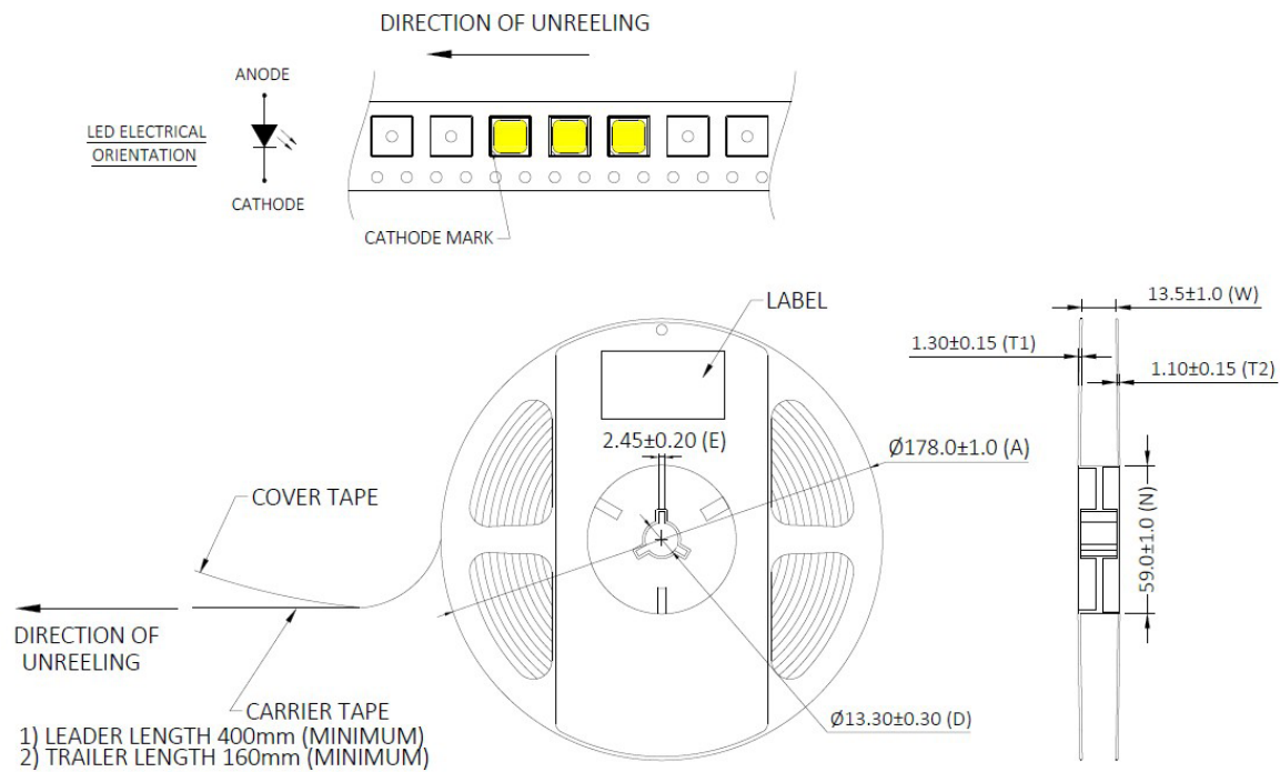
Figure 12c. Reel dimensions for LUXEON 5050 Square Plus
