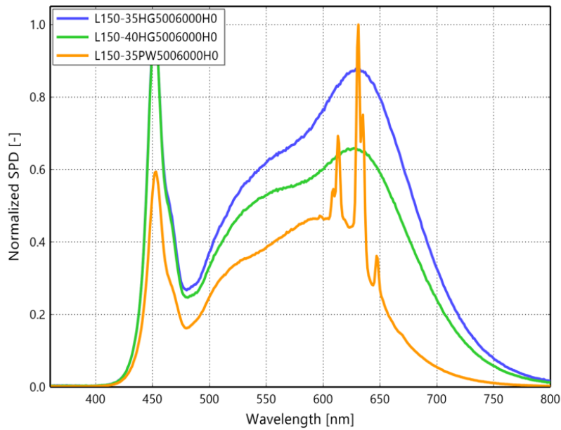
Figure 2d. Typical normalized power vs. wavelength for LUXEON 5050 HE - Crisp Color and Premium White at test current, T_j=25^{\circ}\text{C}
