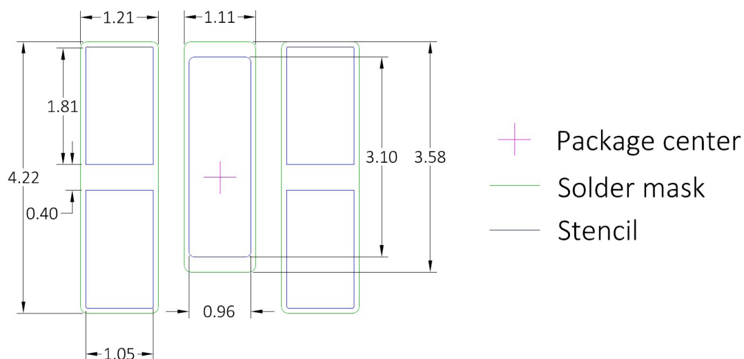
Figure 10b. Recommended PCB solder pad layout for LUXEON 5050 Square LES and LUXEON 5050 Square Plus
