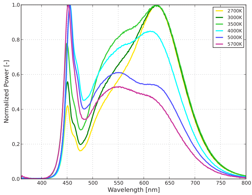
Figure 2c. Typical normalized power vs. wavelength for 90CRI LUXEON 5050 at test current, T_j=25^{\circ}\text{C}
