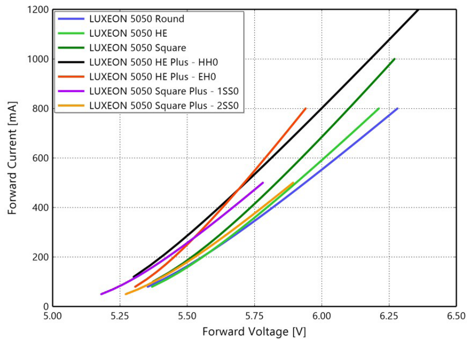
Figure 4a. Typical forward current vs. forward voltage for LUXEON 5050 - 6V, T_j=25^{\circ}\text{C}
