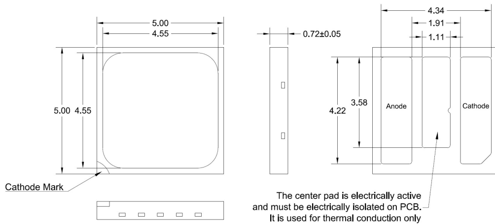
Figure 8e. Mechanical dimensions for LUXEON 5050 HE Plus EH0
