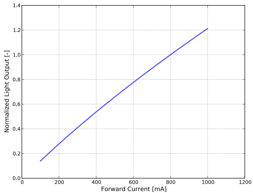
Figure 3d. Typical normalized light output vs. forward current for LUXEON 5050 Square LES - 6V, T_j = 25^\circ\text{C}
