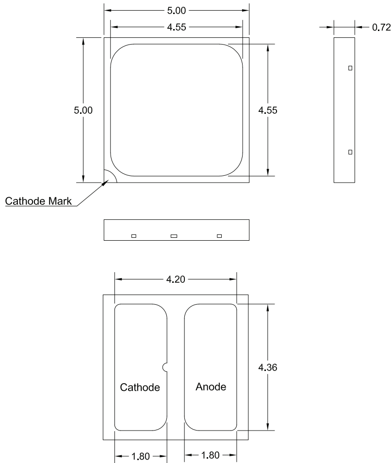
Figure 8d. Mechanical dimensions for LUXEON 5050 HE and LUXEON 5050 HE Plus HH0
