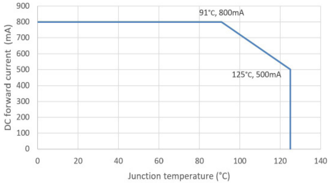
Figure 1a. Maxium DC Forward Current of LUXEON 5050 Square Plus
