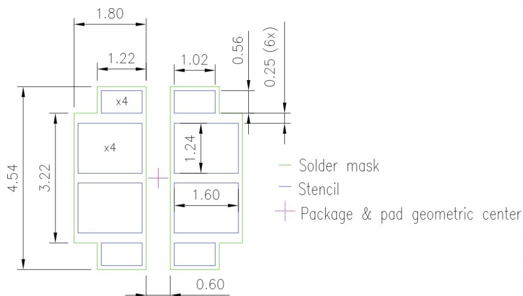
Figure 10a. Recommended PCB solder pad layout for LUXEON 5050 Round LES, LUXEON 5050 HE and LUXEON 5050 HE Plus - HH0
