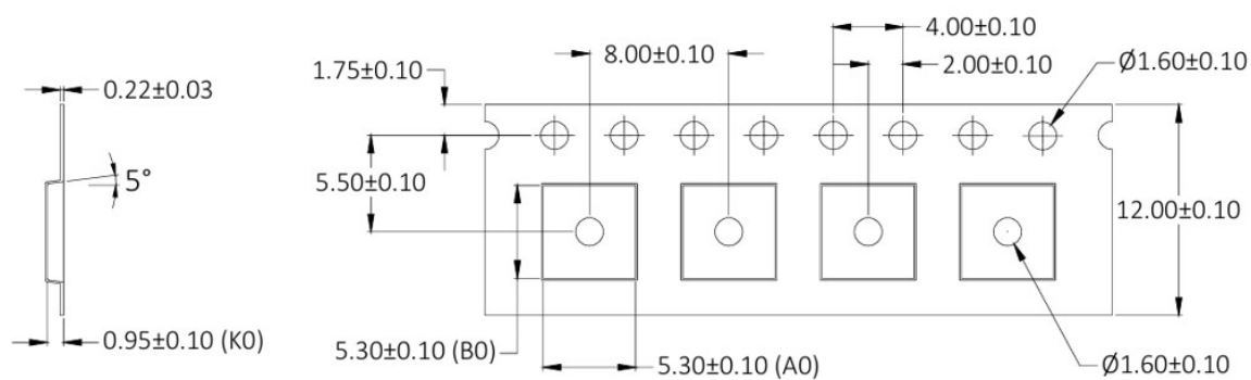
Figure 11b. Pocket Tape dimensions for LUXEON 5050 Square LES, LUXEON 5050 Square Plus
