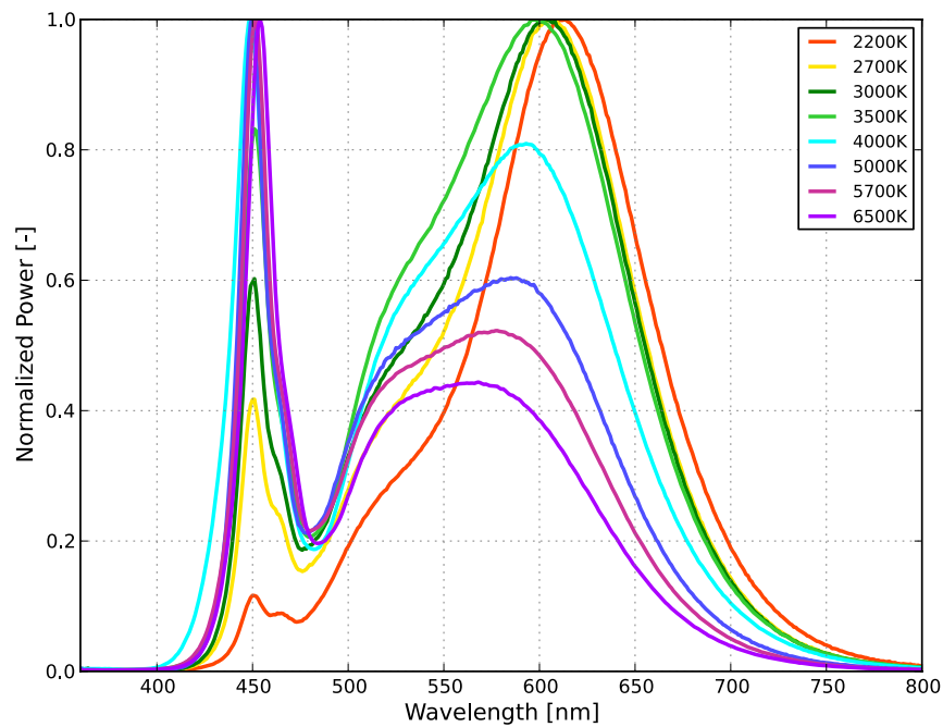
Figure 2b. Typical normalized power vs. wavelength for 80CRI LUXEON 5050 at test current, T_j=25^{\circ}\text{C}
