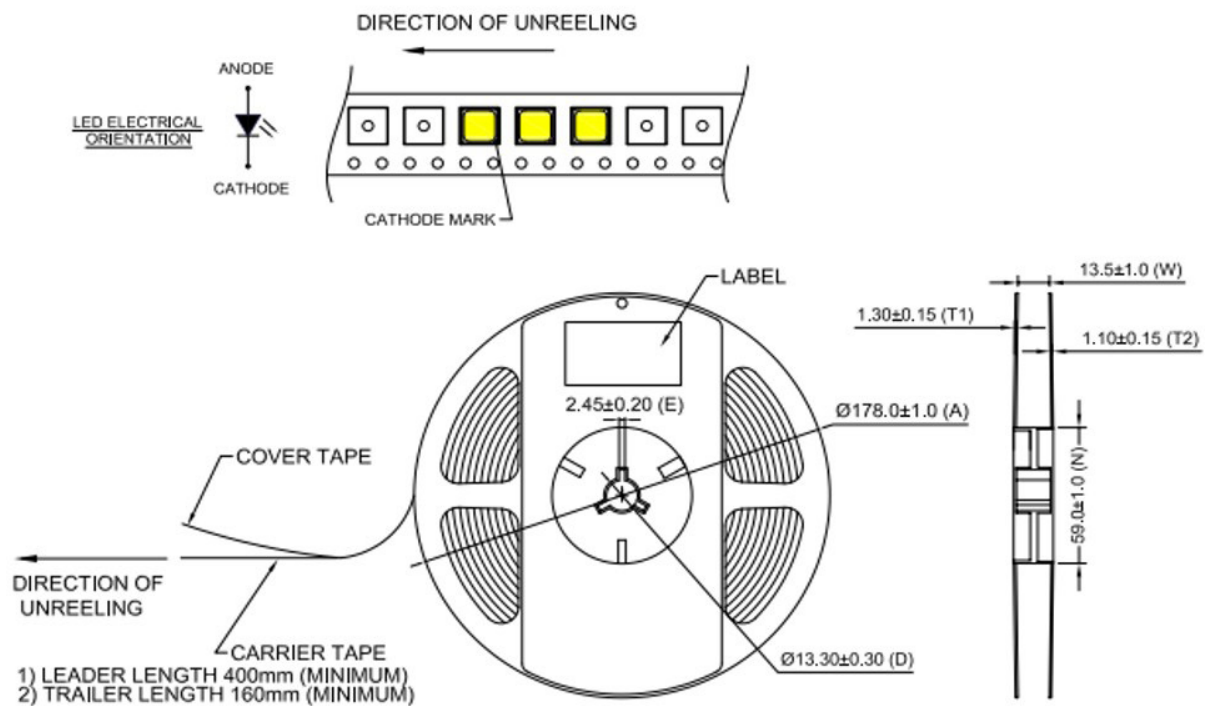
Figure 12d. Reel dimensions for LUXEON 5050 HE and LUXEON 5050 HE Plus
