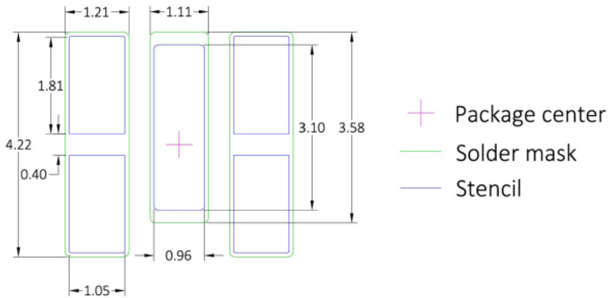
Figure 10c. Recommended PCB solder pad layout for LUXEON 5050 HE Plus - EH0
