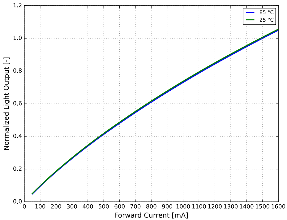
Figure 3b. Typical normalized light output vs. forward current for LUXEON Altilon Intense Gen2 1x2, MP, 25 °C and T_c = 85\text{ °C}
