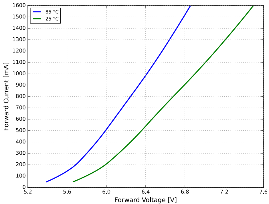
Figure 4a. Typical forward current vs. forward voltage for LUXEON Altilon Intense Gen2 1x2, MP, 25 °C and T_c = 85\text{ °C}
