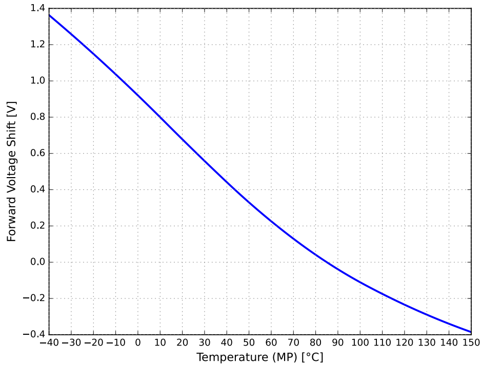
Figure 4b. Typical forward voltage vs. case temperature for LUXEON Altilon Intense Gen2 1x2, 1500 mA MP
