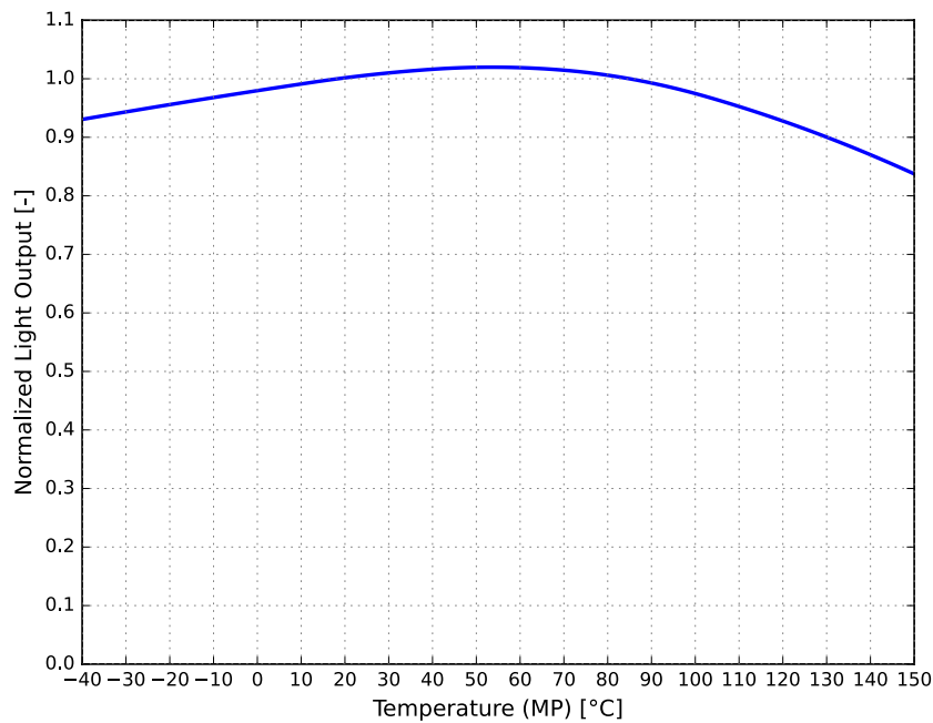
Figure 3a. Typical normalized light output vs. case temperature for LUXEON Altilon Intense Gen2 1x2, 1500 mA MP
