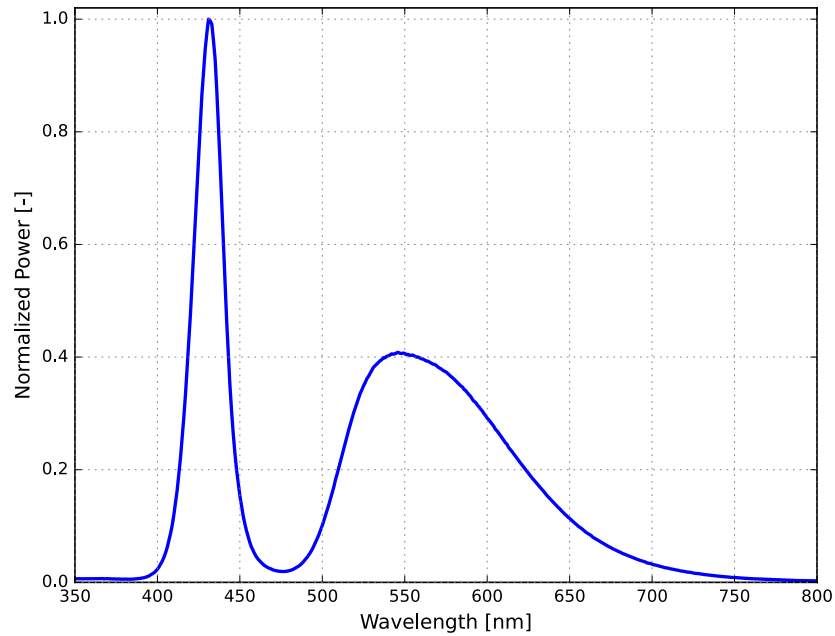
Figure 2. Typical normalized power vs. wavelength for LUXEON Altilon Intense Gen2 1x2, 1500 mA MP, T_c = 85^\circ\text{C}
