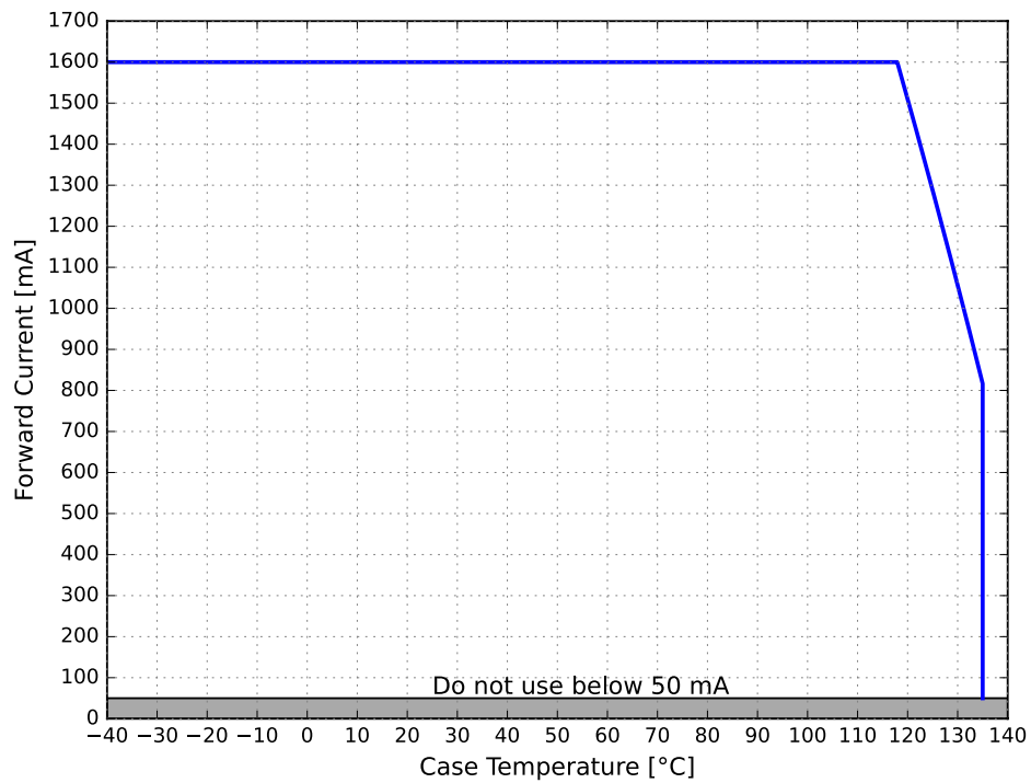
Figure 7. Maximum forward current vs. case temperature for LUXEON Altilon Intense Gen 2 1x2
