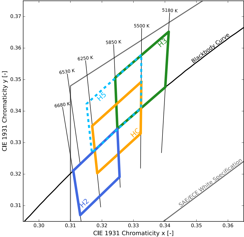
Figure 9. Color bin structure in CIE 1931 color space for LUXEON Altilon Intense Gen2 1x2 at 1500 mA, 20 ms MP, T_c = 85\text{ }^\circ\text{C}
