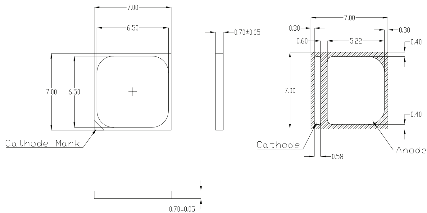
Figure 8. Mechanical dimensions for LUXEON 7070 and LUXEON 7070 HE
