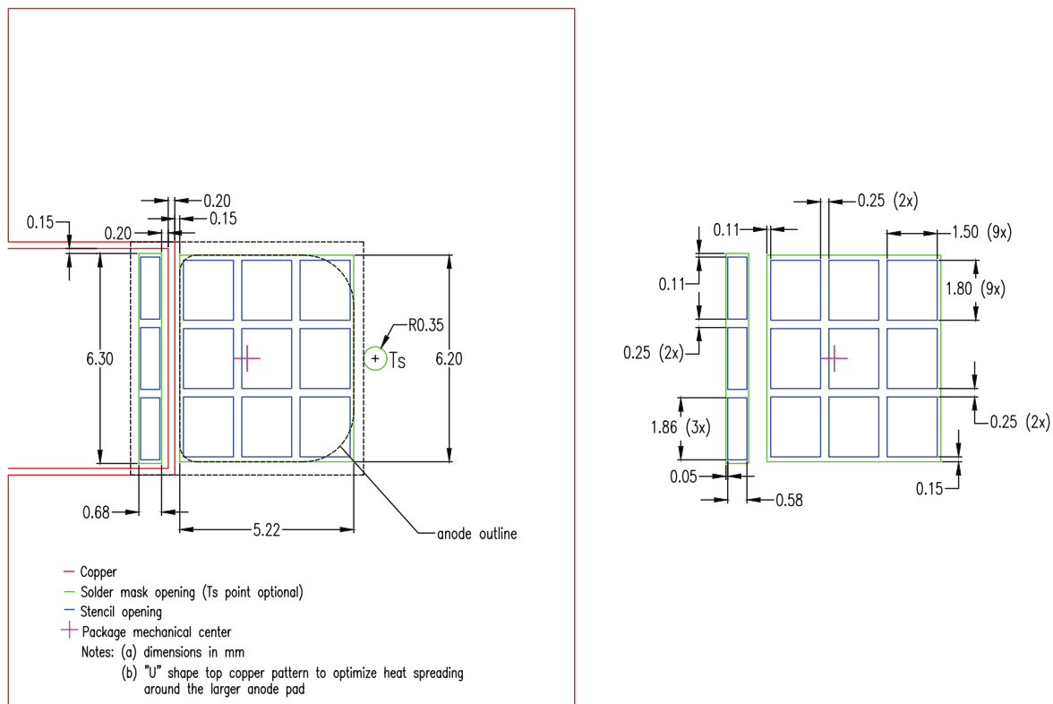
Figure 10. Recommended PCB solder pad layout for LUXEON 7070 and LUXEON 7070 HE
