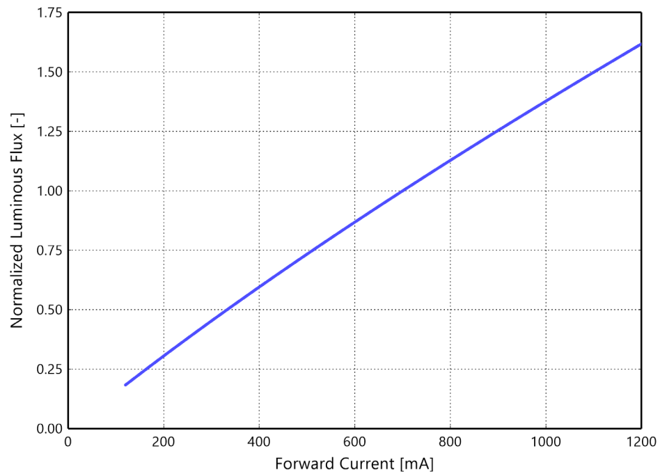
Figure 3c. Typical normalized light output vs. forward current for L170-xxxx7012000A1, T_j=25^{\circ}\text{C}
