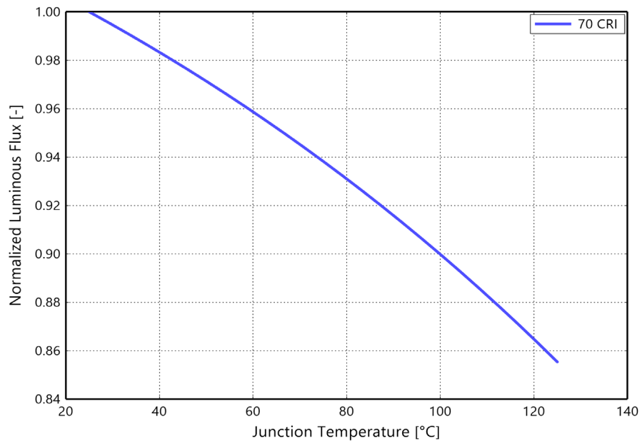
Figure 2b. Typical normalized light output vs. junction temperature for L170-xxx70xx000A1 at test current
