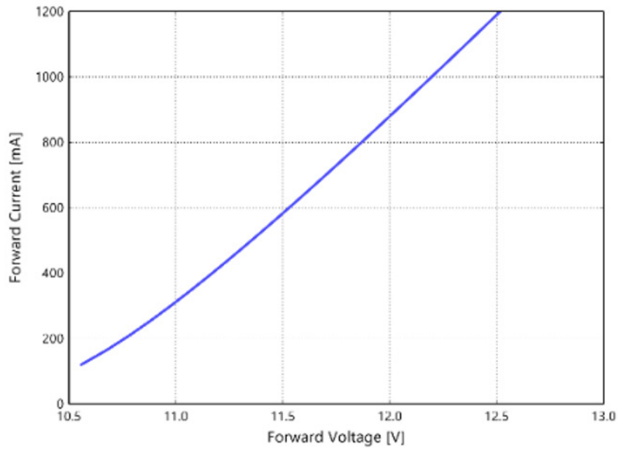
Figure 4c. Typical forward current vs forward voltage for L170-xxxx7012000A1, T_j=25^{\circ}\text{C}
