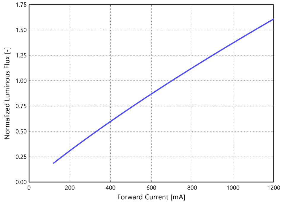
Figure 3a. Typical normalized light output vs. forward current for L170-xx70701200000, T_j=25^{\circ}\text{C}
