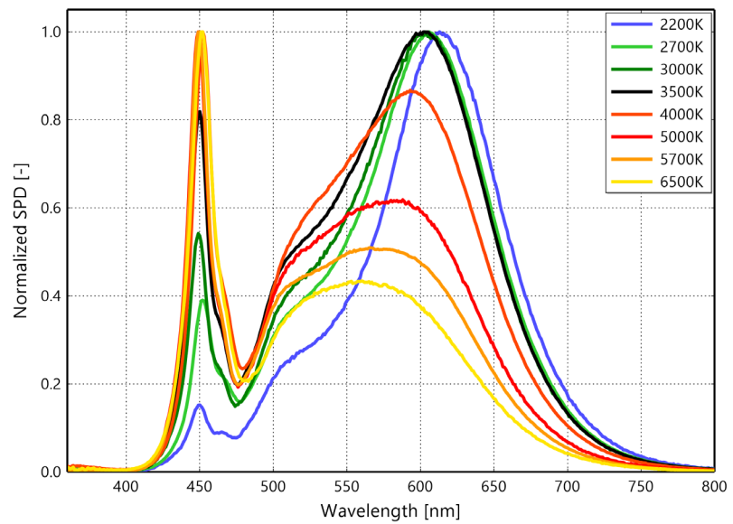
Figure 1b. Typical normalized power vs. wavelength for L170-xx807012000xx at test current, T_j = 25^\circ\text{C}
