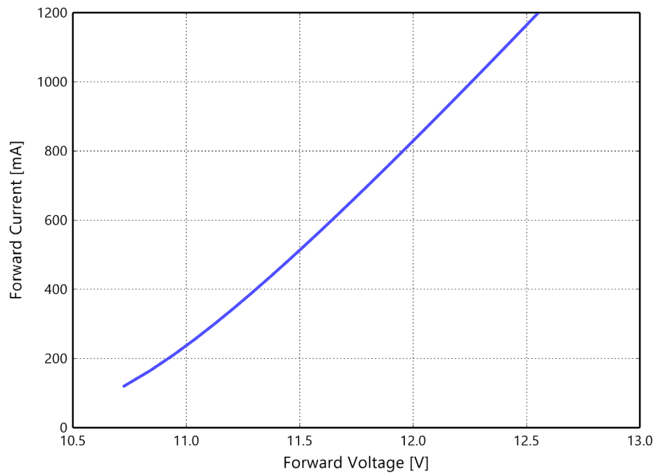
Figure 4a. Typical forward current vs. forward voltage for L170-xxxx701200000, T_j = 25^\circ\text{C}
