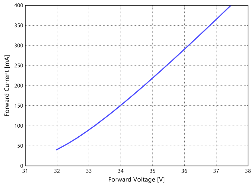
Figure 4b. Typical forward current vs forward voltage for L170-xxxx703600000, T_j=25^{\circ}\text{C}
