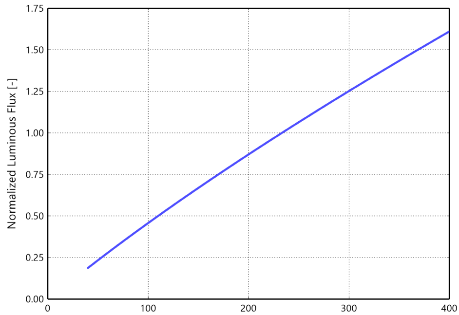
Figure 3b. Typical normalized light output vs. forward current for L170-xxxx703600000, T_j=25^{\circ}\text{C}
