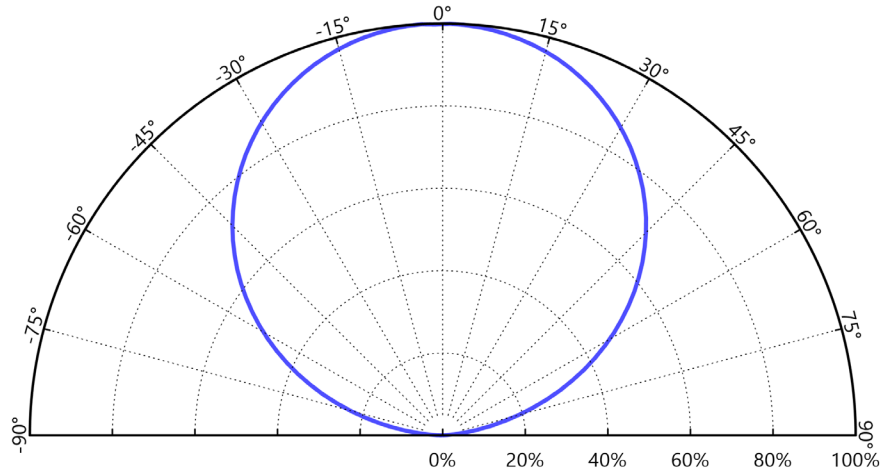
Figure 6b. Typical polar radiation pattern for L170-xxxx70xxx00A1 at test current, T_j=25^\circ\text{C}
