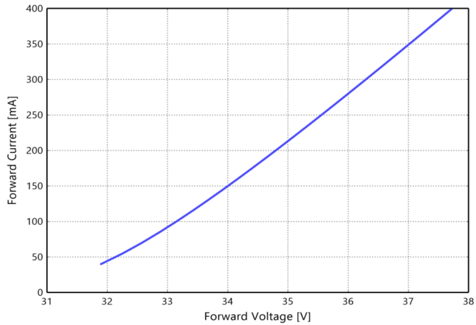
Figure 4d. Typical forward current vs forward voltage for L170-xxxx7036000A1, T_j=25^{\circ}\text{C}
