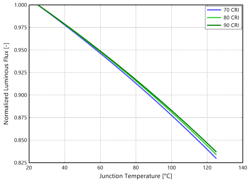
Figure 2a. Typical normalized light output vs. junction temperature for L170-xxxx70xx00000 at test current
