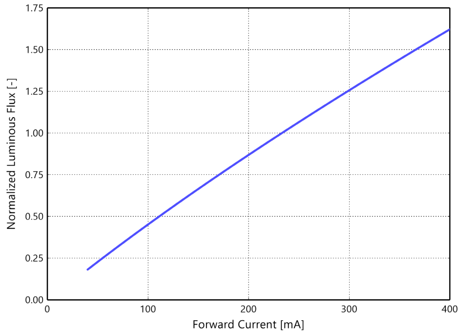
Figure 3d. Typical normalized light output vs. forward current for L170-xxxx7036000A1, T_j = 25^\circ\text{C}
