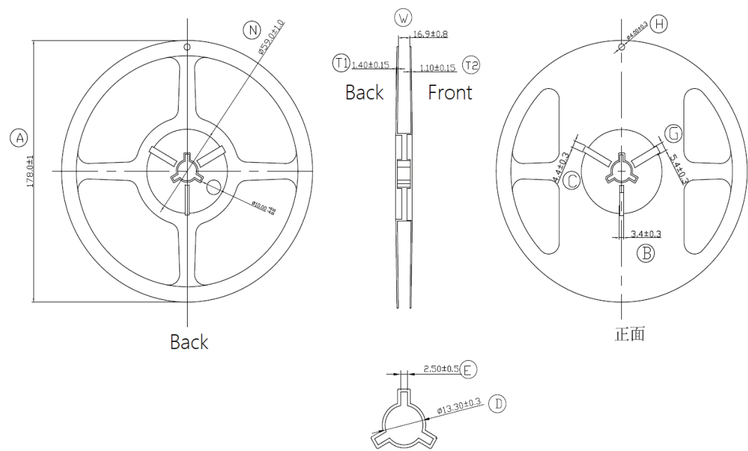
Figure 12. Reel dimensions for LUXEON 7070 and LUXEON 7070 HE
