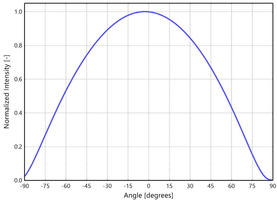
Figure 5a. Typical radiation pattern for L170-xxxx70xxx0000 at test current, T_j=25^{\circ}\text{C}
