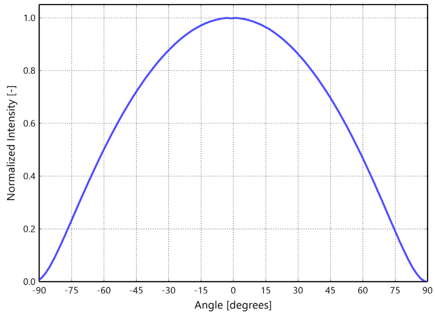
Figure 5b. Typical radiation pattern for L170-xxxx70xxx00A1 at test current, T_j=25^{\circ}\text{C}
