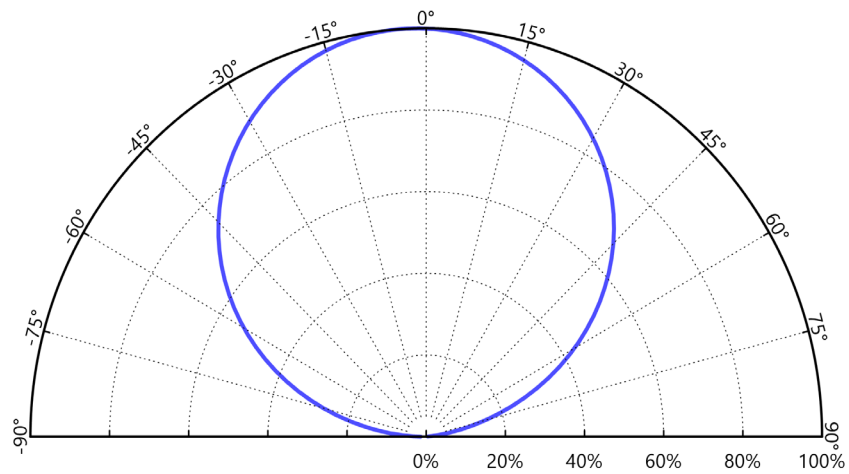
Figure 6a. Typical polar radiation pattern for L170-xxxx70xxx0000 at test current, T_j=25^{\circ}\text{C}
