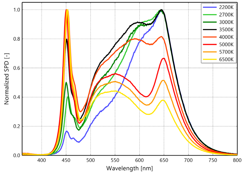
Figure 1c. Typical normalized power vs. wavelength for L170-xx907012000xx at test current, T_j=25^{\circ}\text{C}
