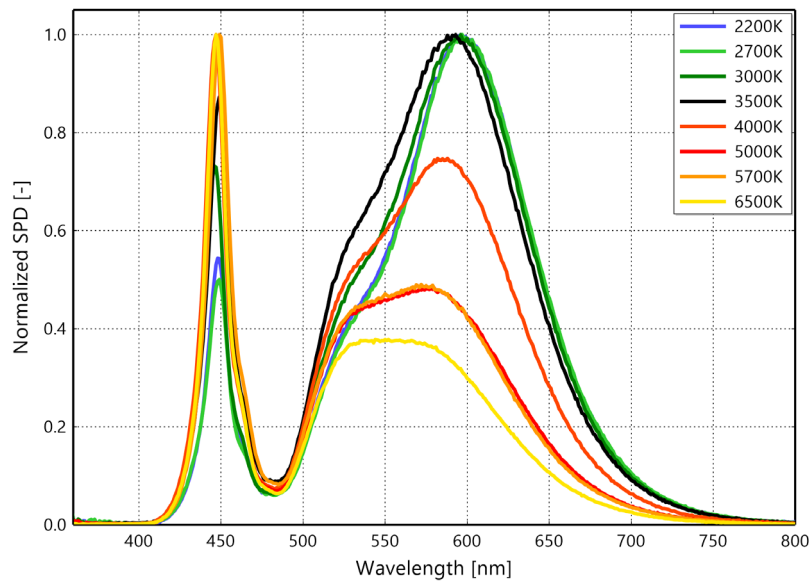
Figure 1a. Typical normalized power vs. wavelength for L170-xx707012000xx at test current, T_j = 25^\circ\text{C}
