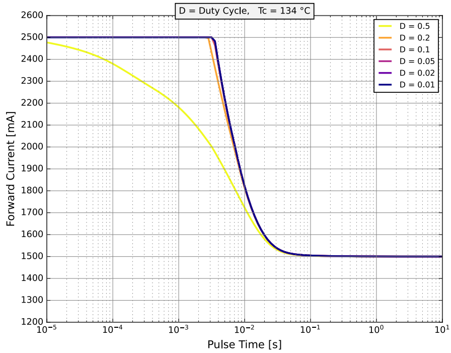
Figure 12a. Pulse handling capability for LUXEON FX2-L Plus Cool-White at highest case temperature, where maximum DC current can be applied
