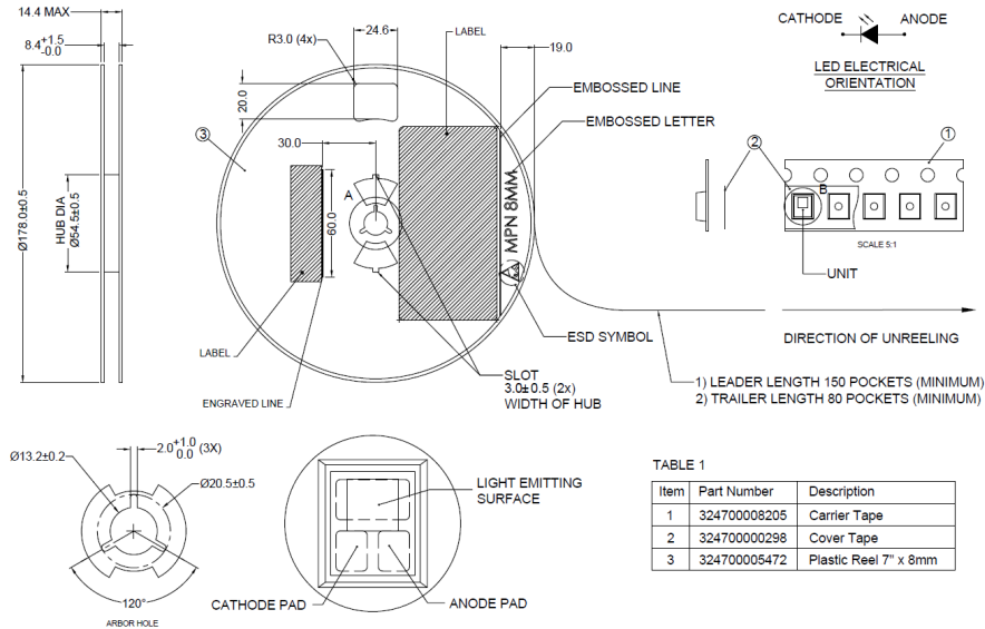
Figure 16. Reel dimensions for LUXEON FX2-L Plus Cool-White
