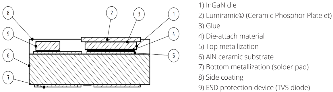
Figure 1. Schematic cross section LUXEON FX2-L Plus Cool-White
