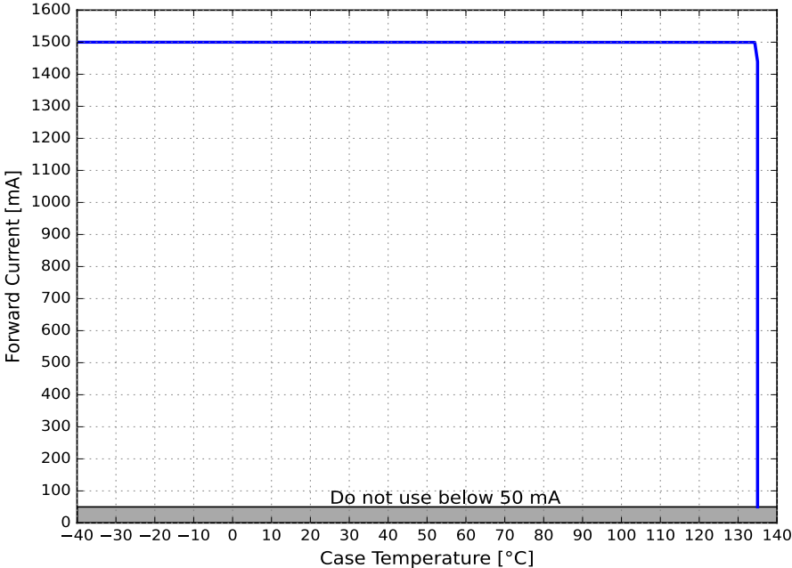
Figure 11. Maximum forward current vs. case temperature for LUXEON FX2-L Plus Cool-White
