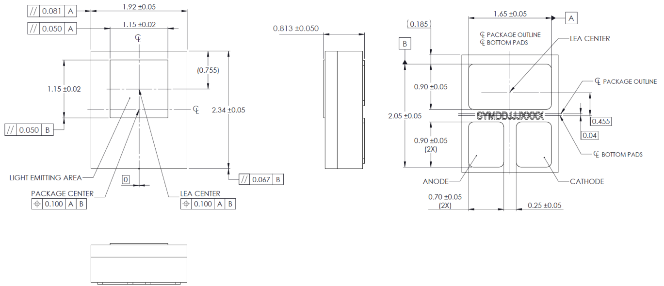
Figure 14: Mechanical Dimensions for LUXEON FX2-L Plus Cool-White
