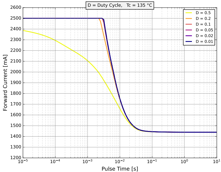
Figure 12b. Pulse handling capability for LUXEON FX2-L Plus Cool-White at maximum case temperature
