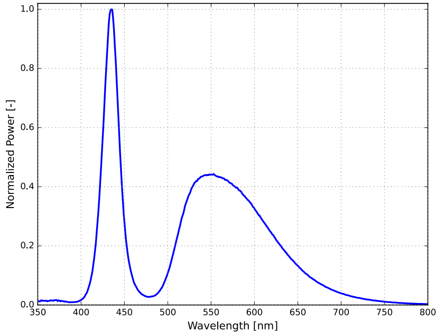
Figure 2. Typical normalized power vs. wavelength for LUXEON FX2-L Plus Cool-White at MP binning conditions
