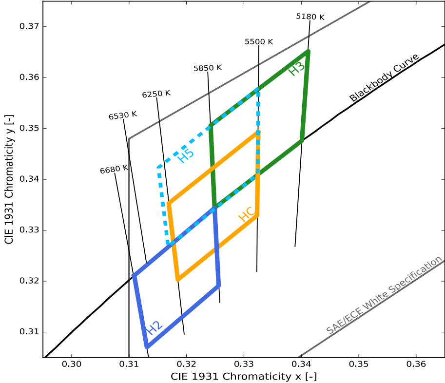
Figure 13. Color bin structure for LUXEON FX2-L Plus Cool-White
