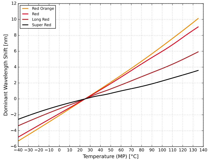
Figure 1b. Typical wavelength shift vs junction temperature for SignalSure 250 at 20 ms MP, 250 mA, T_j = 25\text{ }^\circ\text{C}
