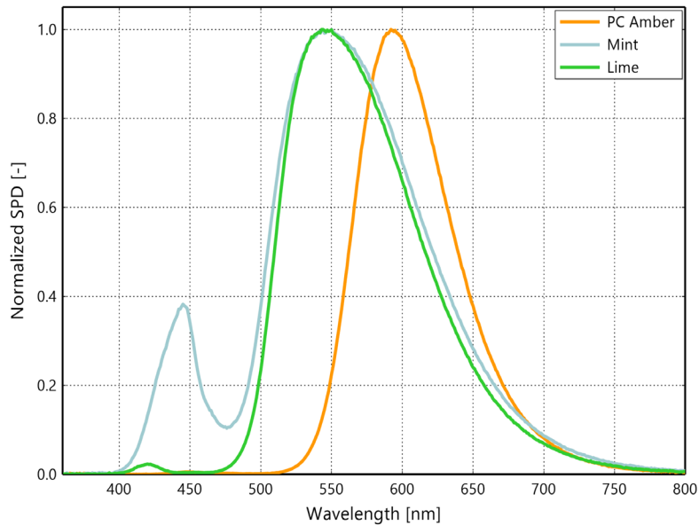
Figure 1b. Typical normalized SPD vs. wavelength for LUXEON C ES Phosphor Converted Colors at 1000mA, T_j=85^\circ\text{C}
