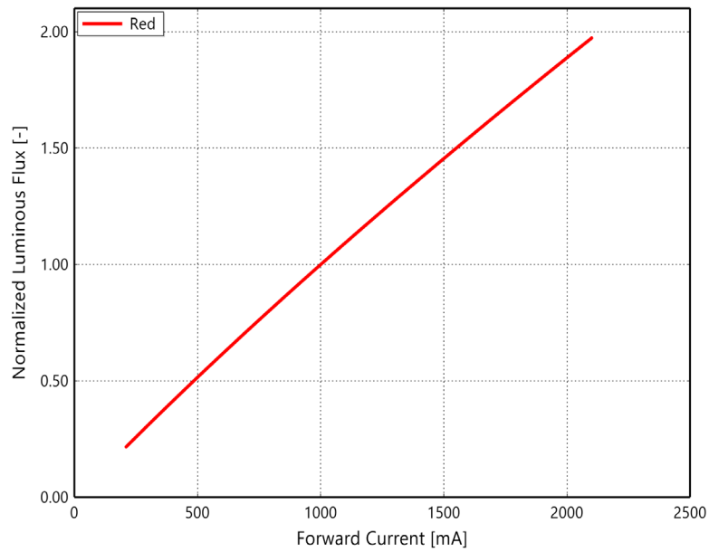
Figure 3b. Typical normalized luminous flux vs. forward current for LUXEON C ES Red at T_j=85^\circ\text{C}
