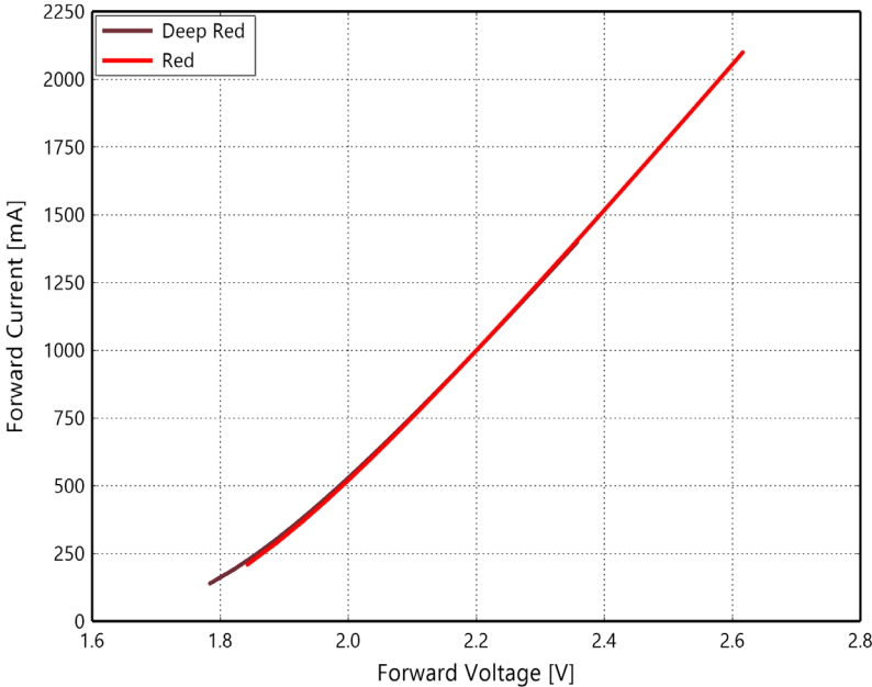
Figure 4a. Typical forward current vs. forward voltage for LUXEON C ES Deep Red and Red at T_j=85^\circ\text{C}
