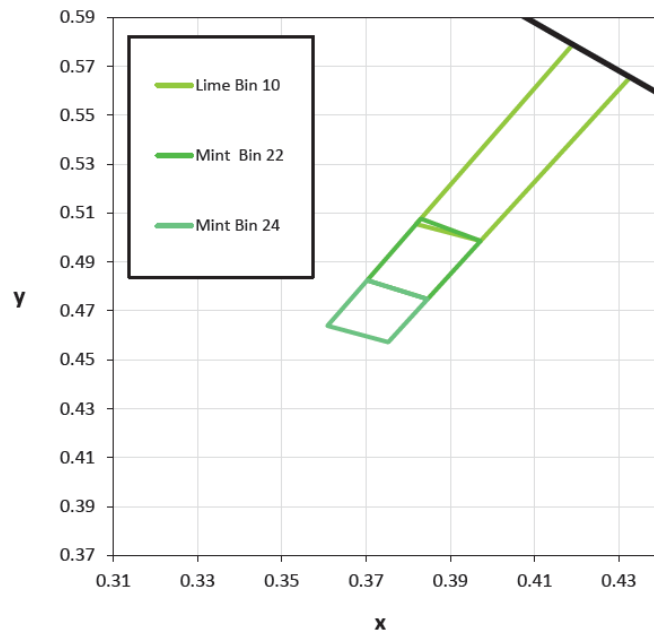
Figure 8. Color bin structure for LUXEON C ES Mint and Lime for Table 7
