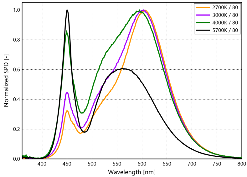
Figure 1d. Typical normalized SPD vs. wavelength for LUXEON C ES White 80CRI at 1000mA, T_j=85^\circ\text{C}
