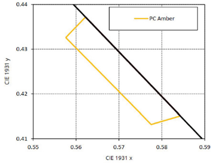
Figure 7. Color bin structure for LUXEON C ES PC Amber for Table 7
