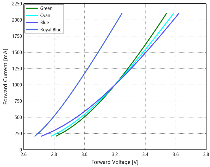
Figure 4c. Typical forward current vs. forward voltage for LUXEON C ES Green, Cyan, Blue and Royal Blue at T_j=85^\circ\text{C}
