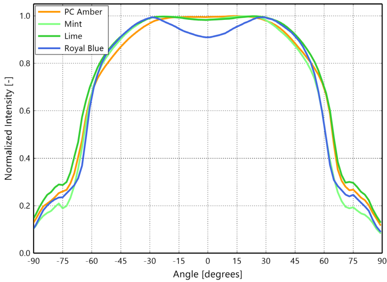
Figure 5b. Typical radiation pattern for LUXEON C ES PC Amber, Mint, Lime and Royal Blue at 1000mA, T_j=85^{\circ}\text{C}
