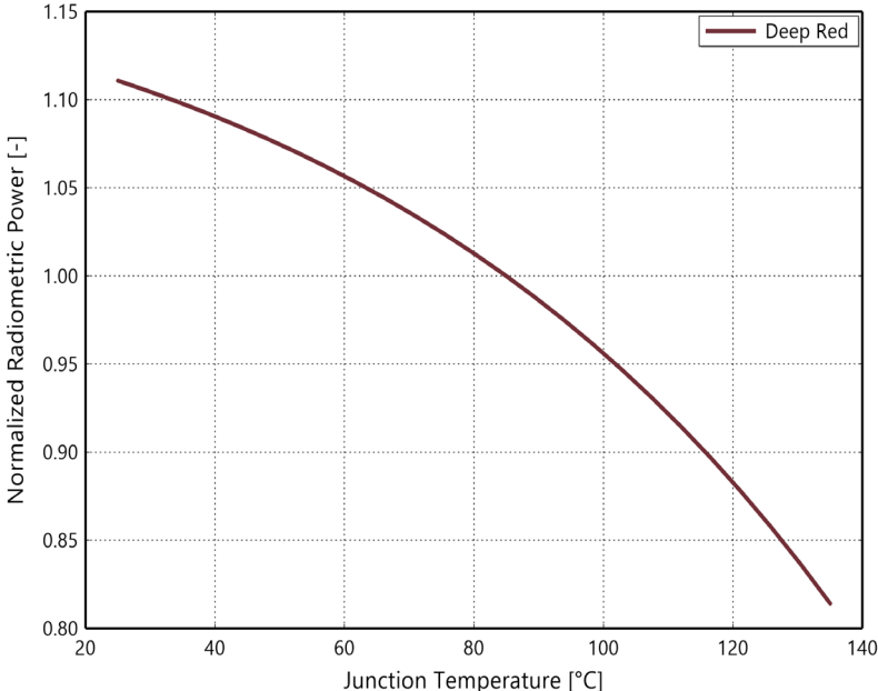
Figure 2a. Typical normalized radiometric power vs. junction temperature for LUXEON C ES Deep Red at 1000mA
