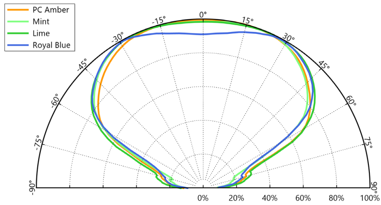
Figure 6b. Typical polar radiation pattern for LUXEON C ES PC Amber, Mint, Lime and Royal Blue at 1000mA, T_j=85^\circ\text{C}
