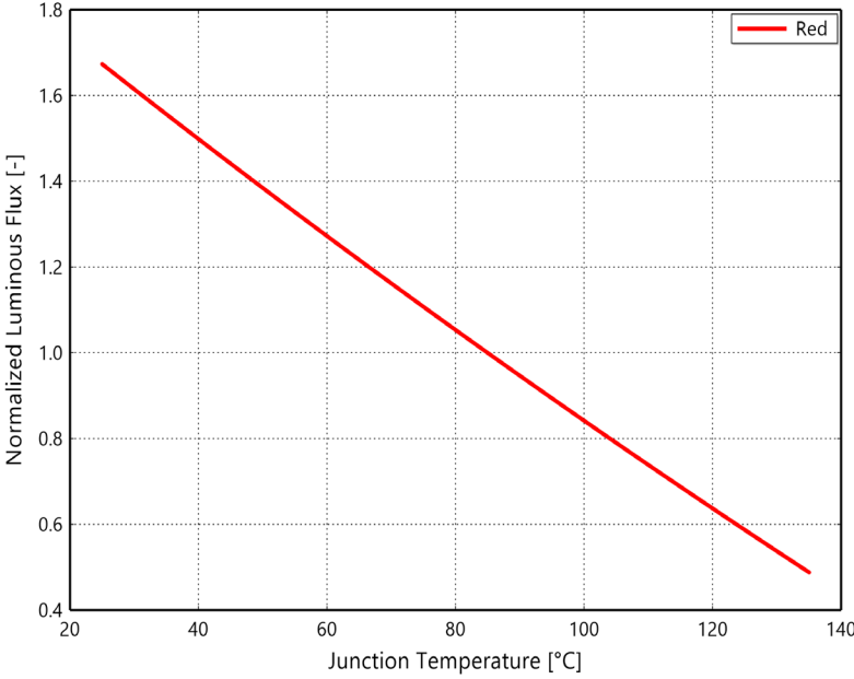
Figure 2b. Typical normalized luminous flux vs. junction temperature for LUXEON C ES Red at 1000mA
