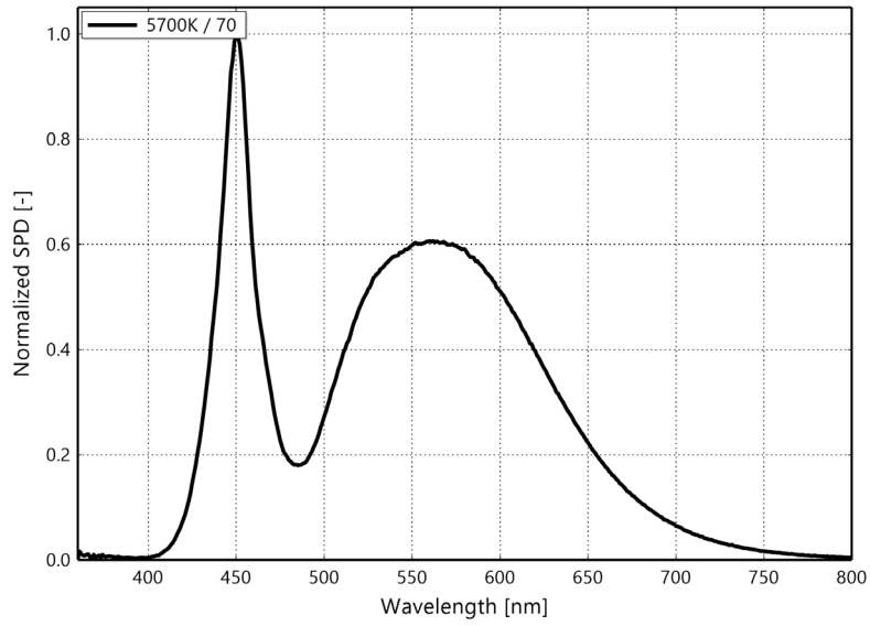
Figure 1c. Typical normalized SPD vs. wavelength for LUXEON C ES White 70CRI at 1000mA, T_j=85^\circ\text{C}
