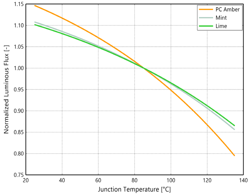
Figure 2c. Typical normalized luminous flux vs. junction temperature for LUXEON C ES PC Amber, Mint and Lime at 1000mA
