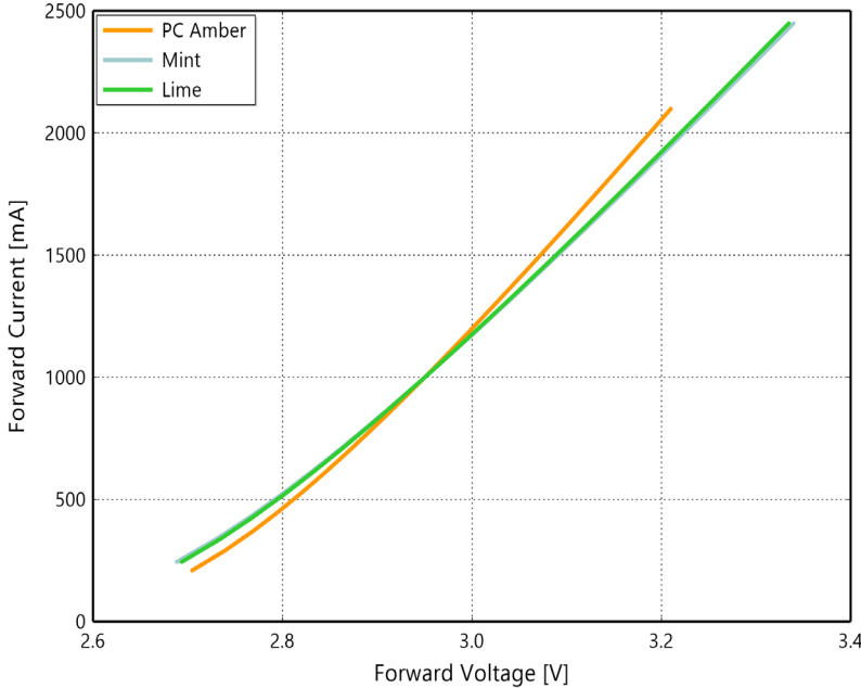
Figure 4b. Typical forward current vs. forward voltage for LUXEON C ES PC Amber, Mint and Lime at T_j=85^\circ\text{C}
