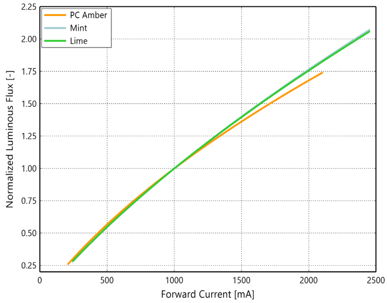
Figure 3c. Typical normalized luminous flux vs. forward current for LUXEON C ES PC Amber, Mint and Lime at T_j=85^\circ\text{C}
