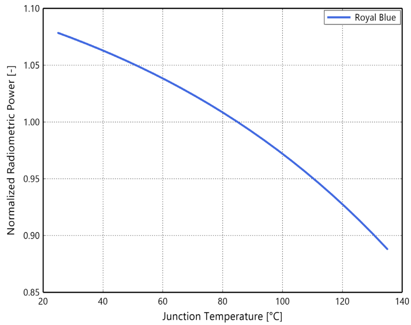
Figure 2e. Typical normalized radiometric power vs. junction temperature for LUXEON C ES Royal Blue at 1000mA
