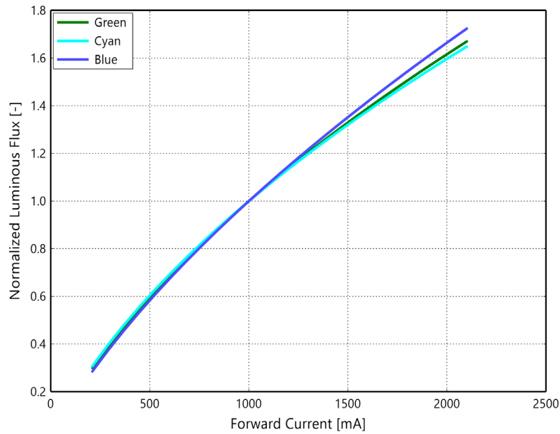
Figure 3d. Typical normalized luminous flux vs. forward current for LUXEON C ES Green, Cyan and Blue at T_j=85^\circ\text{C}
