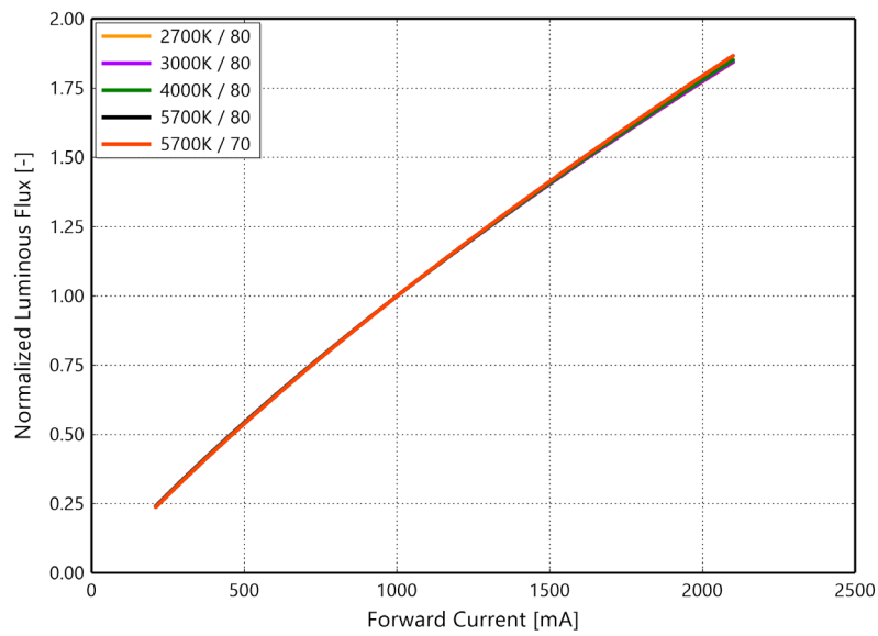
Figure 3f. Typical normalized luminous flux vs. forward current for LUXEON C ES White at T_j=85^\circ\text{C}
