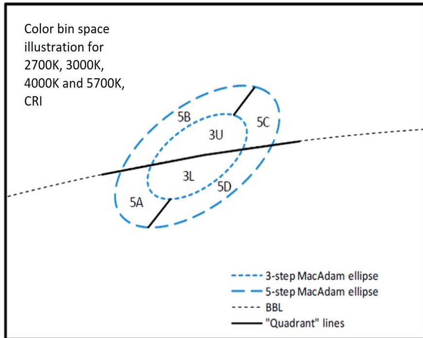
Figure 9. Color bin structure for LUXEON C ES Color Line
