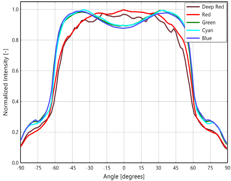
Figure 5a. Typical radiation pattern for LUXEON C ES Deep Red, Red, Green, Cyan and Blue at 1000mA, T_j=85^{\circ}\text{C}
