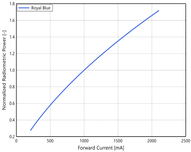
Figure 3e. Typical normalized radiometric power vs. forward current for LUXEON C ES Royal Blue at T_j=85^\circ\text{C}
