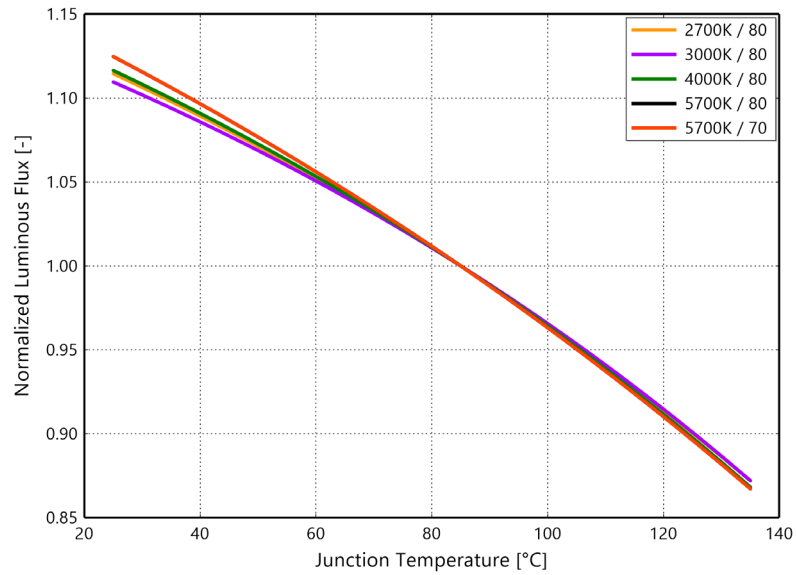
Figure 2f. Typical normalized luminous flux vs. junction temperature for LUXEON C ES White at 1000mA
