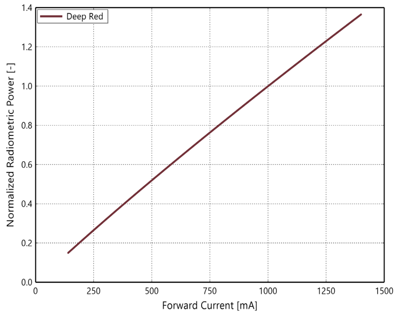
Figure 3a. Typical normalized radiometric power vs. forward current for LUXEON C ES Deep Red at T_j=85^\circ\text{C}
