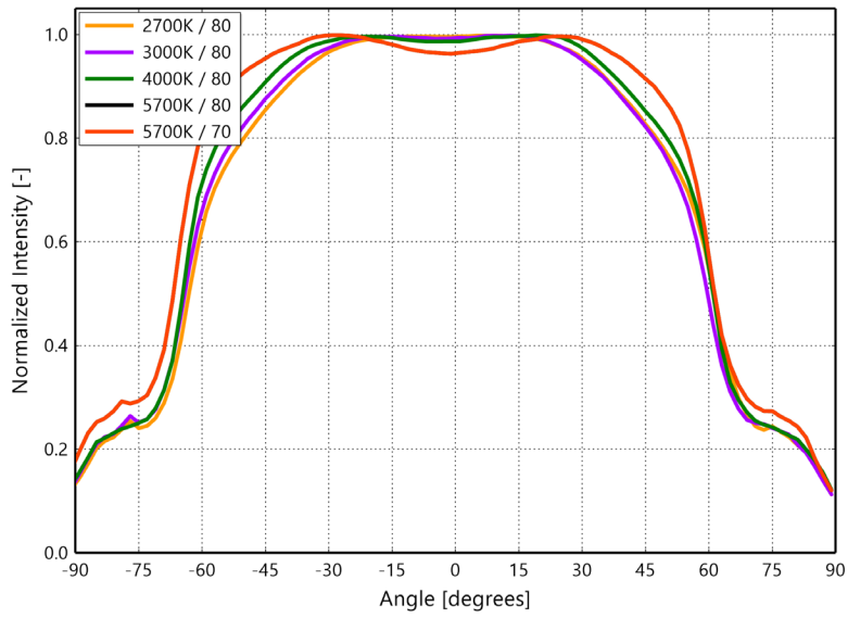
Figure 5c. Typical radiation pattern for LUXEON C ES White at 1000mA, T_j=85^\circ\text{C}
