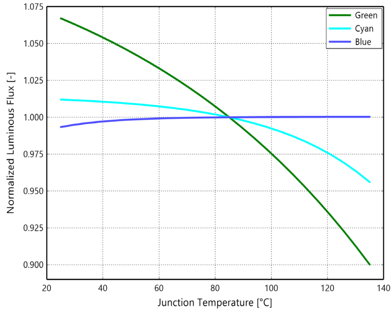
Figure 2d. Typical normalized luminous flux vs. junction temperature for LUXEON C ES Green, Cyan and Blue at 1000mA
