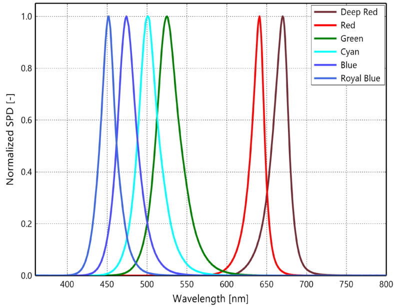
Figure 1a. Typical normalized SPD vs. wavelength for LUXEON C ES Direct Colors at 1000mA, T_j=85^\circ\text{C}
