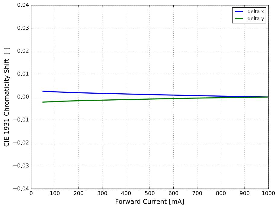
Figure 8. Typical color shift in CIE 1931 x, y coordinates vs. forward current for LUXEON FX2-L Plus PC-Amber at MP binning temperature
