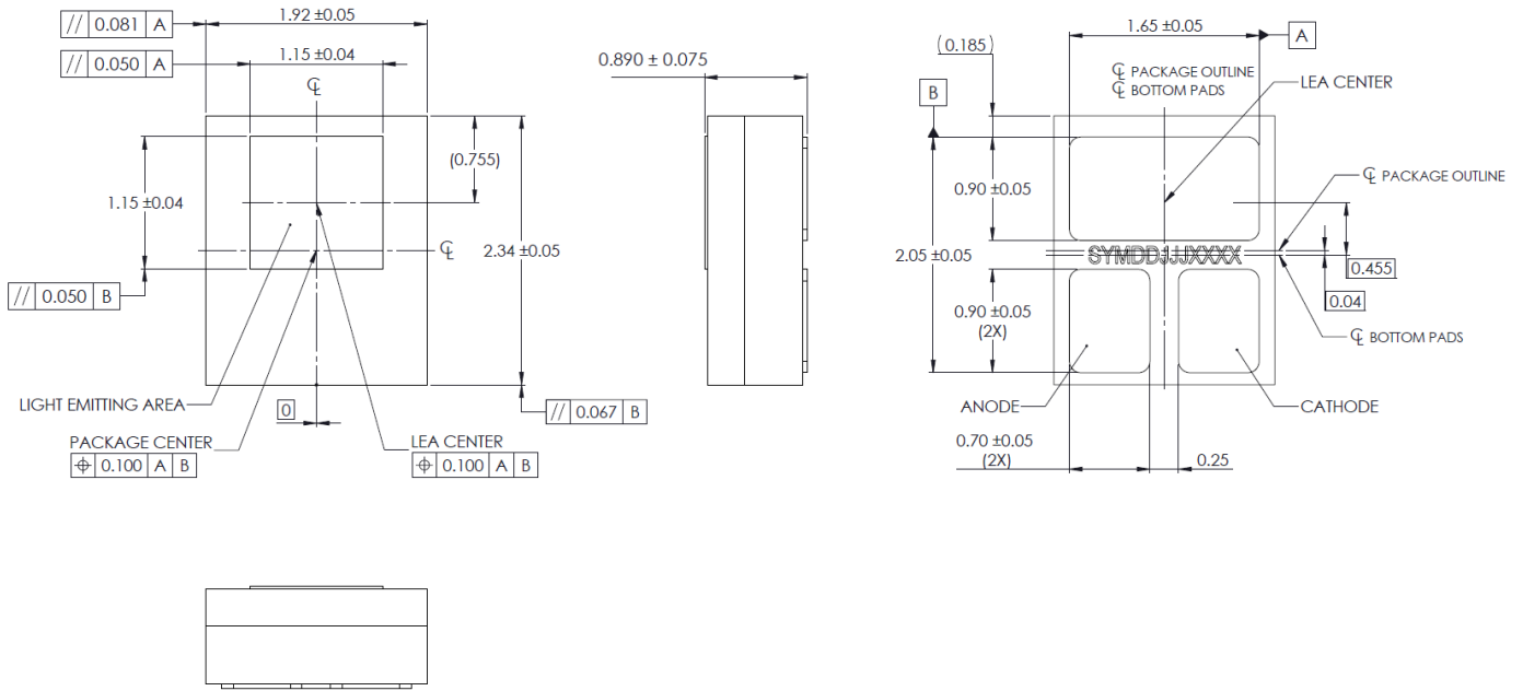
Figure 14. Mechanical dimensions for LUXEON FX2-L Plus PC-Amber
