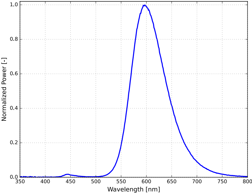
Figure 2. Typical normalized power vs. wavelength for LUXEON FX2-L Plus PC-Amber at MP binning conditions
