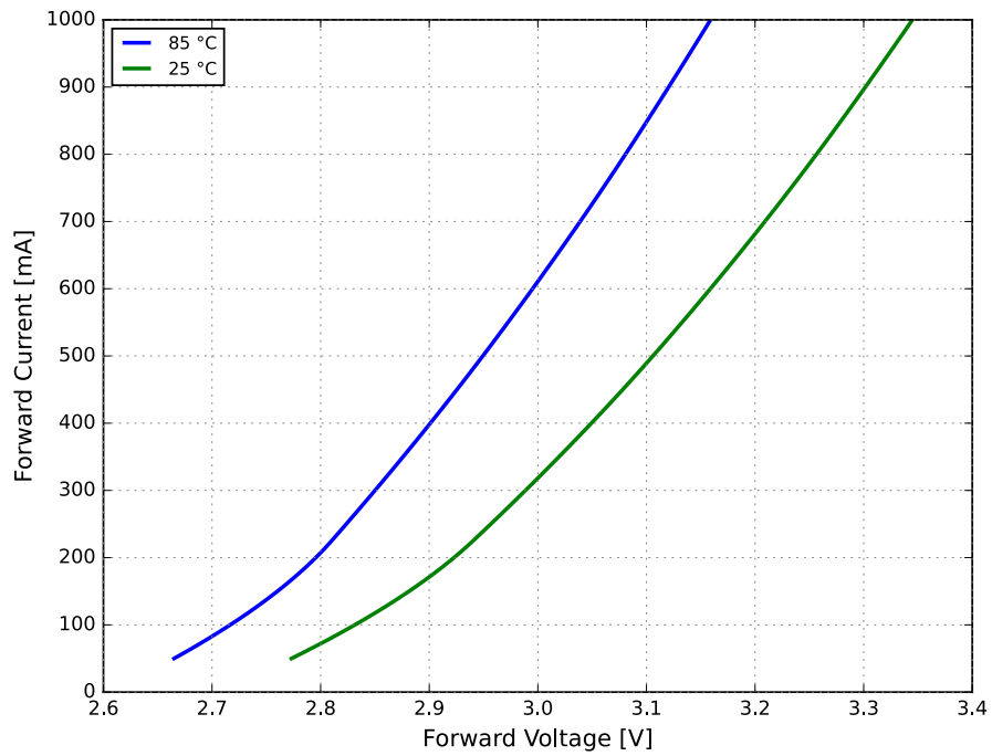
Figure 5. Typical forward current vs. forward voltage for LUXEON FX2-L Plus PC-Amber at MP binning temperature and at room temperature
