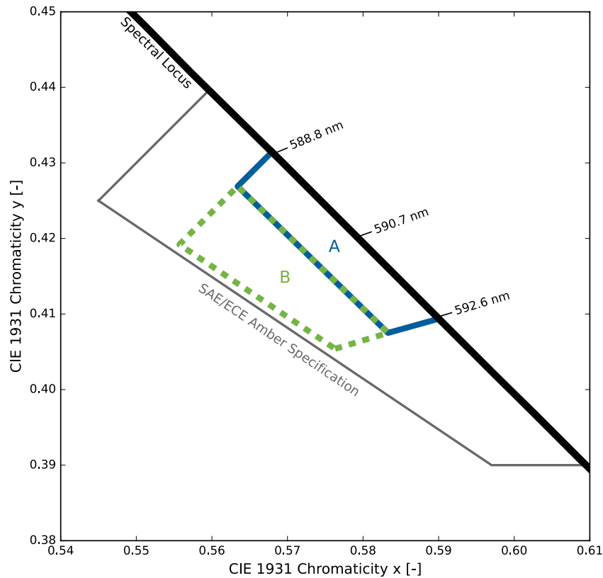
Figure 13. Color bin structure for LUXEON FX2-L Plus PC-Amber
