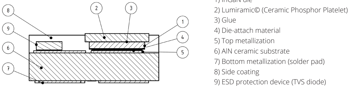
Figure 1. Schematic cross section LUXEON FX2L Plus PC-Amber
