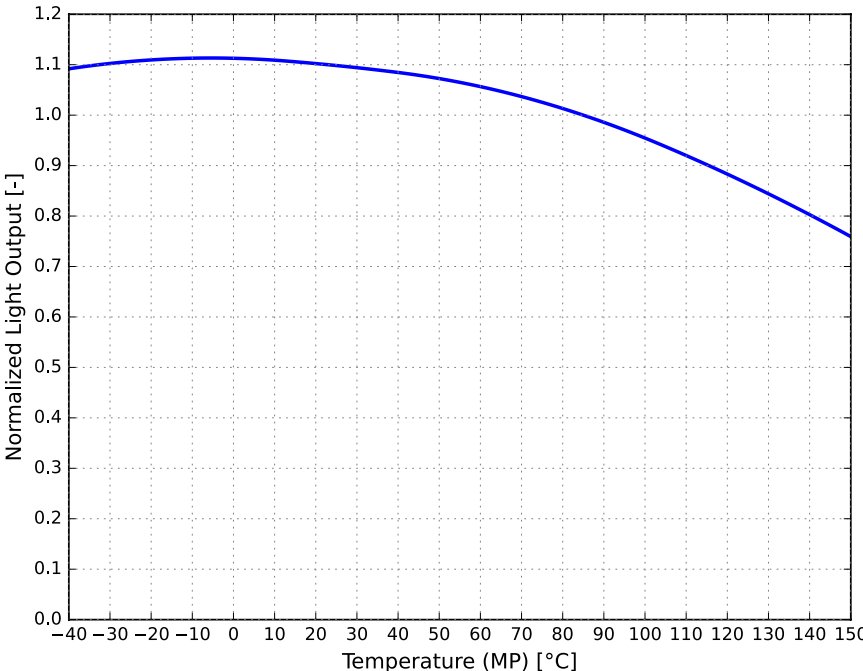
Figure 3. Typical normalized light output vs. temperature for LUXEON FX2-L Plus PC-Amber at MP binning current
