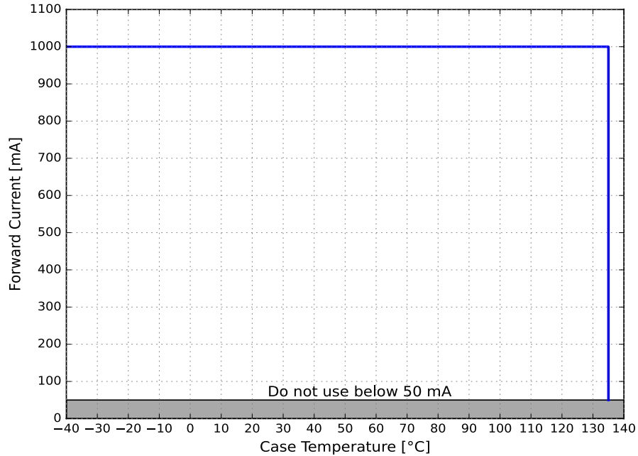
Figure 11. Maximum forward current vs. case temperature for LUXEON FX2-L Plus PC-Amber
