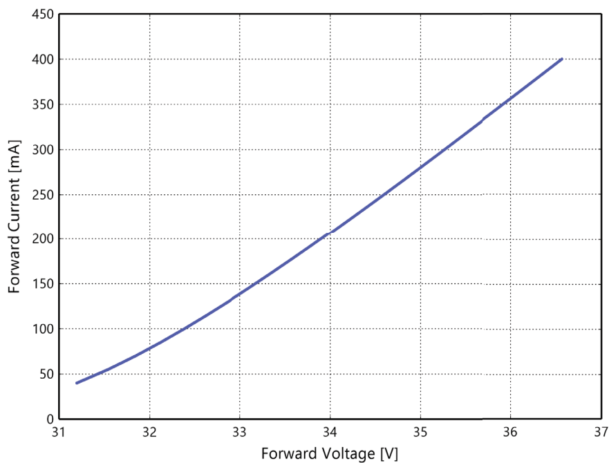
Figure 4b. Typical forward current vs. forward voltage for L2C5-xxxx1202x090x at T_j=85^{\circ}\text{C} .
