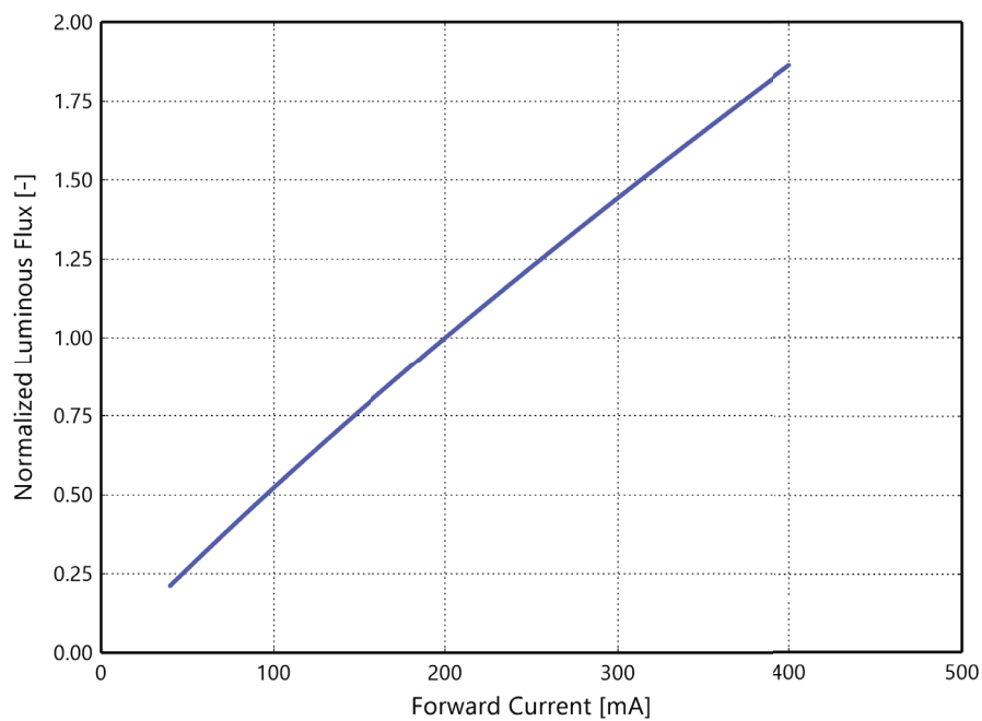
Figure 3a. Typical normalized light output vs. forward current for L2C5-xxxx1202x060x at Tj=85°C.
