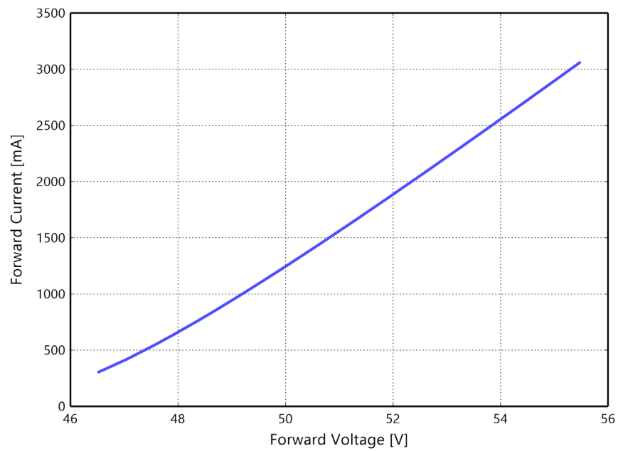
Figure 4l. Typical forward current vs. forward voltage for L2C5-xxxx1817xxx0x at T_j=85^{\circ}\text{C} .
