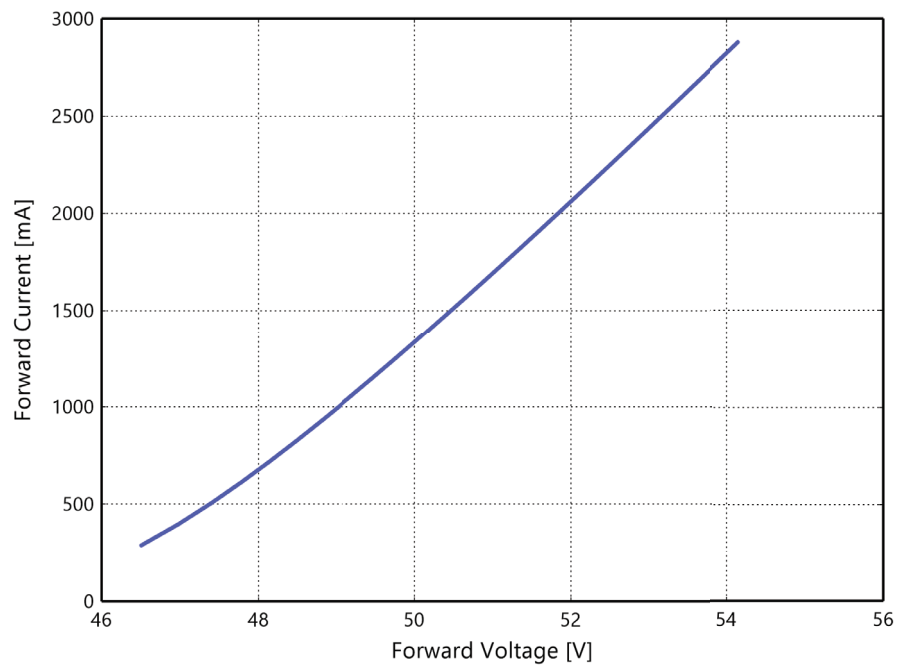
Figure 4k. Typical forward current vs. forward voltage for L2C5-xxxx1816xxx0x at T_j=85^{\circ}\text{C} .
