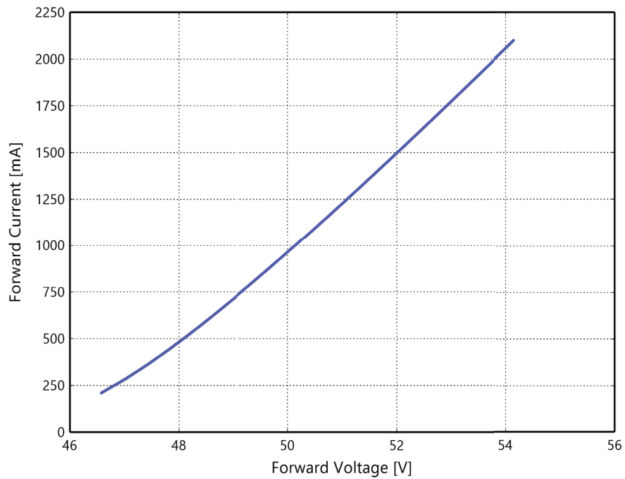
Figure 4j. Typical forward current vs. forward voltage for L2C5-xxxx1812xxx0x at T_j=85^{\circ}\text{C} .
