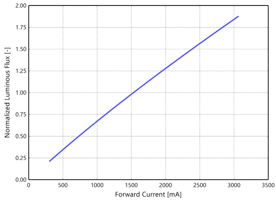
Figure 3l. Typical normalized light output vs. forward current for L2C5-xxxx1817xxx0x at T_j=85^{\circ}\text{C} .
