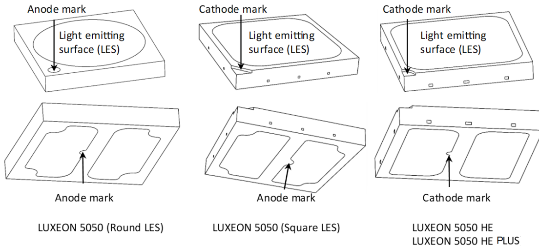
Figure 1. Package rendering of the LUXEON 5050 emitter.
