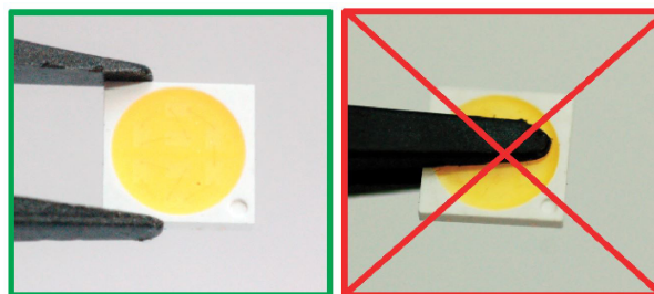
Figure 2. Correct tweezers handling of a representative LUXEON 5050 (left). Incorrect handling (right).
