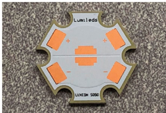
Figure 3b. An example of a LUXEON 5050 (Round LES) star board showing the LED electrode pad solder mask openings.
