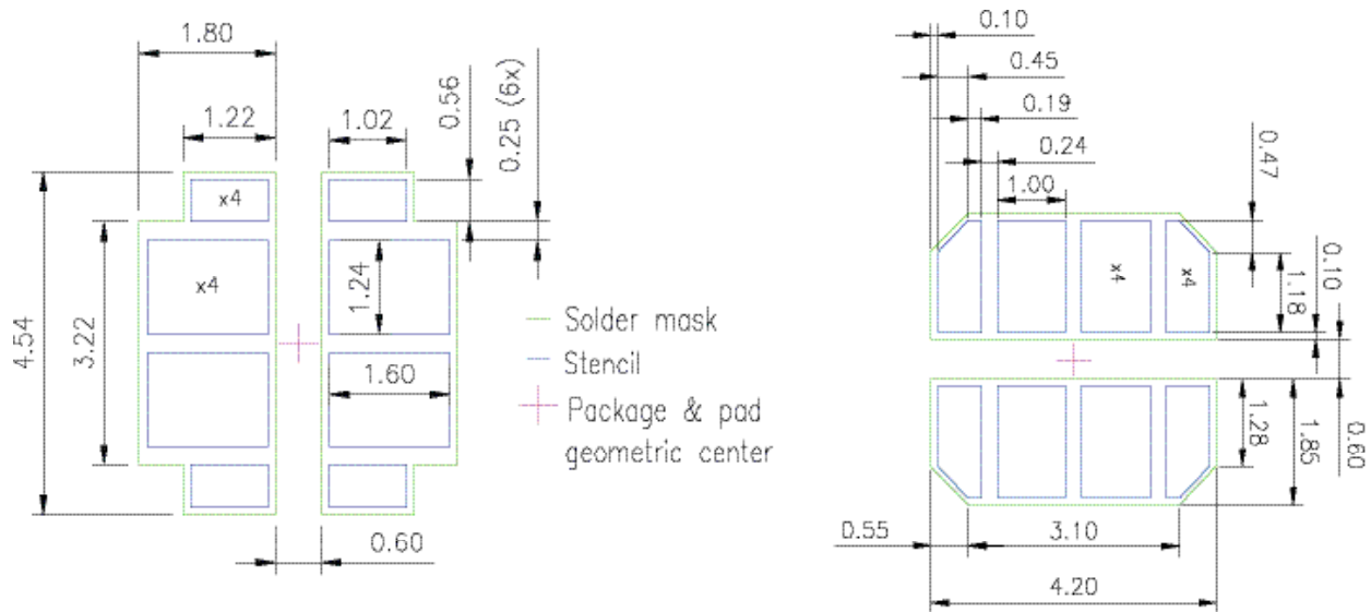
Figure 3a. Recommended PCB footprint showing solder mask and stencil opening for LUXEON 5050 (Round LES)/LUXEON 5050 HE, left, and LUXEON 5050 (Square LES), right. Dimensions are in mm.
