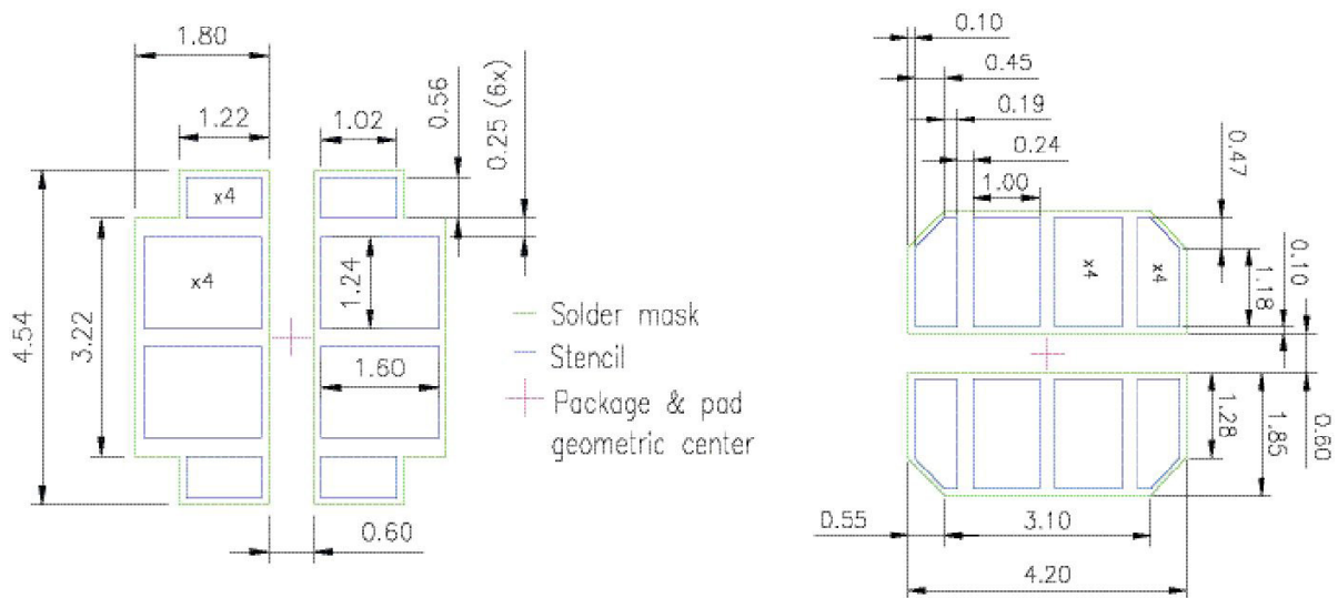
Figure 3a. Recommended PCB footprint showing solder mask and stencil opening for LUXEON 5050 (Round LES)/LUXEON 5050 (Square LES)/LUXEON 5050 HE /LUXEON 5050 HE Plus, left, and optimized design for LUXEON 5050 (Square LES), right. Dimensions are in mm.).
