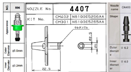
Figure 5. Examples of possible off-the-shelf nozzles.
