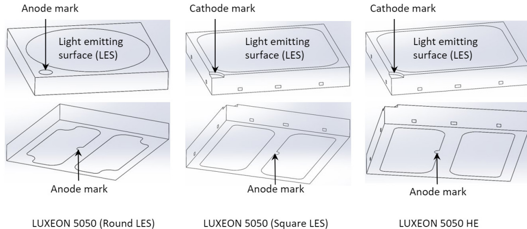
Figure 1. Package rendering of the LUXEON 5050 emitter.
