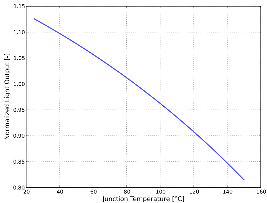
Figure 2. Typical normalized light output vs. junction temperature for LXZx-xxxx, at test current.
