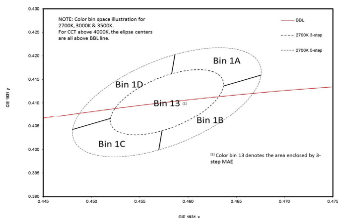
Figure 6. Color space definition for LUXEON Rebel PLUS.
