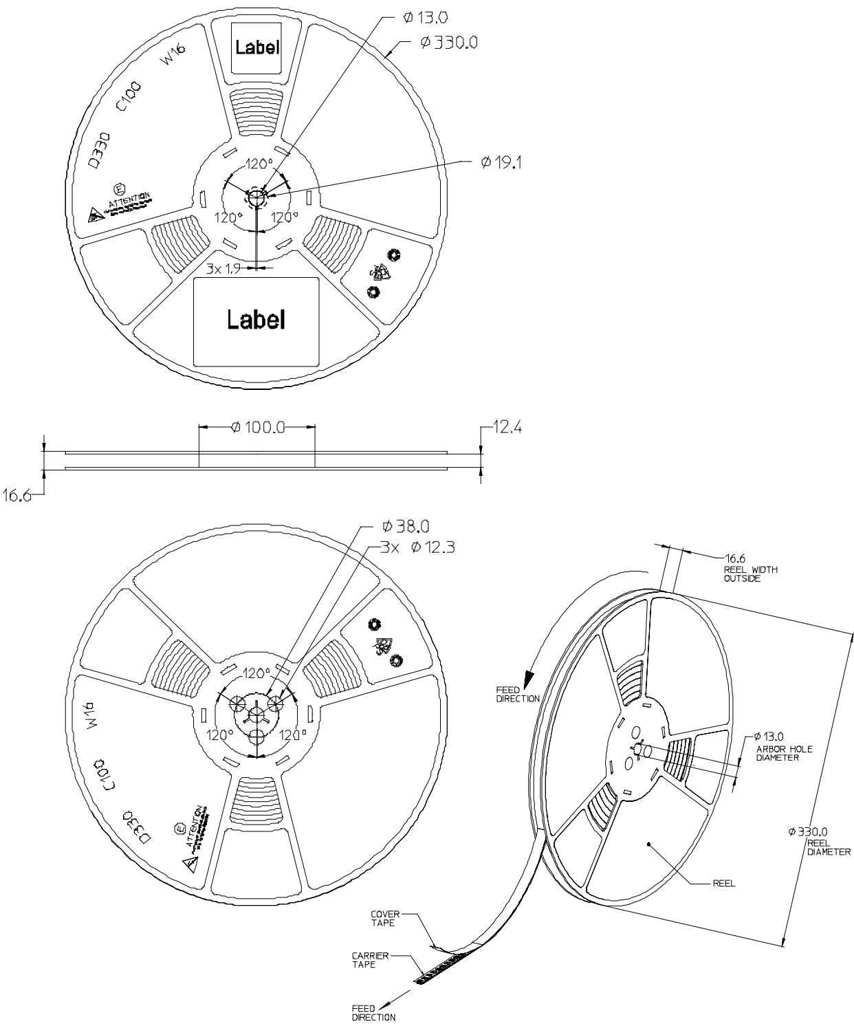
Figure 13. Reel dimensions for LUXEON Rebel PLUS.
