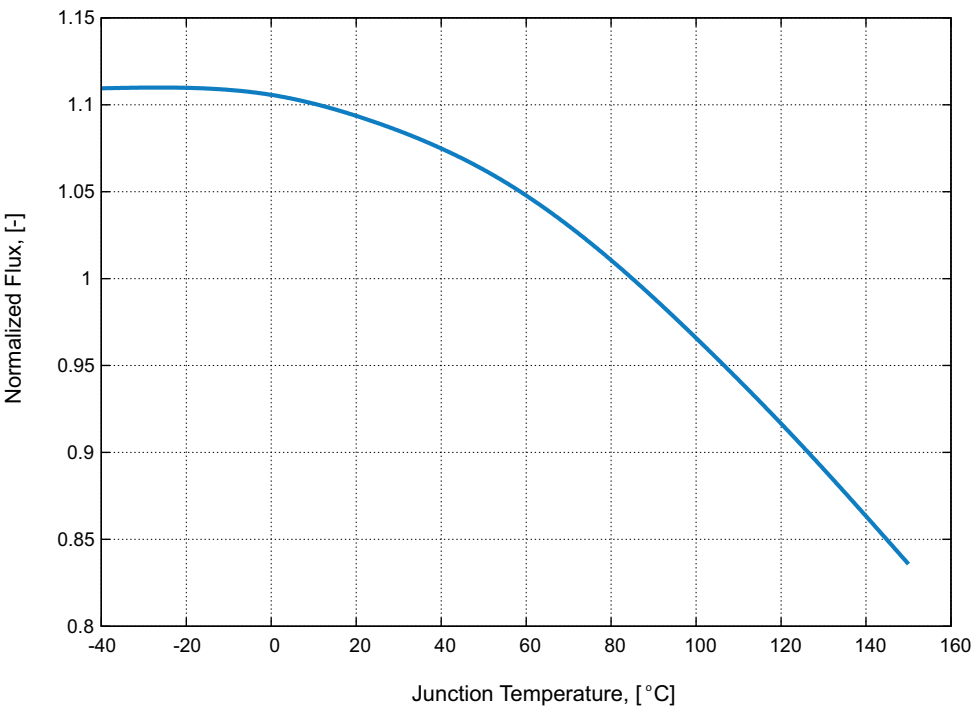
Figure 2. Typical normalized light output vs. junction temperature for LUXEON Rebel PLUS at 350mA.
