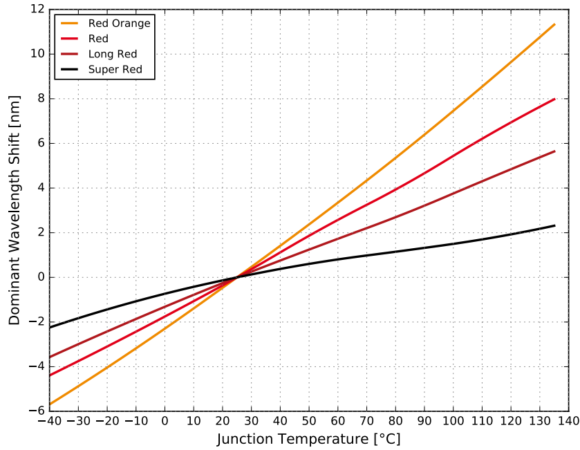
Figure 1b. Typical dominant wavelength shift vs junction temperature for SignalSure 75 at 20 ms MP, 75 mA, T_j = 25^\circ\text{C}
