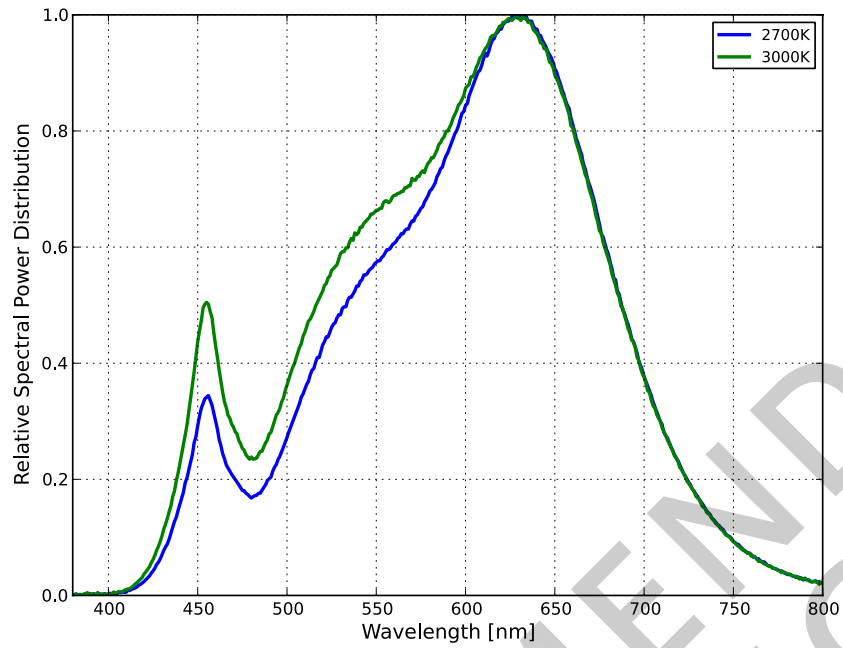
Figure 1c. Typical normalized power vs. wavelength for L1T2-xx90000000000 at 700mA, T_j=85^\circ\text{C} .
